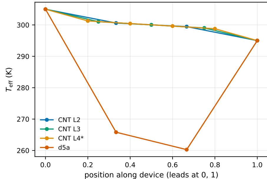
Local effective temperature (eq:Teff_local)
