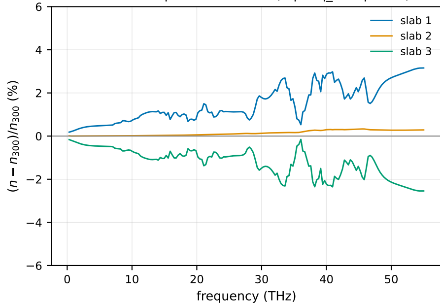
CNT L3 occupation deviation (eq:neq_occupation)
