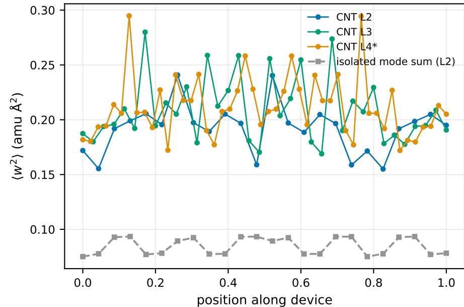
CNT mean-square displacement
