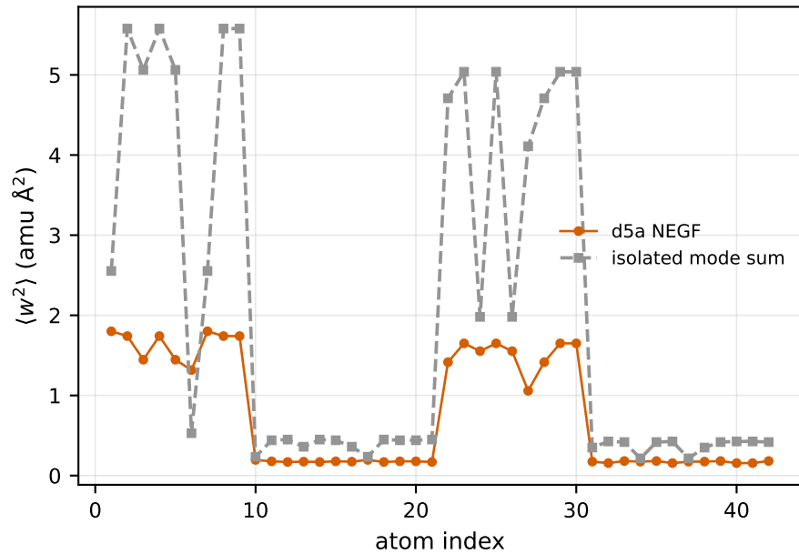
d5a mean-square displacement
