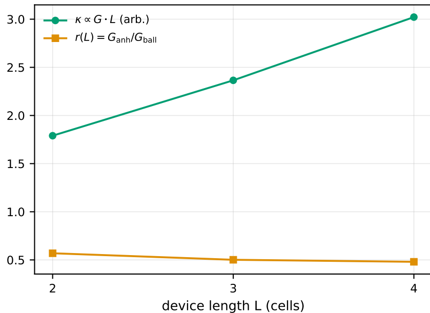
Length scaling
