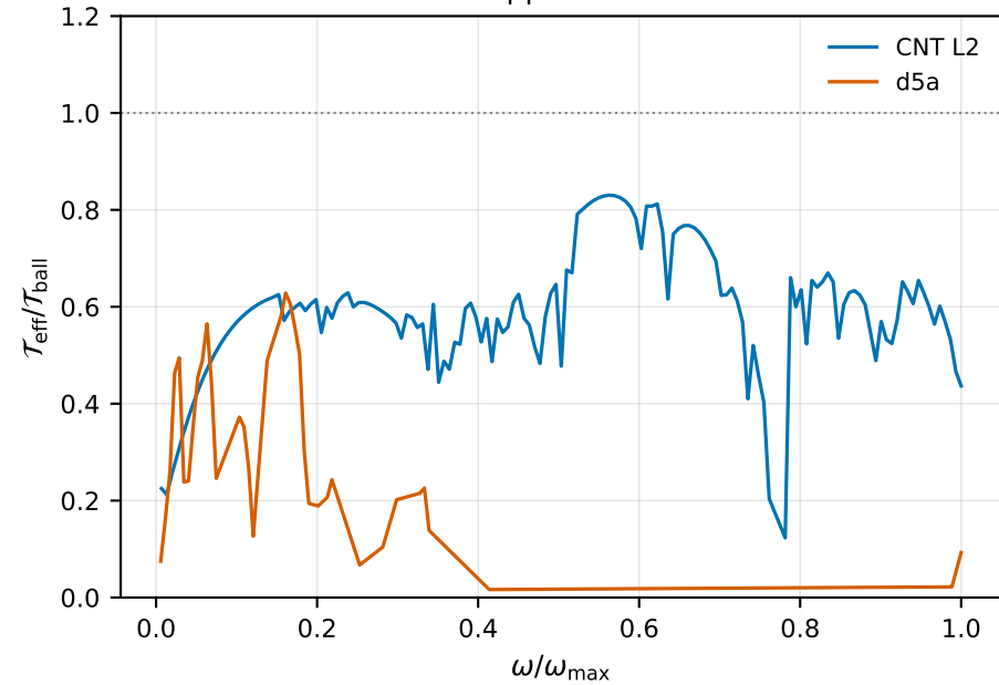
Anharmonic suppression: CNT vs d5a
