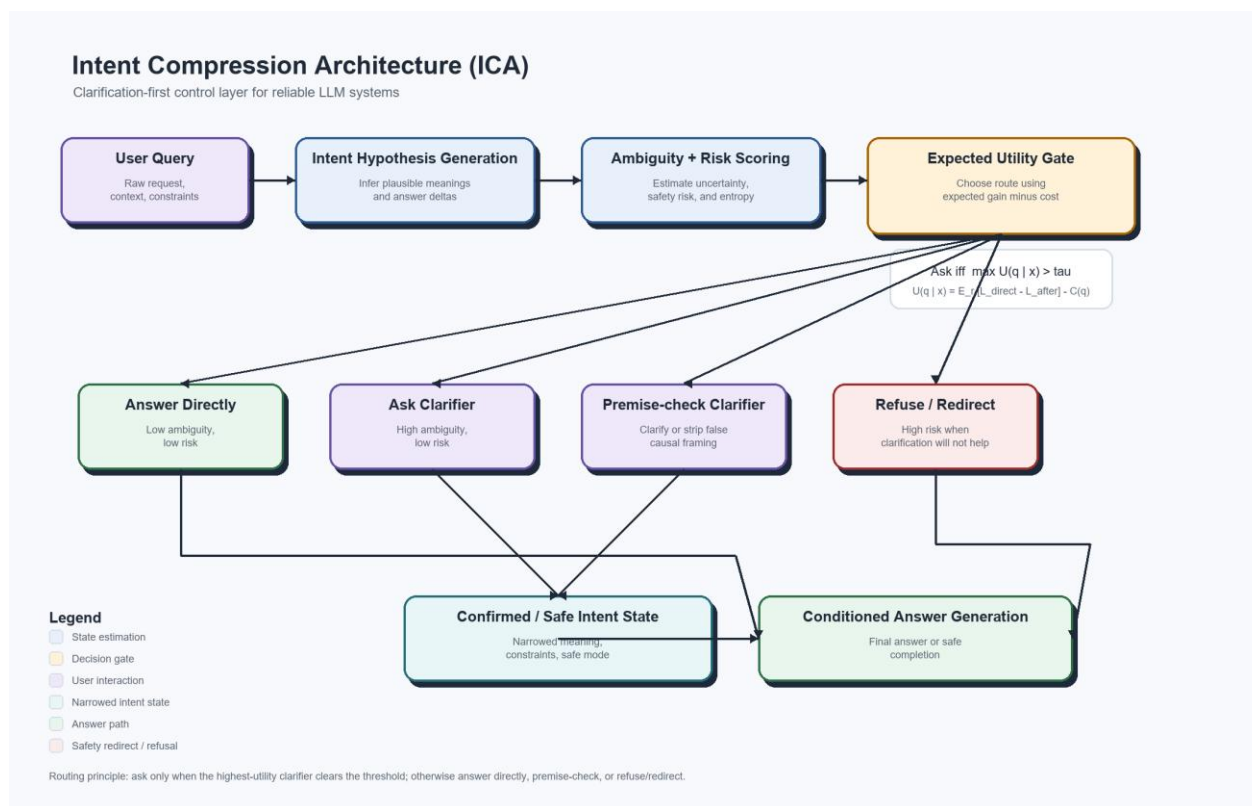
Figure 1. ICA control flow with expected-utility routing and embedded legend.
