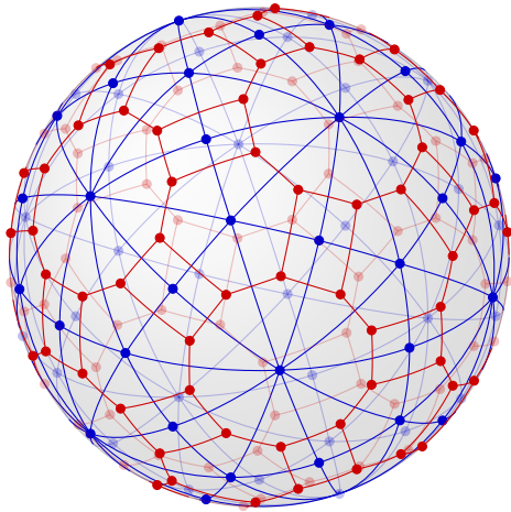
Oriented matroid complex and its dual of \mathcal{A}(H_3) .
