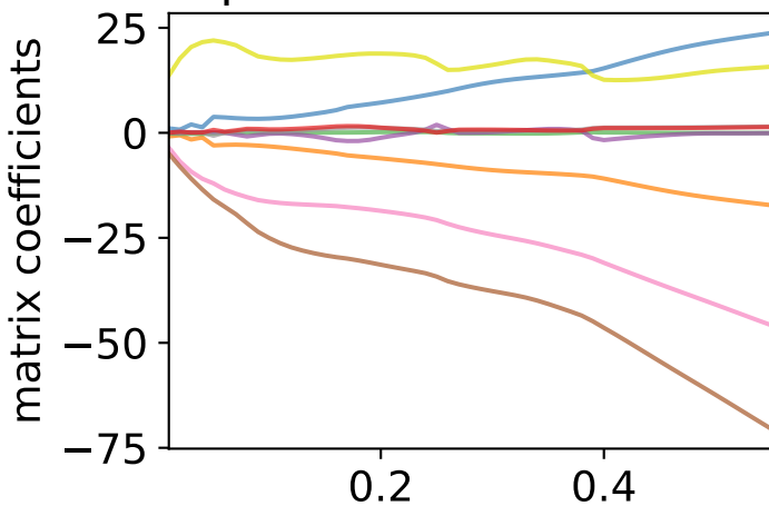
Optimal \mathbf{A} to forecast z
