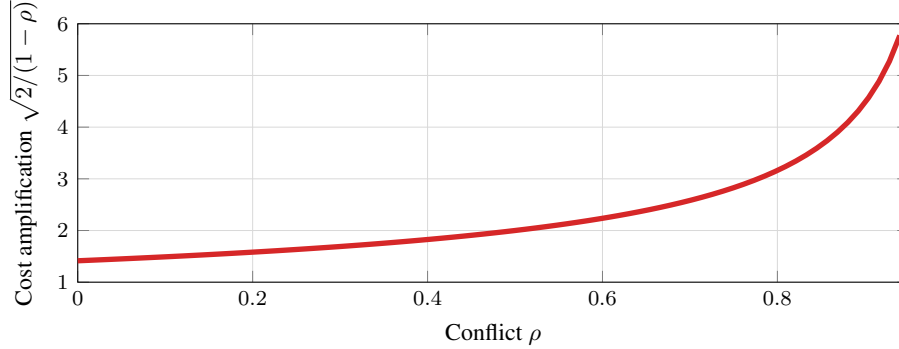
Figure A1: Cost Amplification. Meta-theorem [Operating Envelope]: escape is not. The diagonal cost factor \sqrt{2/(1-\rho)} (Corollary 3.5) diverges as conflict \rho \rightarrow 1 . At \rho = 0 (orthogonal), cost is \sqrt{2} \approx 1.41 . At \rho = 0.5 , cost doubles. At \rho = 0.9 , cost exceeds 4\times .
