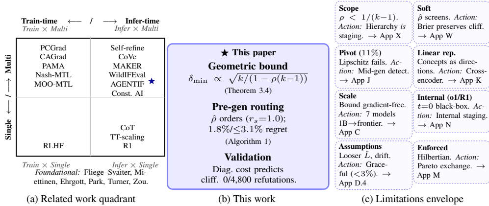
Figure 7: Where this work sits and where it stops. (a) Related work quadrant: existing methods cluster in single-constraint inference and multi-constraint training; multi-constraint inference (upper right) lacked a geometric foundation. (b) This paper: geometric bound (Theorem 3.4) and pre-generation routing (Algorithm 1). (c) Limitations envelope: each card names a boundary and the system’s action there (deferral, mid-generation detection, hierarchy/staging, graceful degradation). Operationally : bounded honesty about observability is what makes pre-generation routing fail-safe. All citations in (a) hyperlink to App Z; all cards in (c) hyperlink to their appendix discussions.
