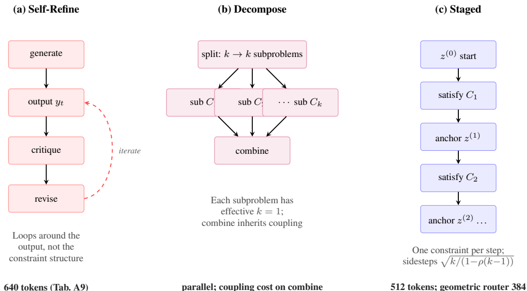
Self-Refine addresses capability variance ; Staged addresses constraint structure ; Decompose reduces effective k .
