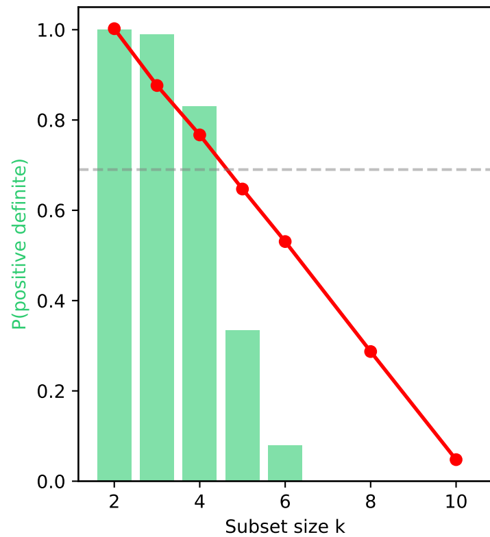
k-Subset Phase Transition (real constitution rho)
