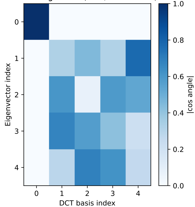
DCT Alignment (k=5, rho=0.267)
