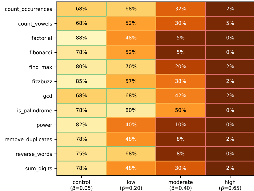
Per-Task Pass Rate by Tier (11/12 monotone)
