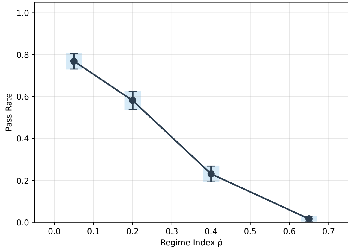
Aggregate Pass Rate with 95% Bootstrap CI r_s = -0.942 (48 pts), p = 2.12e-23
