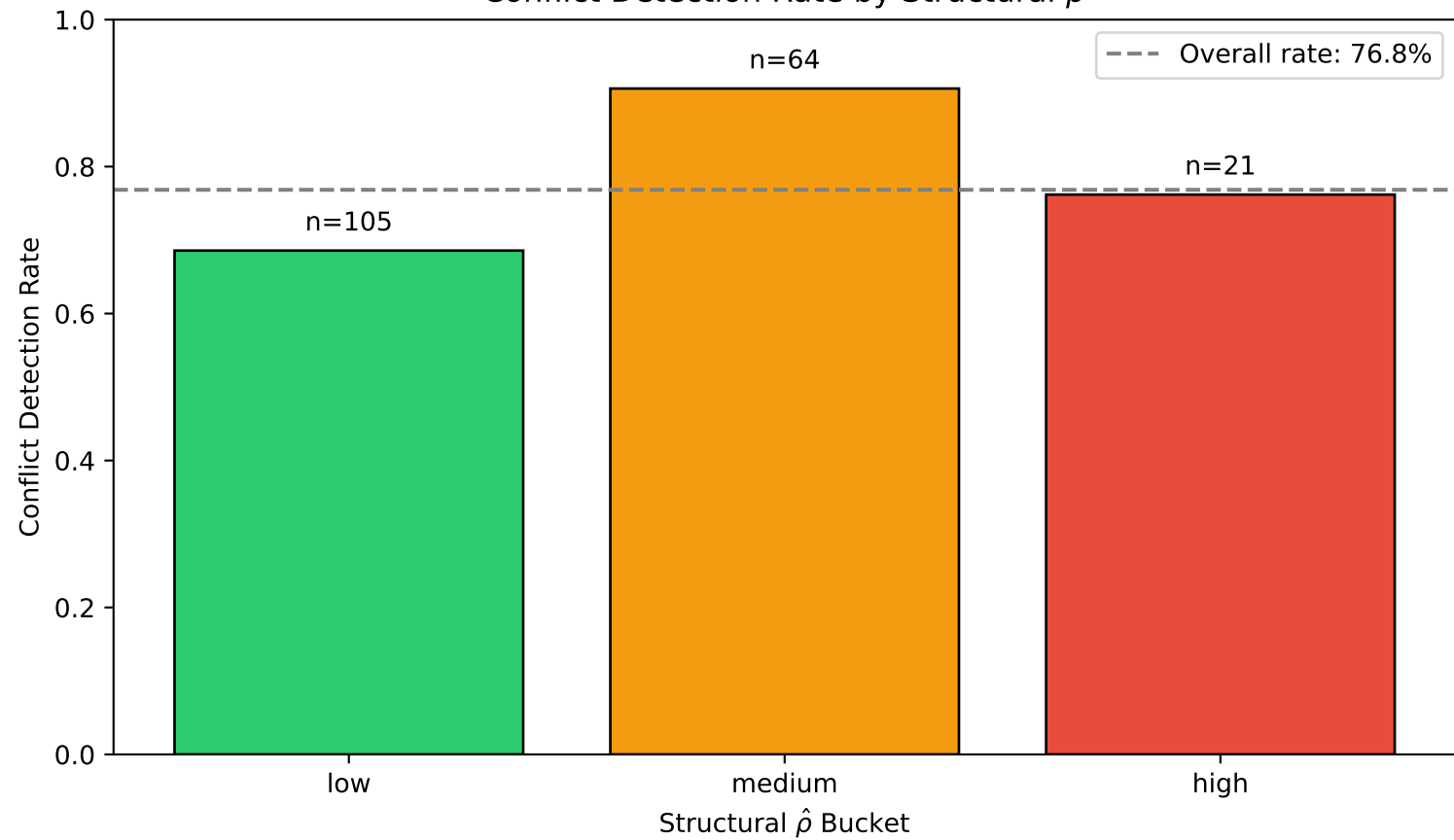
Conflict Detection Rate by Structural \hat{\rho}
