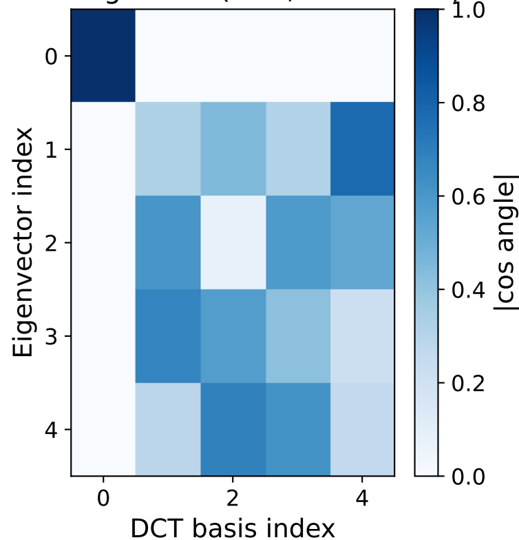
DCT Alignment (k=5, rho=0.267)
