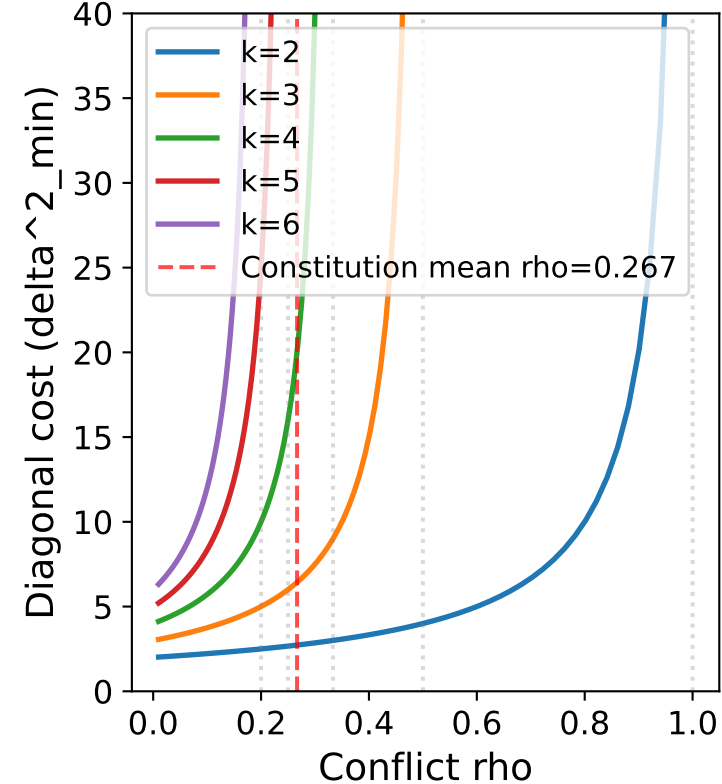
Phase Transition + Real rho
