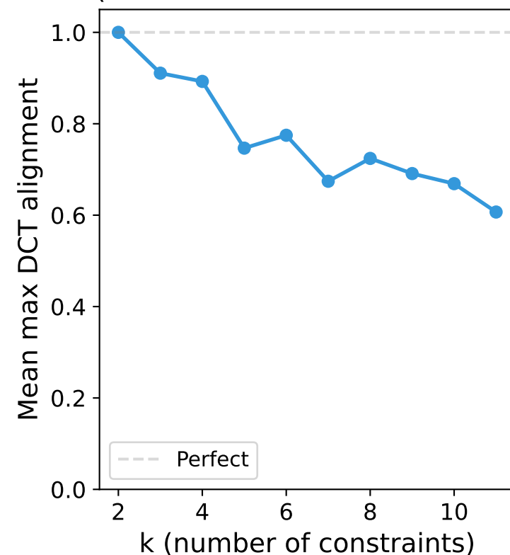
DCT Alignment vs k (rho=0.267 from constitution)
