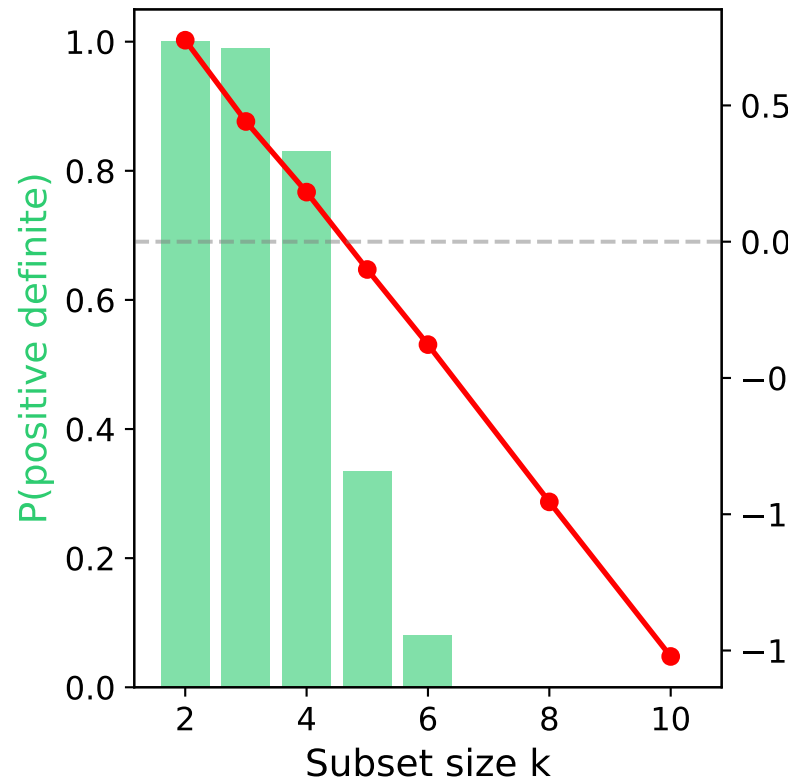
k-Subset Phase Transition (real constitution rho)
