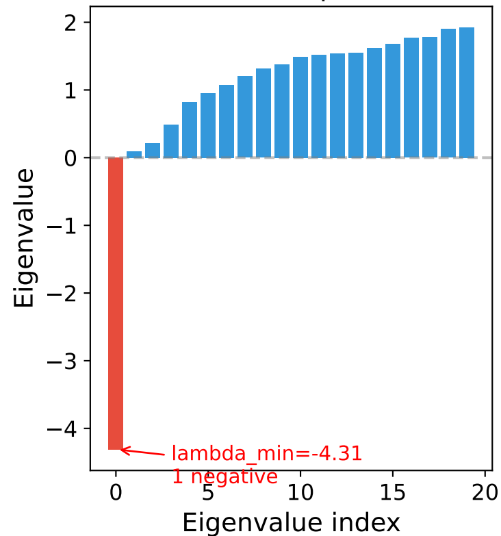
Constitution Gram Spectrum (n=20)
