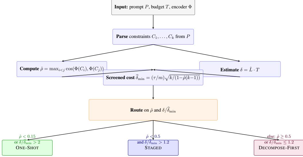
Figure A4: Algorithm 1 as a decision tree (schematic). The screening statistic \hat{\rho} and budget ratio \delta/\hat{\delta}_{\min} are computed from the prompt before generation, then composed at a single routing junction with three terminal regimes. The conditions printed beside each terminal are exactly those in lines 6–12 of Algorithm 1. Provenance: ci/illustration_lineage.json; draft via gpt-5.4-image-2; final asset is hand-authored TikZ. Schematic illustration only; not empirical evidence.
