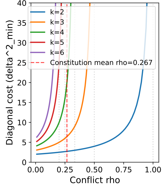
Phase Transition + Real rho
