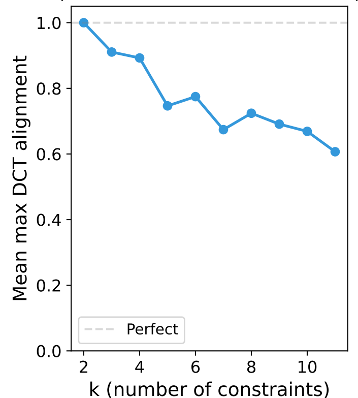
DCT Alignment vs k (rho=0.267 from constitution)
