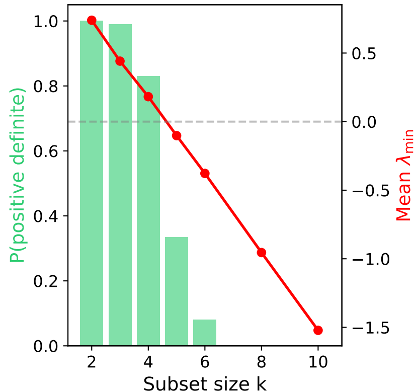
k-Subset Phase Transition (real constitution rho)
