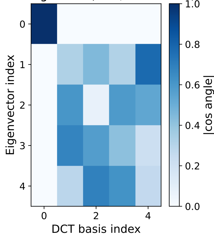
DCT Alignment (k=5, rho=0.267)
