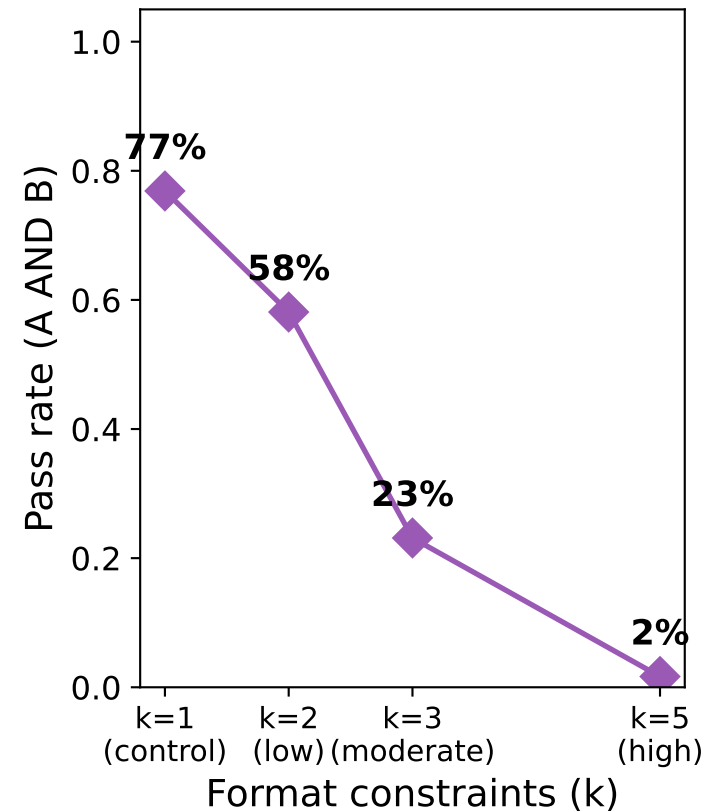
Empirical Cliff (4 models, 1920 trials)
