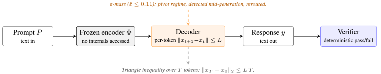
Figure A2: Interface Assumption (schematic): text-in / text-out, frozen encoder, deterministic verifier. The Lipschitz bound \|x_{t+1} - x_t\| \leq L on per-token displacement is the contract; integrating over T tokens gives \|x_T - x_0\| \leq LT . The \varepsilon -mass (11%) is the pivot regime detected mid-generation and rerouted (Appendix J). Provenance for this illustration: ci/illustration_lineage.json ; the certificate fails if the source assumption text drifts.
