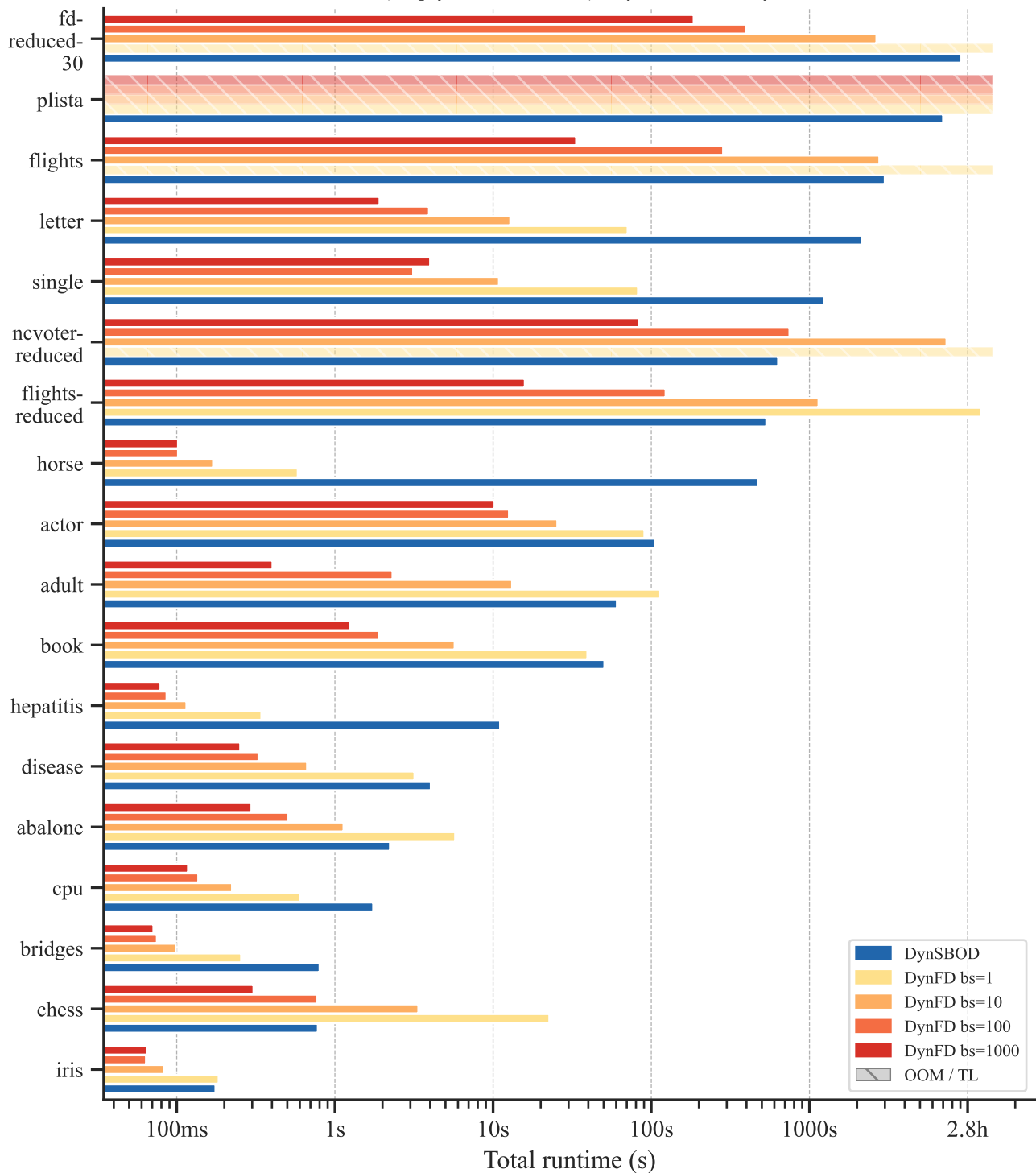
Insert (empty → full dataset): DynSBOD vs DynFD
