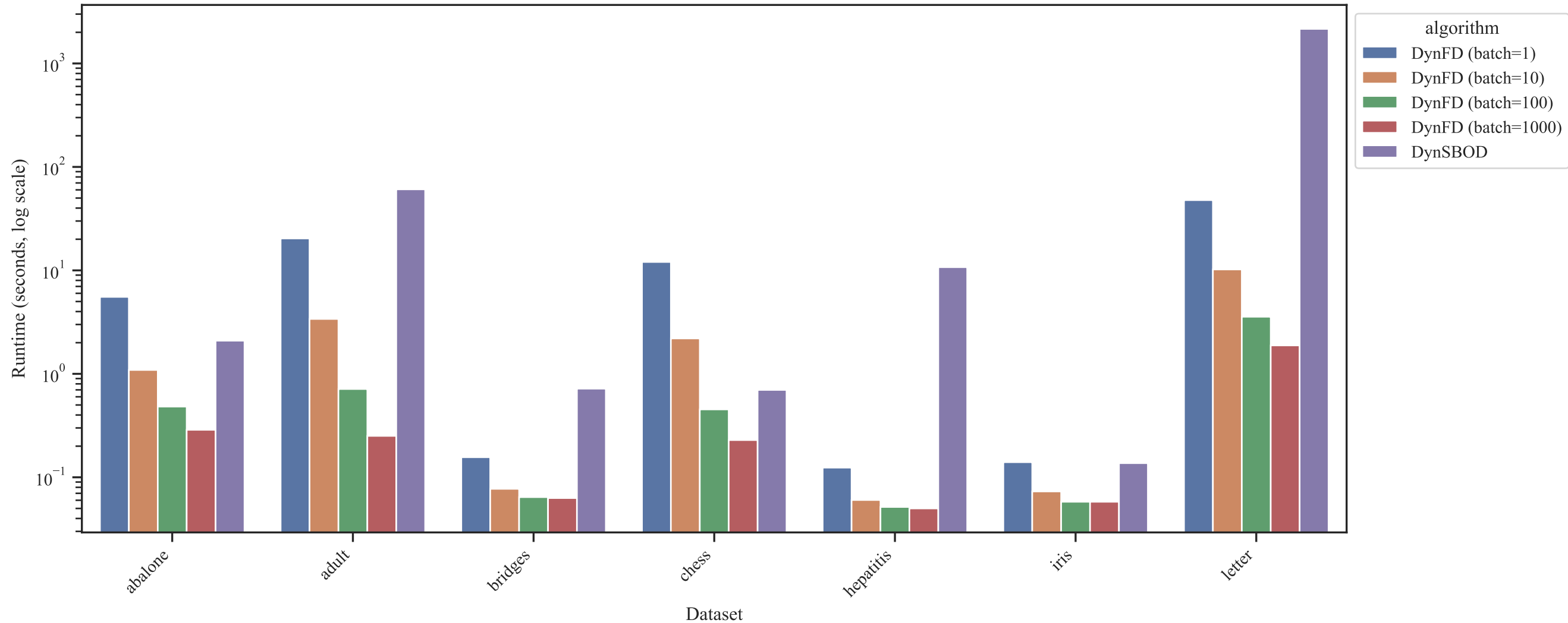
DynFD (different batch sizes) vs DynSBOD Runtime Comparison
