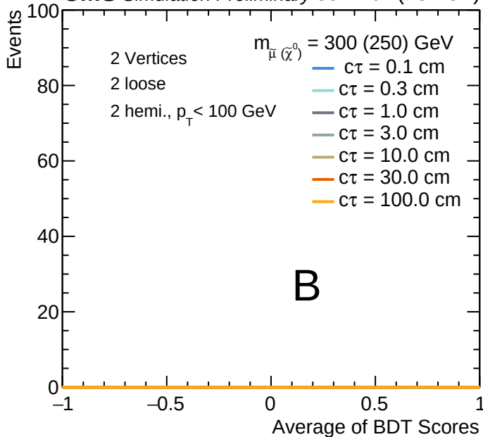
CMS Simulation Preliminary 59.7 fb -1 (13 TeV)
