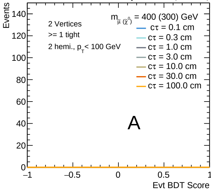
CMS Simulation Preliminary 59.7 fb -1 (13 TeV)
