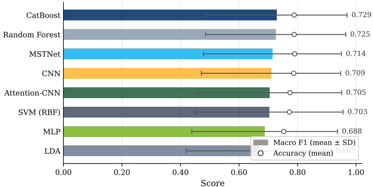
Leave-One-Session-Out Cross-Validation
