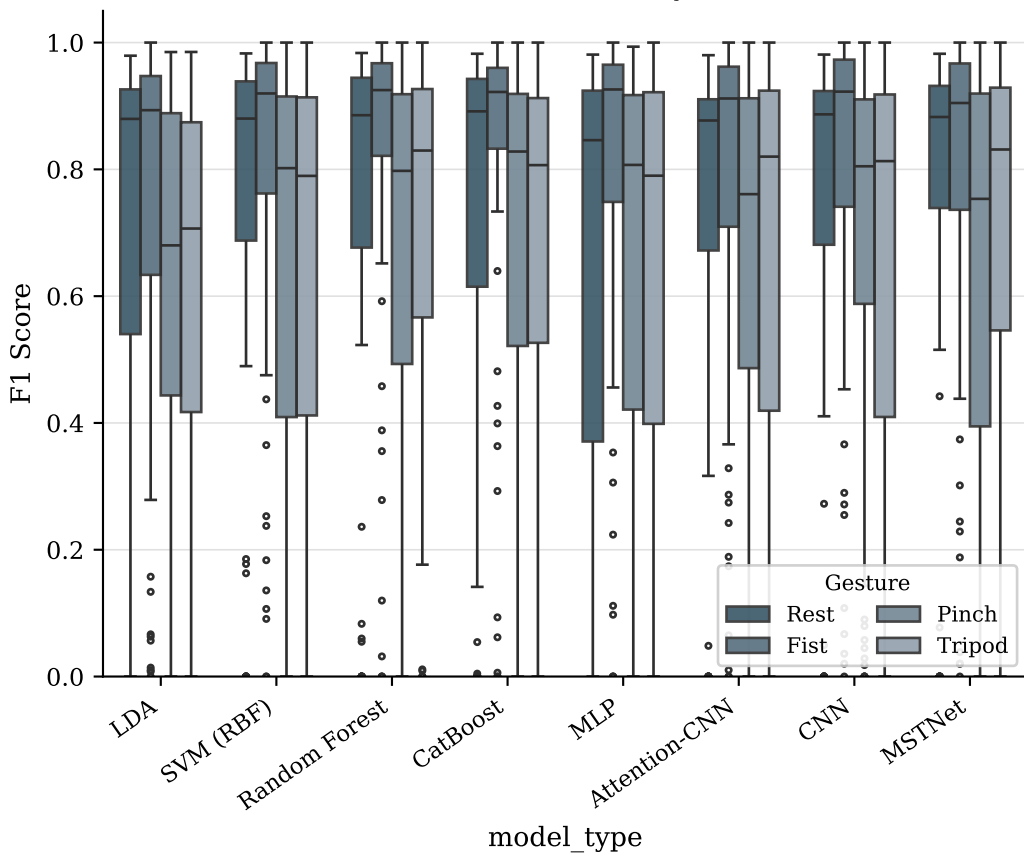
Per-Class F1 Distribution by Classifier
