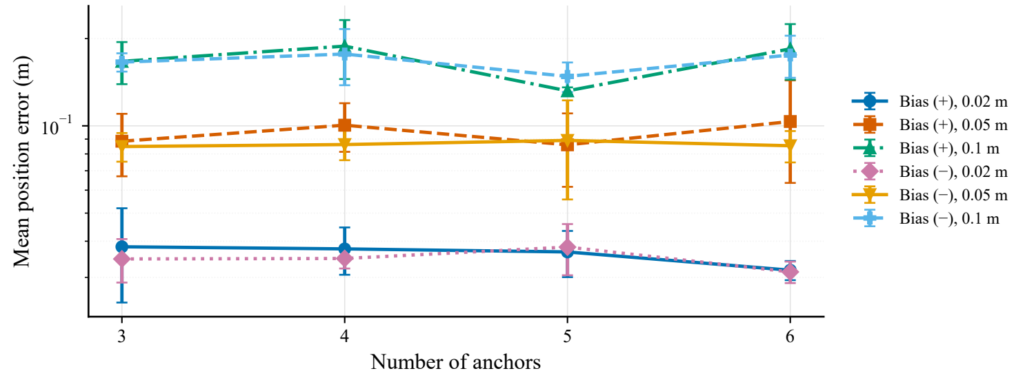
Effect of distance bias on positioning error
