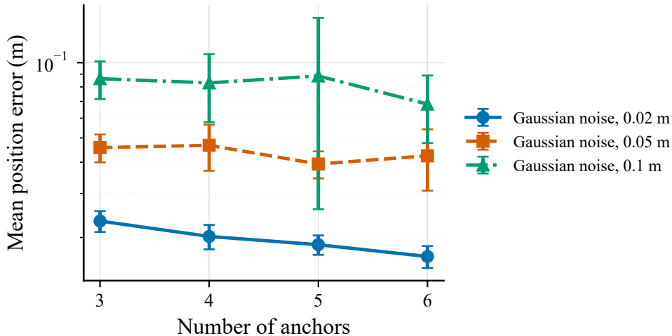
Effect of Gaussian distance noise on positioning error
