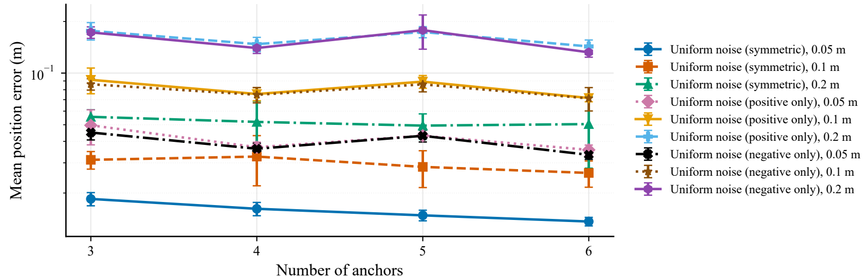
Effect of uniform distance noise on positioning error
