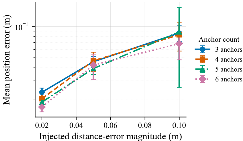
Error vs. Gaussian noise \sigma
