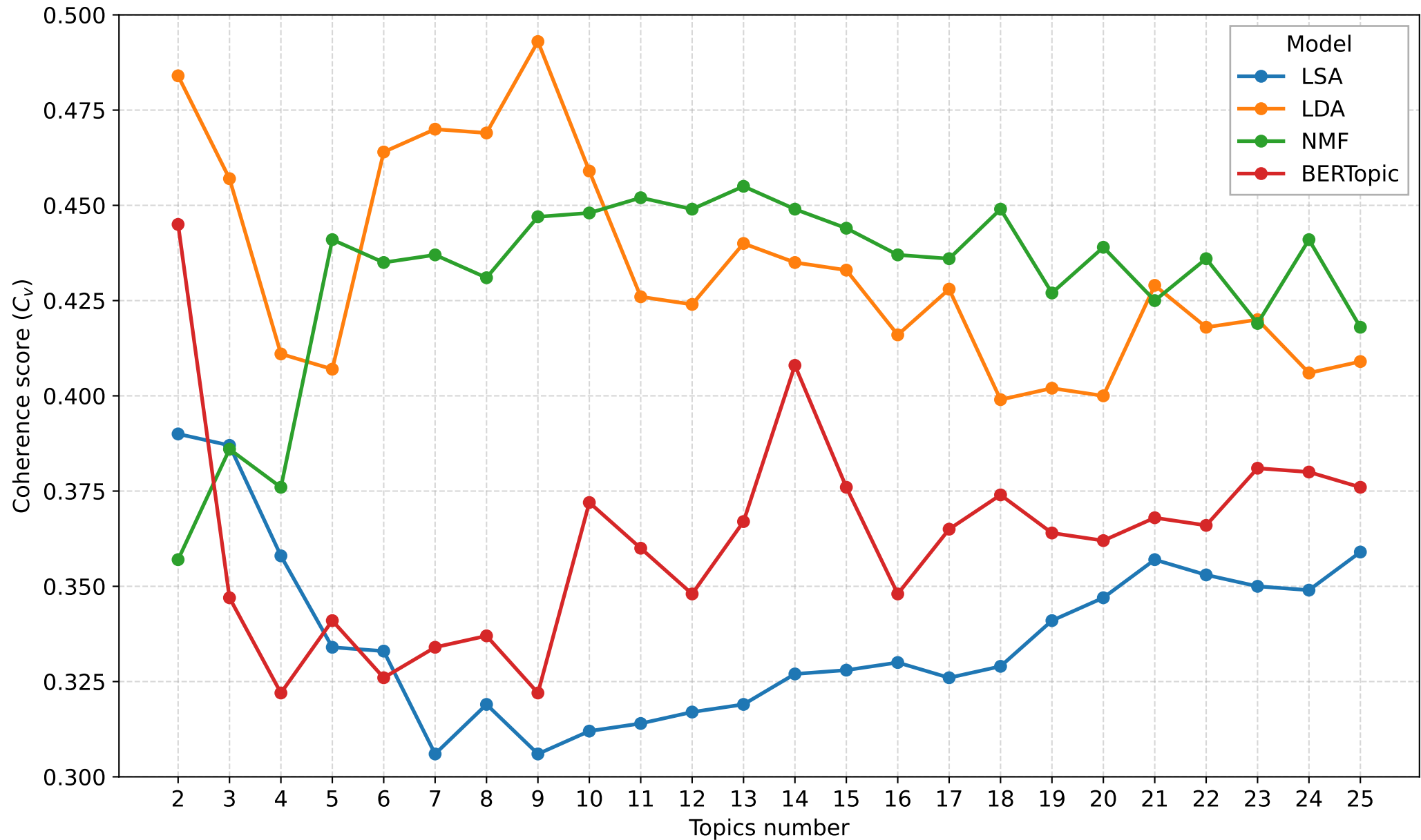
Coherence ( C_v ) score per model and topics number
