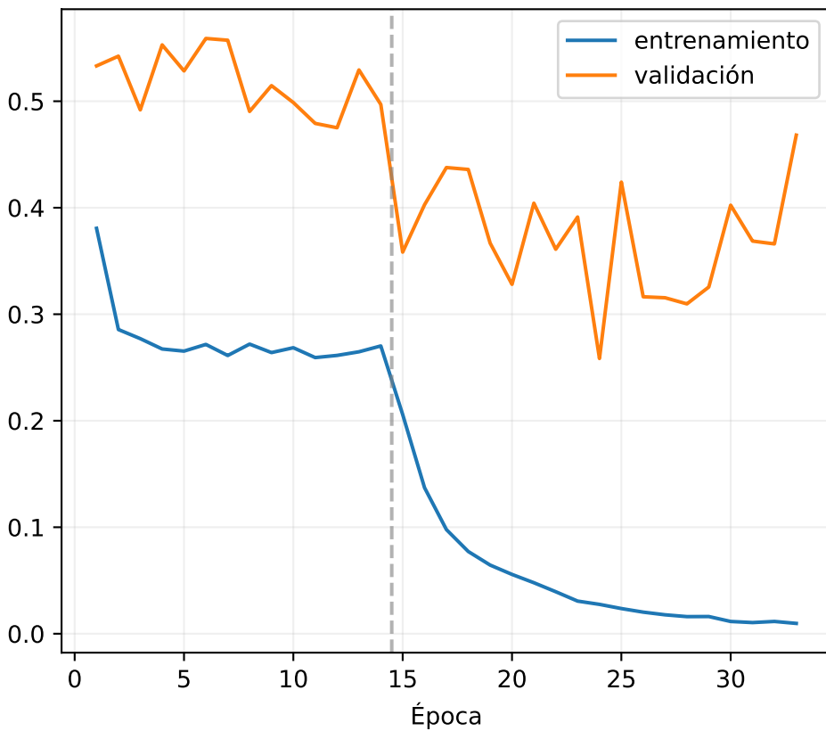
Loss
