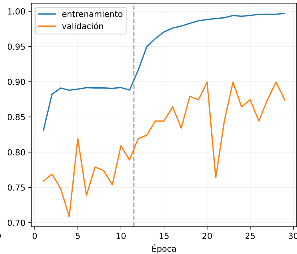
Accuracy
