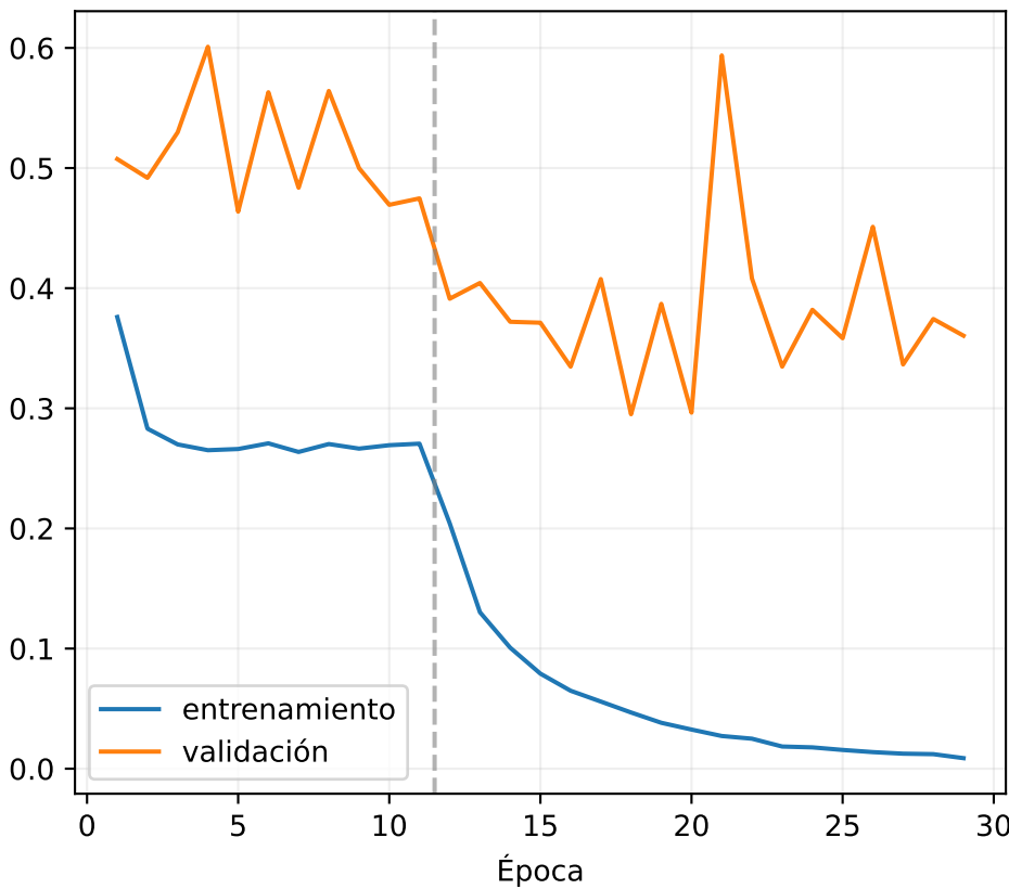
Loss
