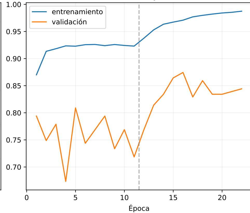
Accuracy
