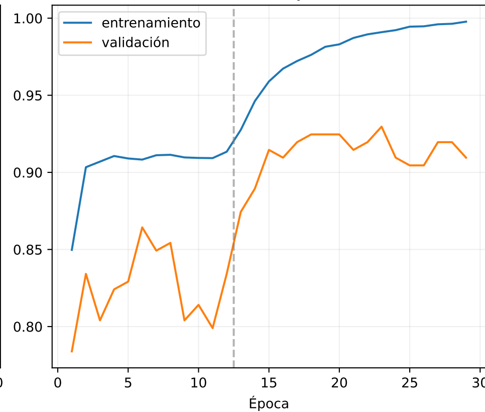
Accuracy
