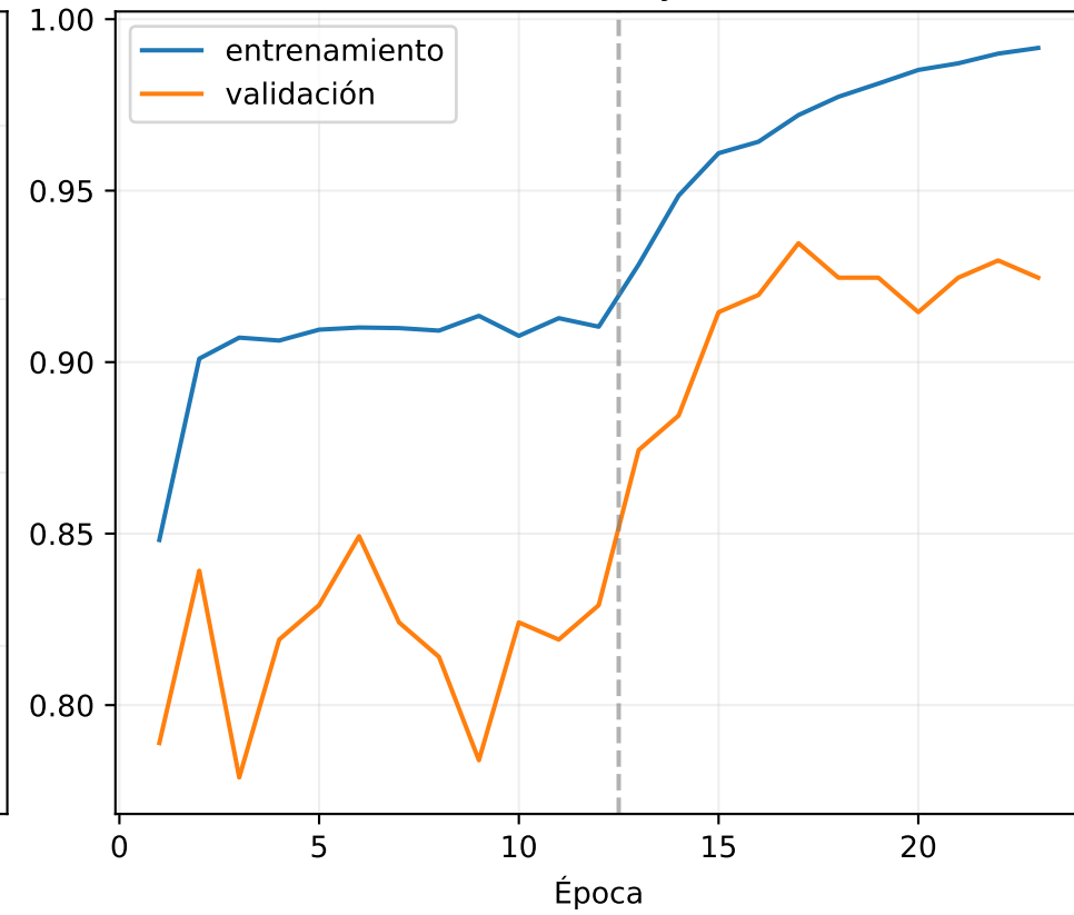
Accuracy
