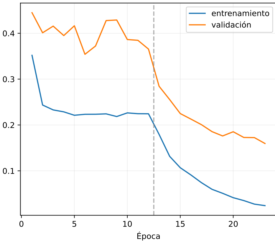
Loss
