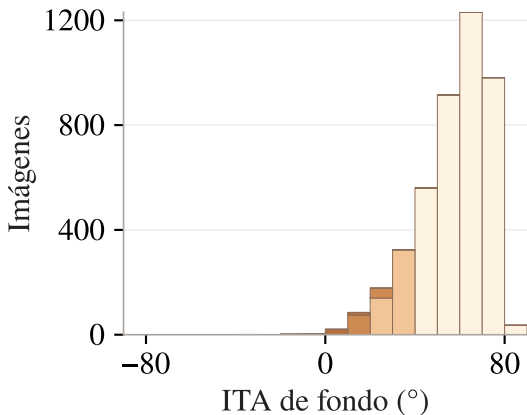
(c) ISIC2020
