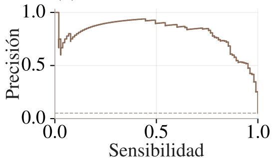
(b) BCC · AP = 0,809
