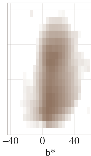
ISIC 2019
