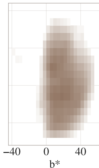
ISIC 2020
