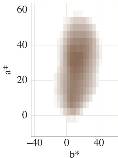
(b) HAM10000
