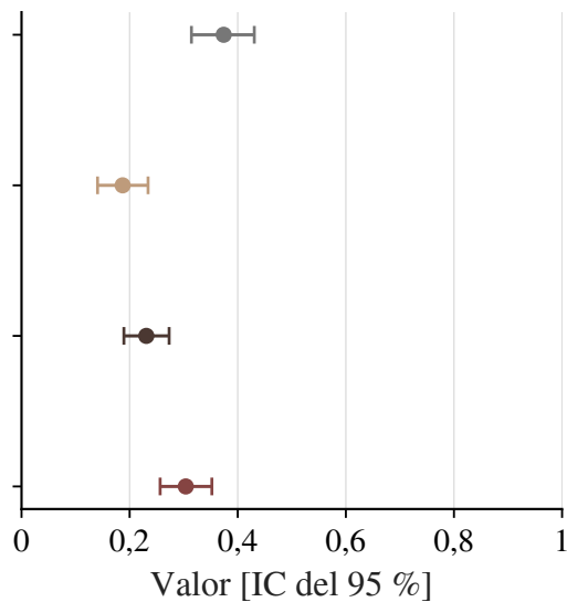
MCC
