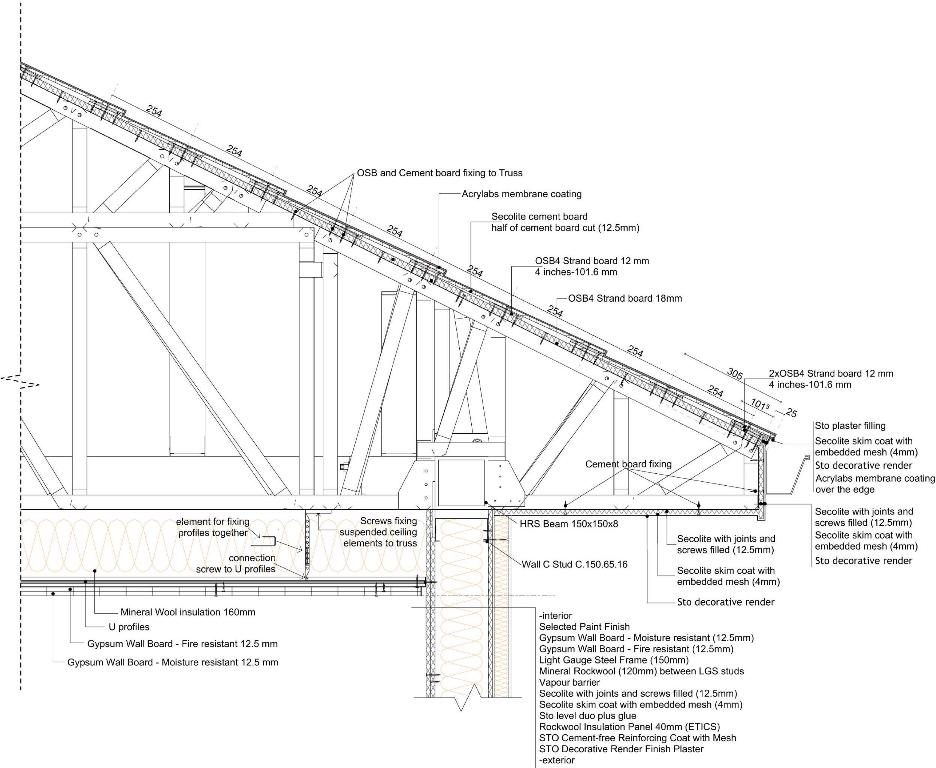
D.Island Style Roof Detail
