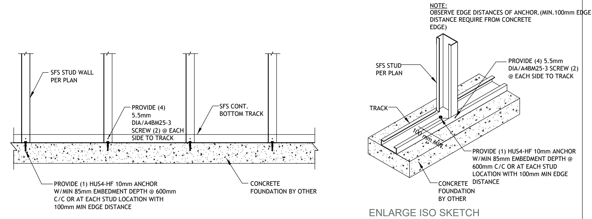
Typical Detail : SFS Bottom Track to Concrete Connection (External Wall)
