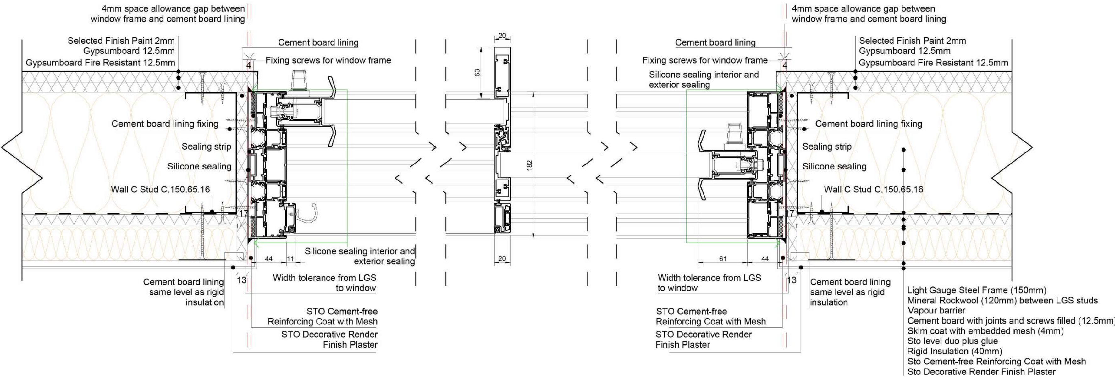
D.Sliding Door/Window Floor Plan with insect screens
