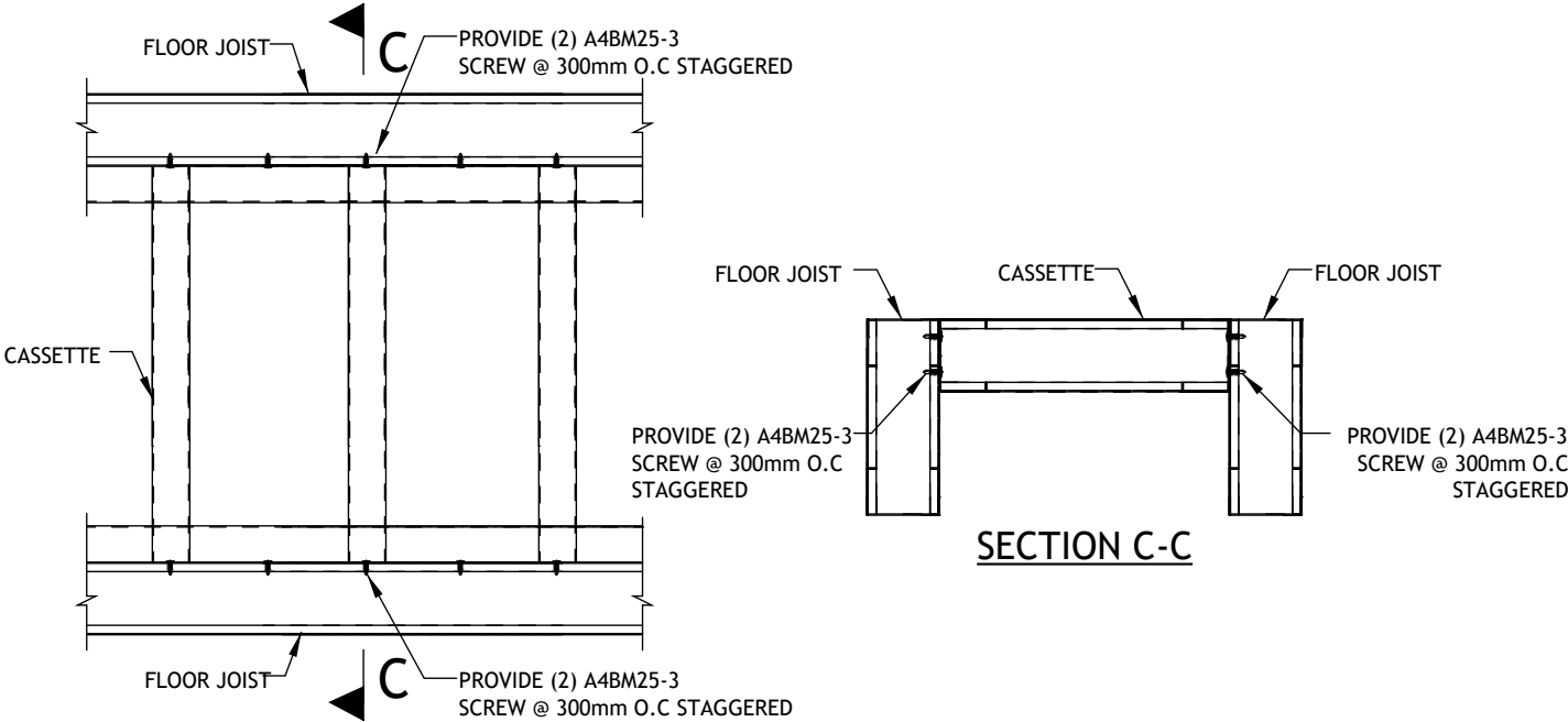
Floor Blocking to Floor Joist Connection
