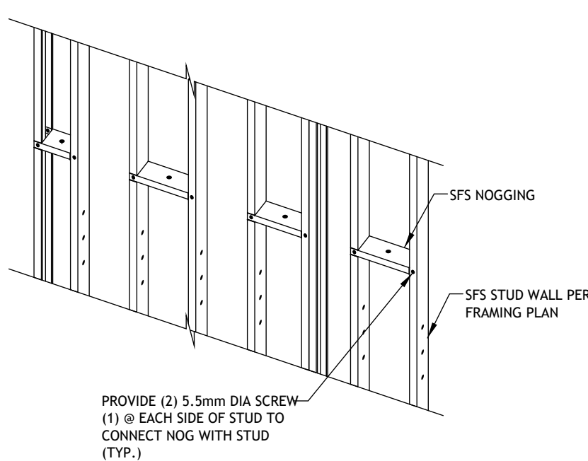
Hit and Miss Nogging to Stud Connection Detail
