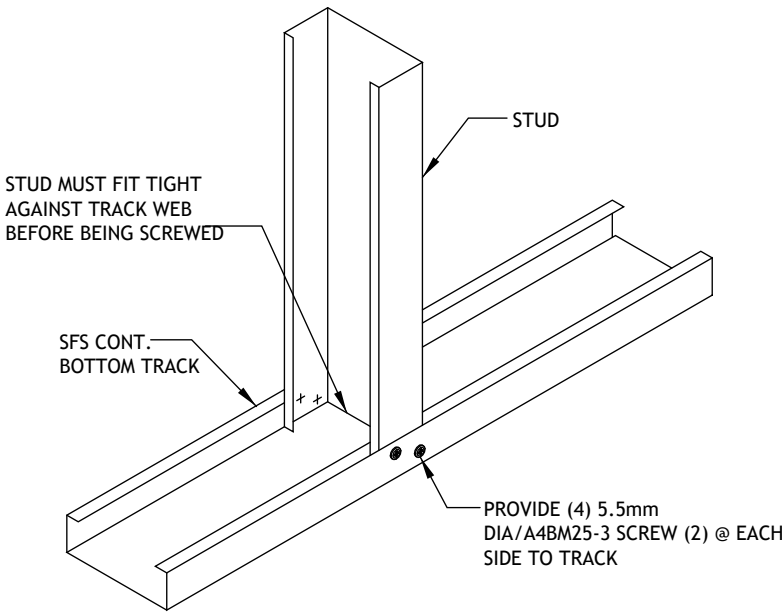
Stud to Bottom Track Connection (External Wall)
