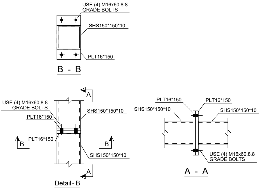
Typ. Vertical Splice Connection
