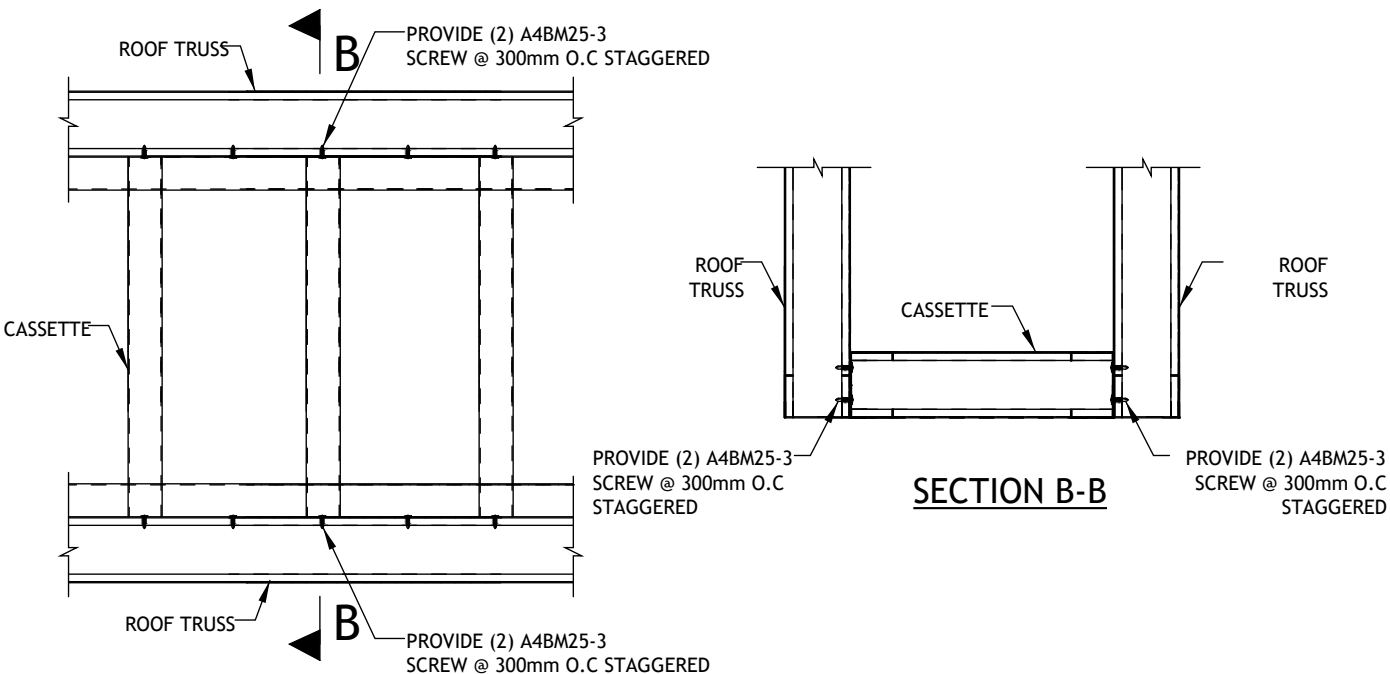
Cassette to Roof Truss Connection
