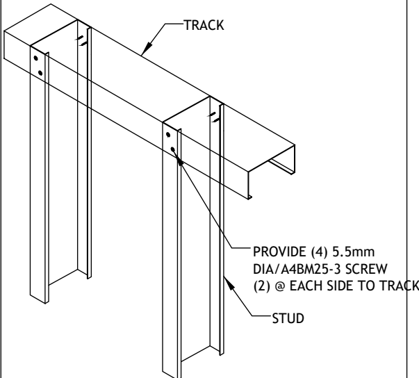
Stud to Top Track Connection (External Wall)
