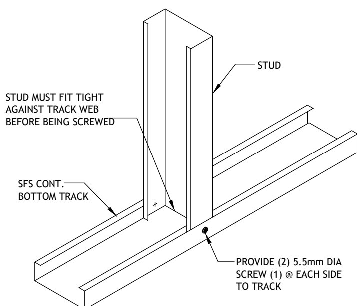
Stud to Bottom Track Connection (Internal Wall)
