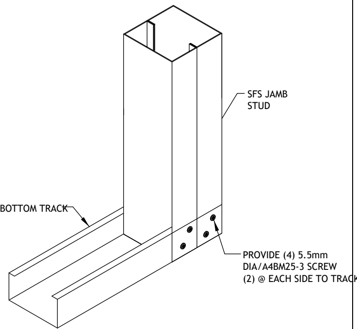
Box Jamb to Bottom Track Connection
