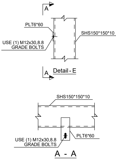
Typ. Wall to Beam Top Plate Connection
