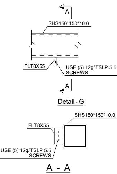
Cassette to Beam Connection
