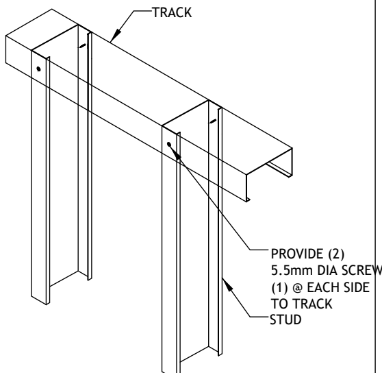
Stud to Top Track Connection (Internal Wall)
