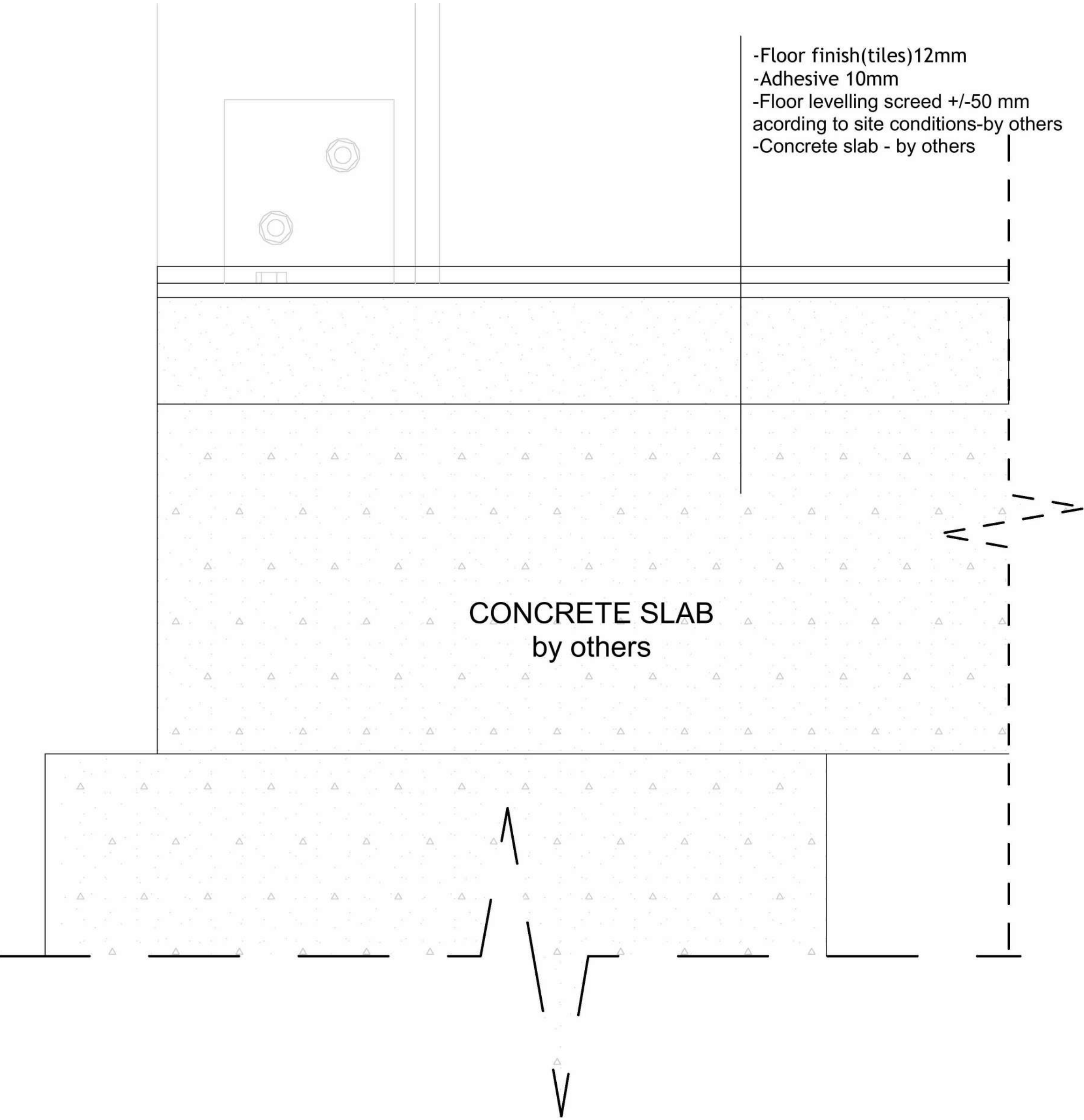
D11.Exterior terrace base Detail
