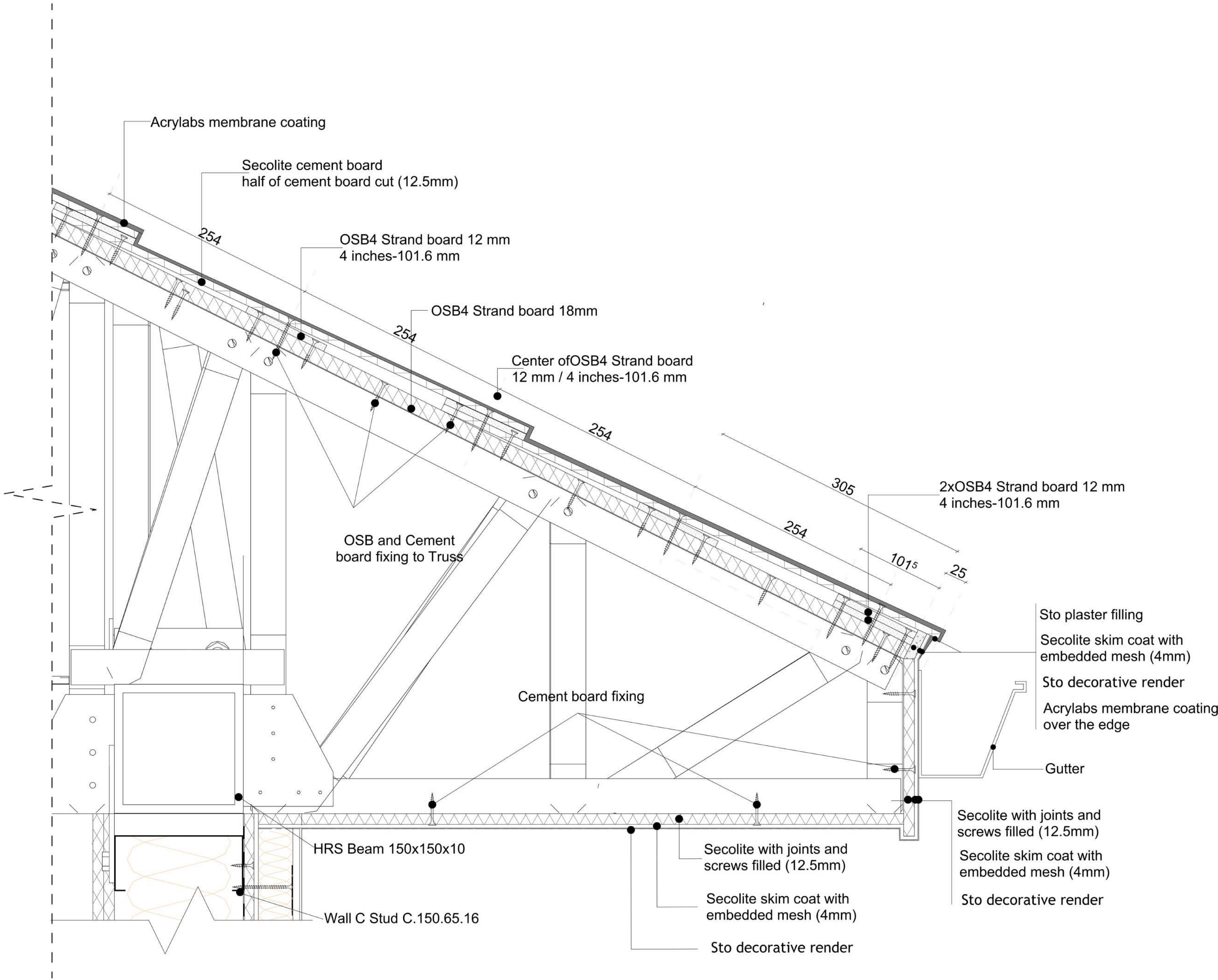
D.Island Style Roof Detail
