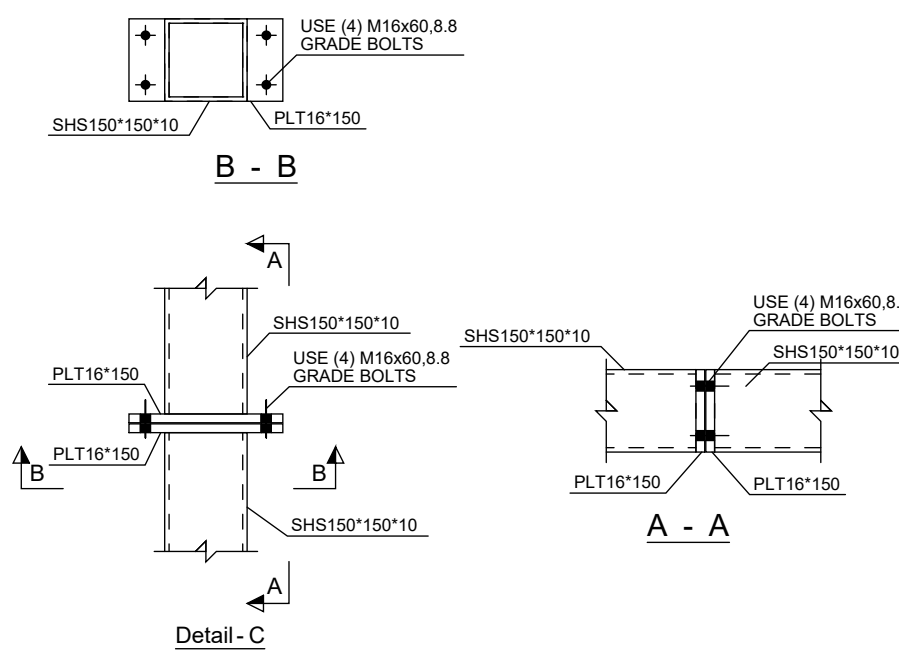
Typ. Horizontal Splice Connection
