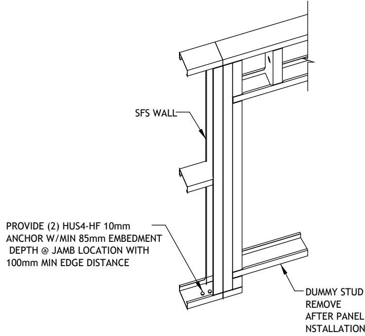
Typical Detail for Two Anchor at Jamb Location
