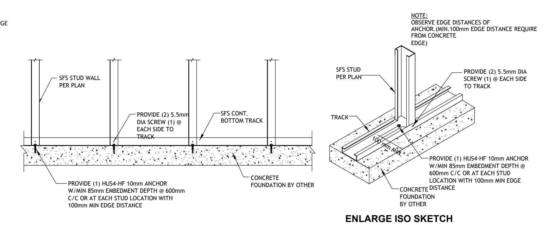
Typical Detail : Bottom Track to Concrete Connection (Internal Wall)
