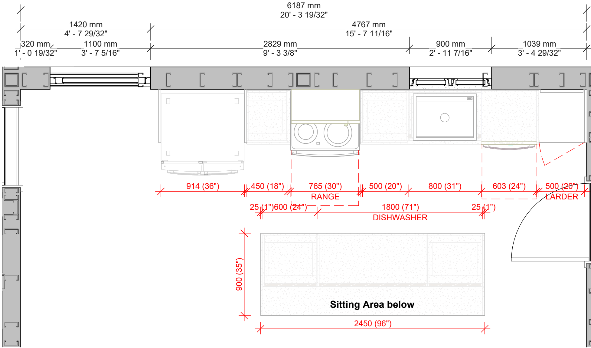
Kitchen Plan
