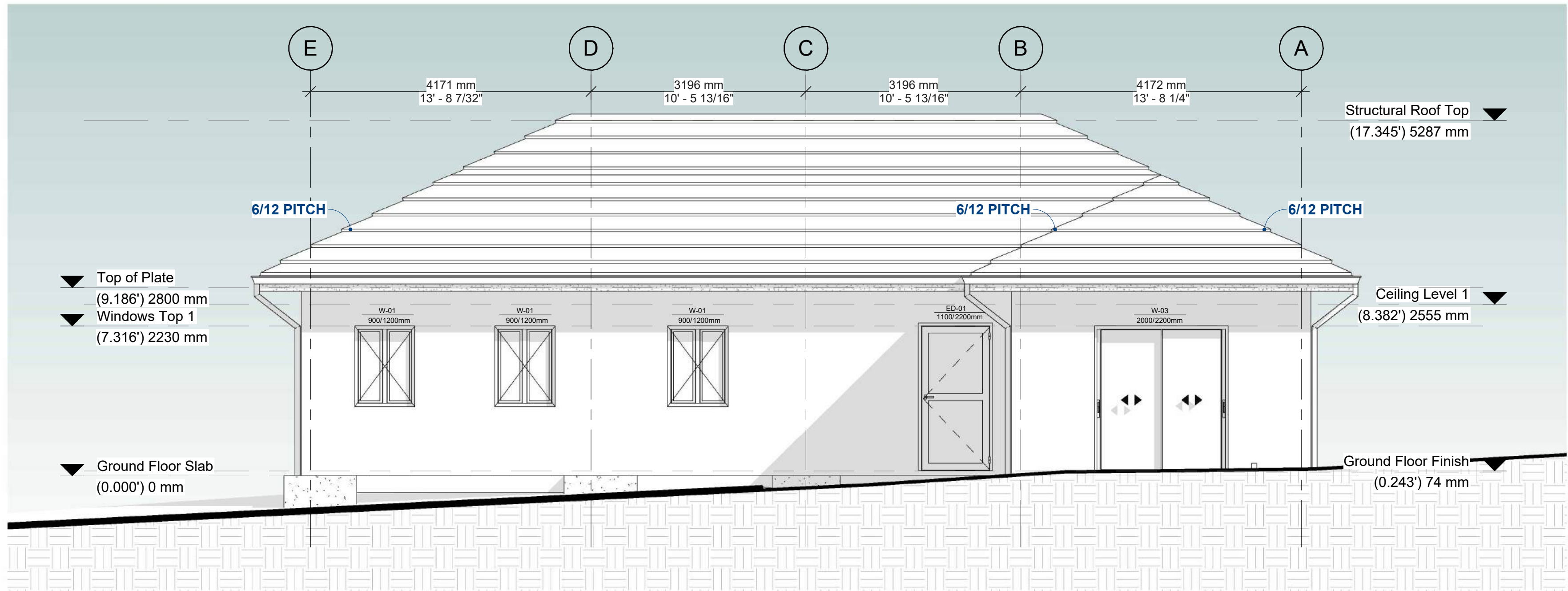
Rear Elevation
