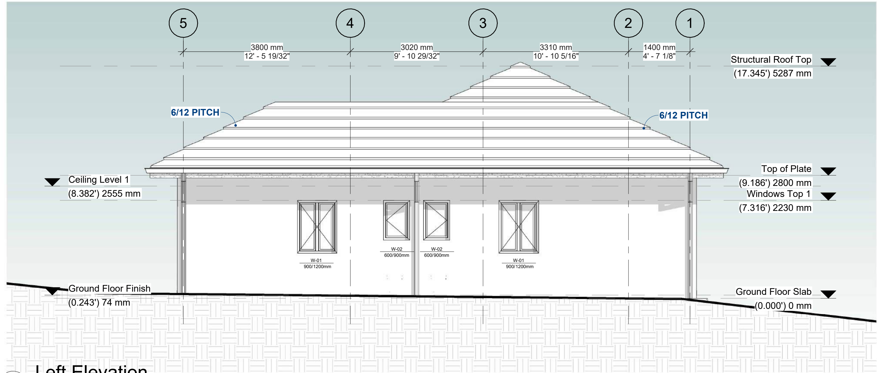
1 Left Elevation 1 : 50
