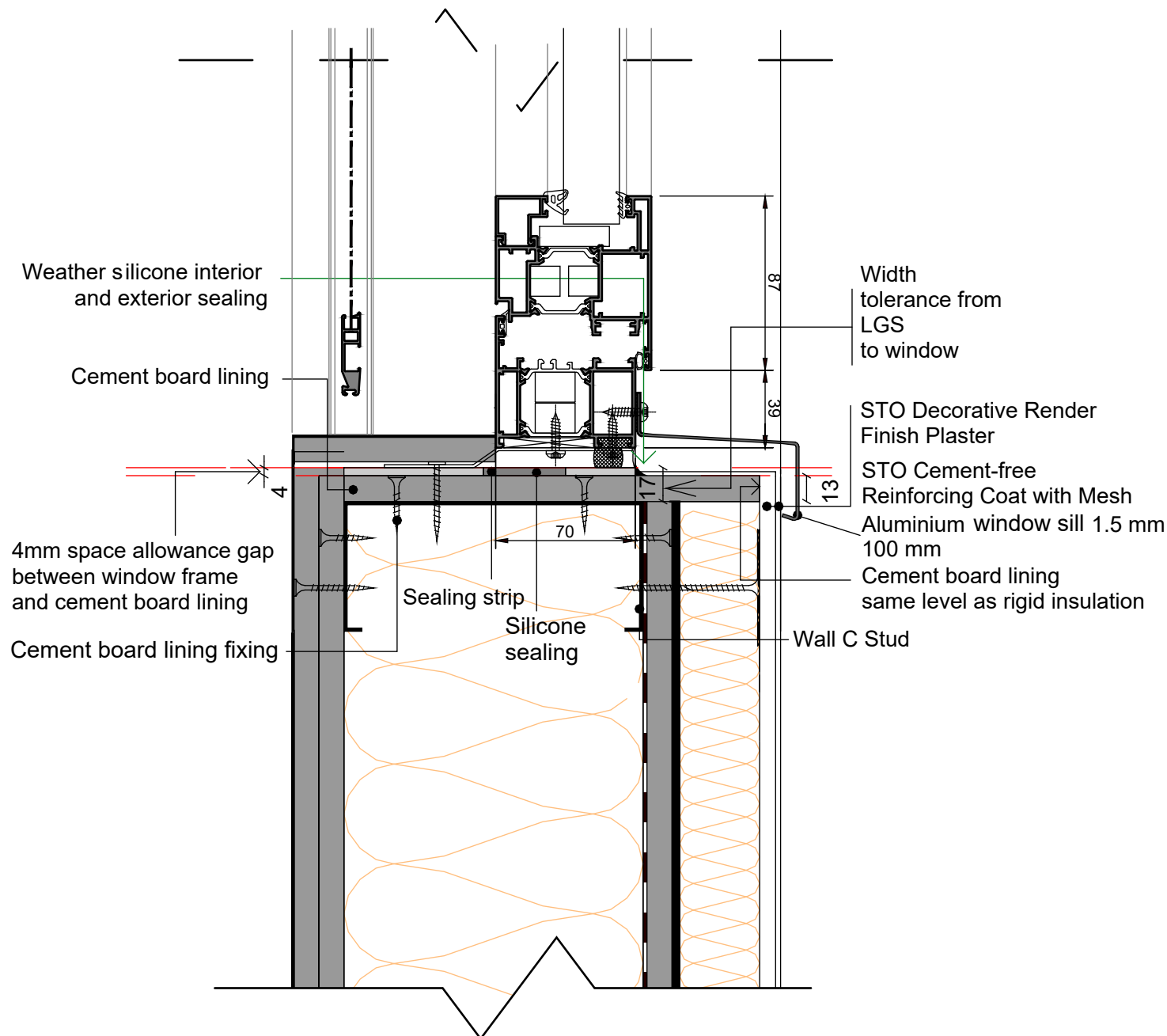
Section Detail: Slider Window with insect screens
