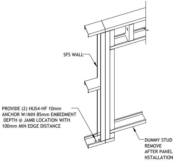
Typical Detail for Two Anchor at Jamb Location
