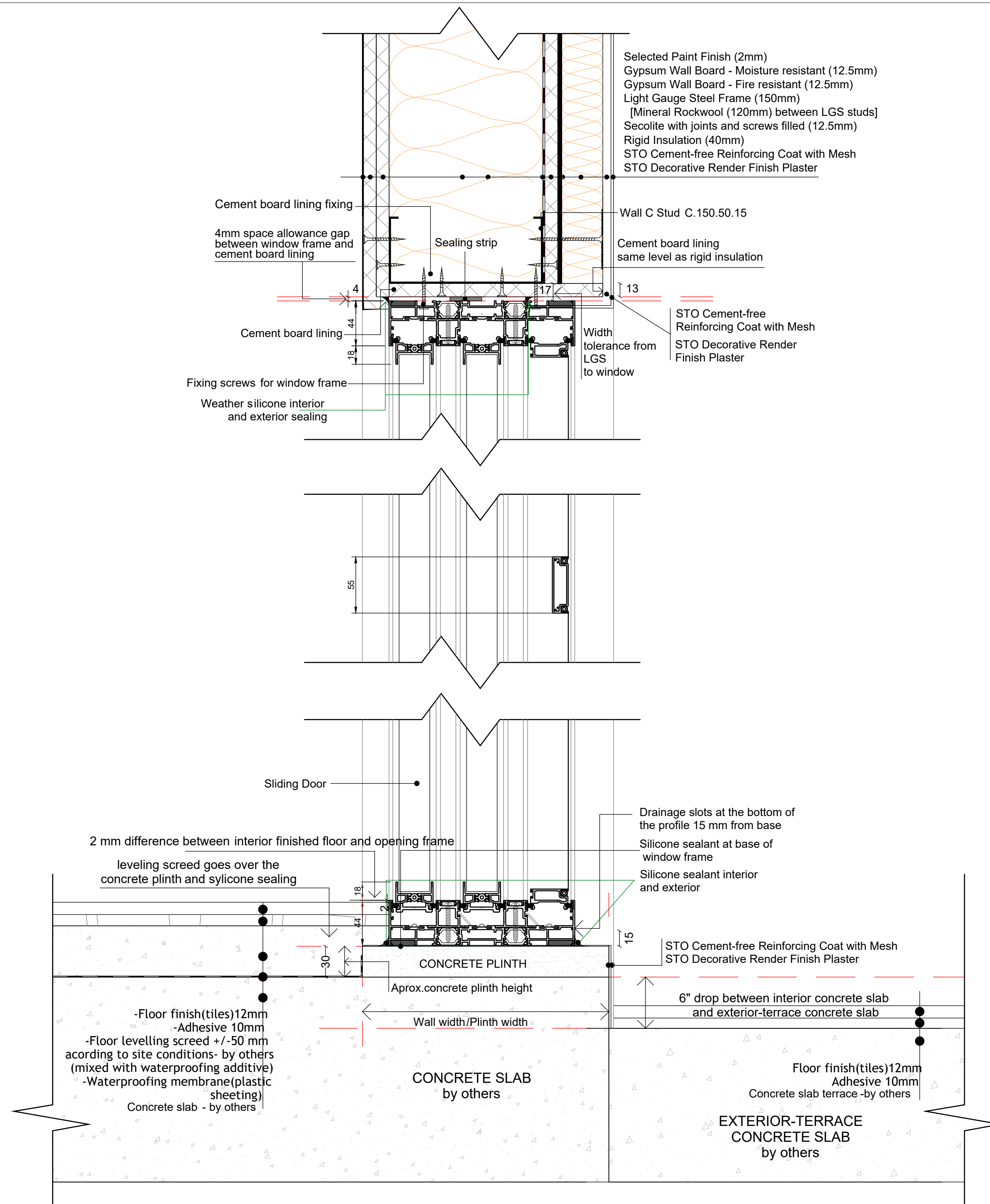
Section Detail: Slider door base fixing detail (with insect screen)
