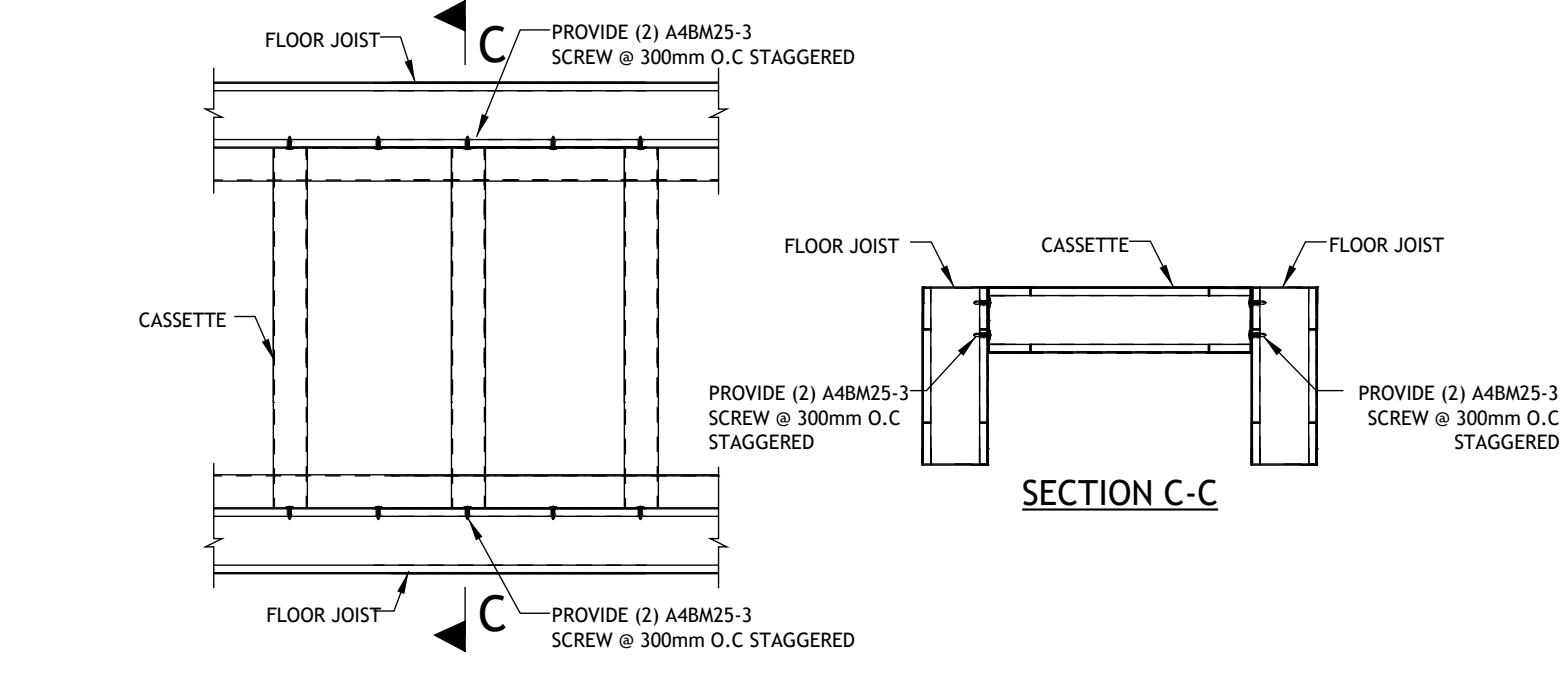
Cassette to Floor Joist Connection
