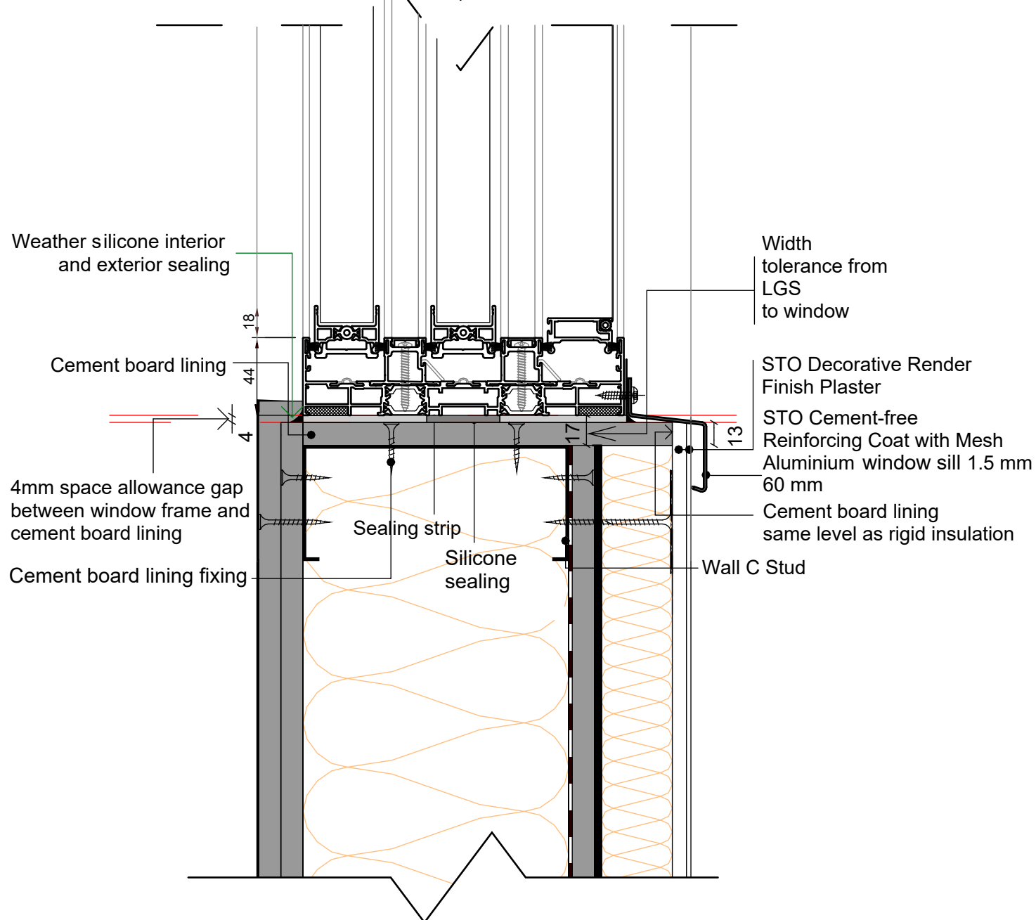
Section Detail: Casement Window with insect screens
