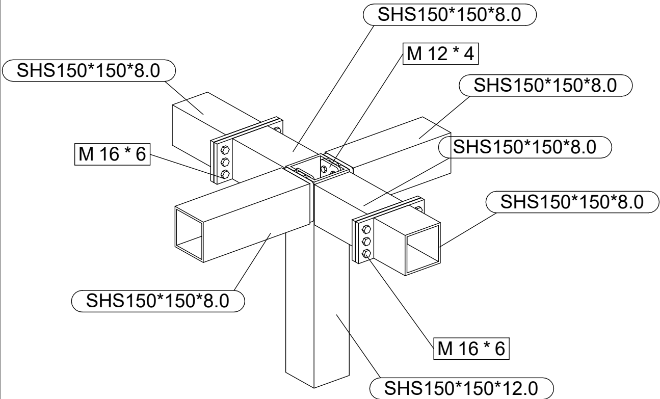
Typical Roof Column Beam Connection
