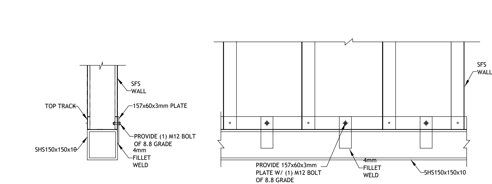
Cassette to Roof Truss Connection
