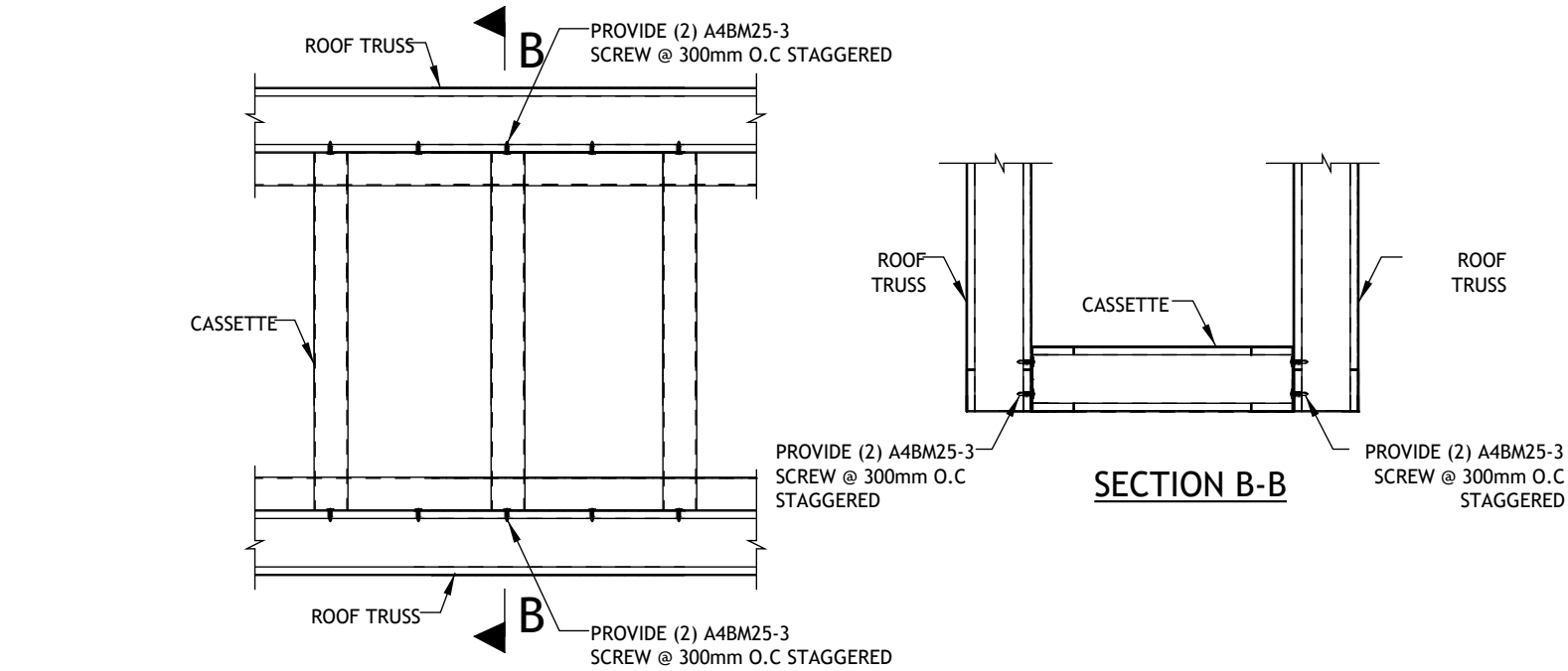
Cassette to Roof Truss Connection
