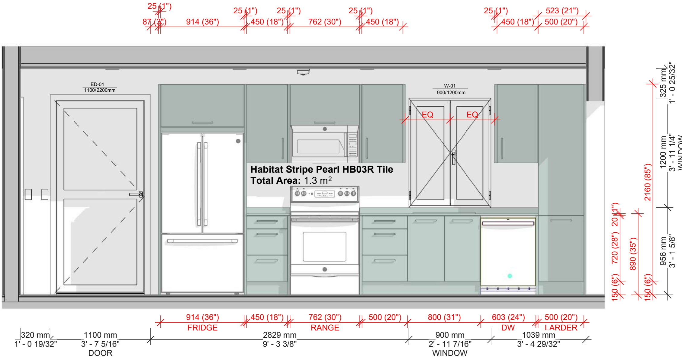
K3 Section
