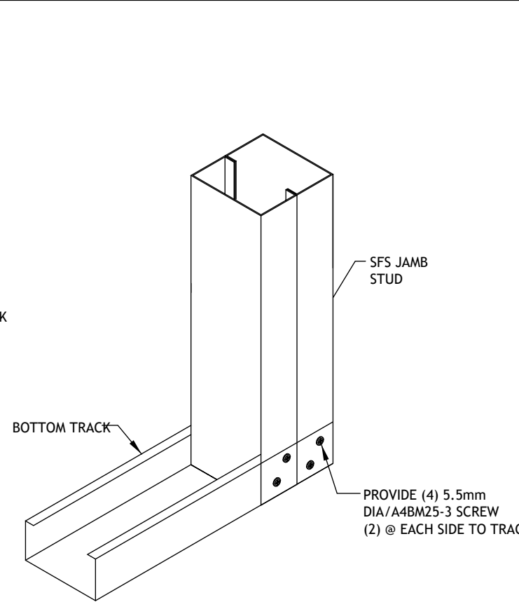
Box Jamb to Bottom Track Connection
