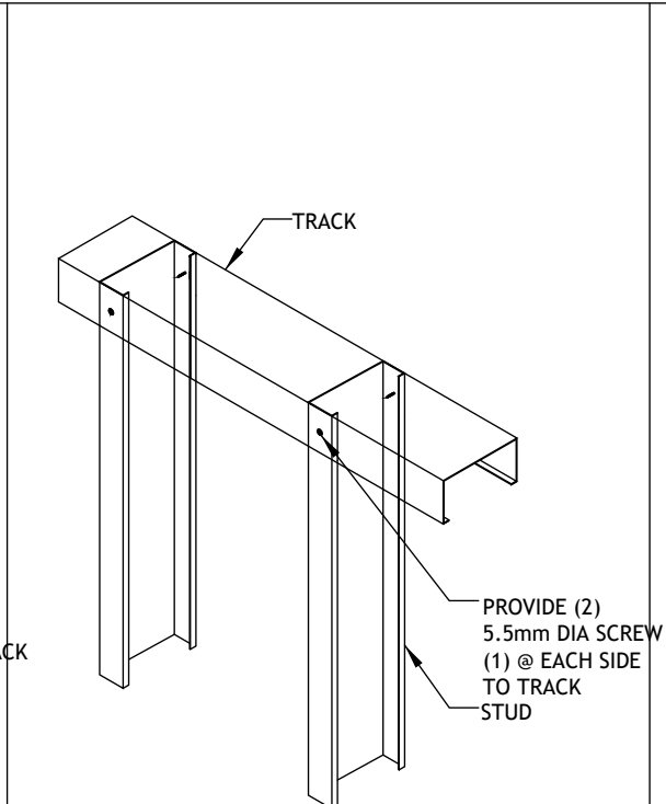
Stud to Top Track Connection (Internal Wall)
