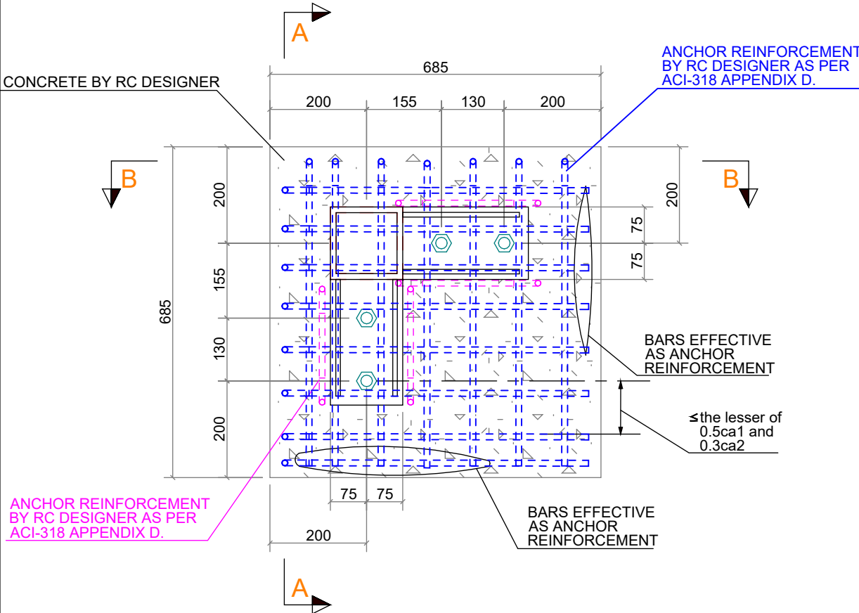
L TYPE BASE PLATE
