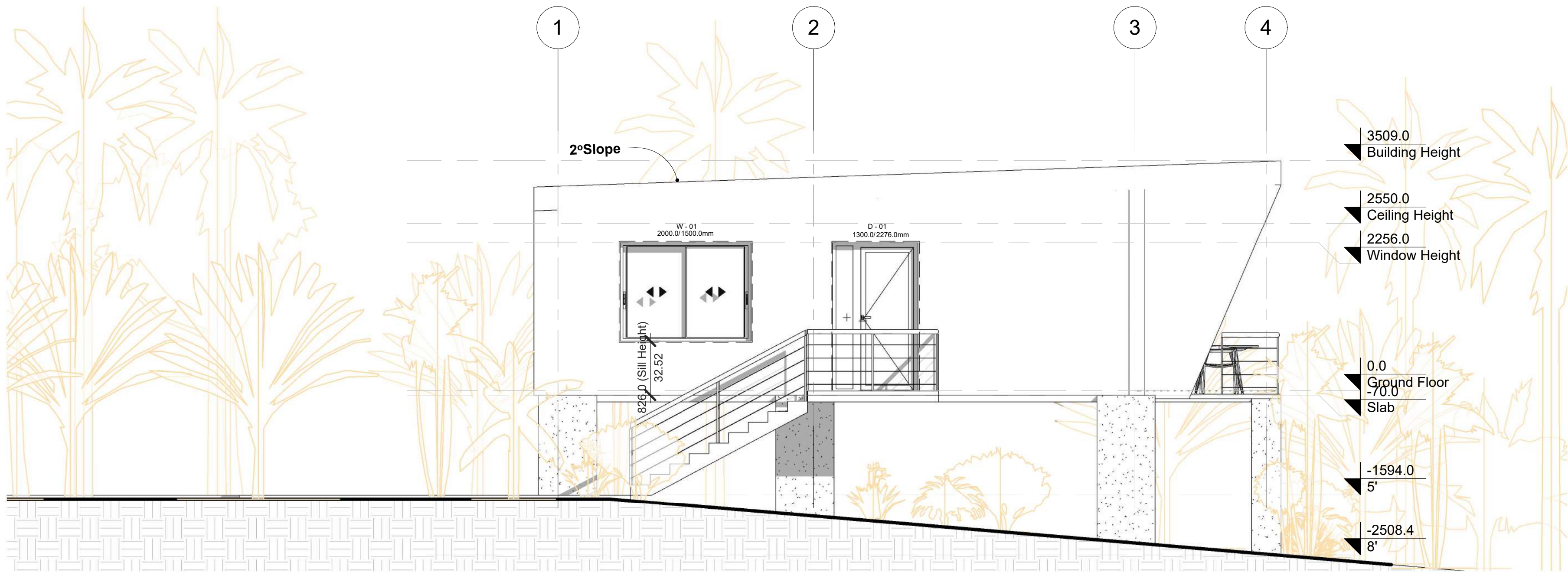
3 Left Elevation 1 : 50
