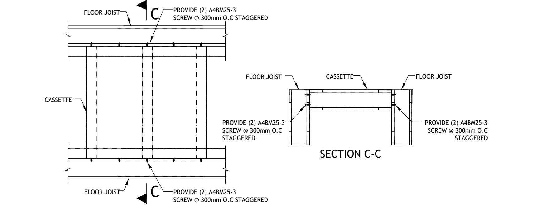
Cassette to Floor Joist Connection
