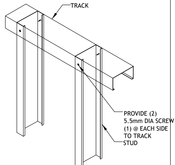
Stud to Top Track Connection (Internal Wall)
