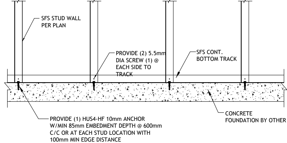
Typical Detail : Bottom Track to Concerrete Connection (Internal Wall)
