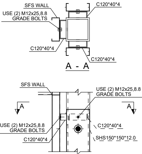
HRS Bracket Detail for Wall Connection
