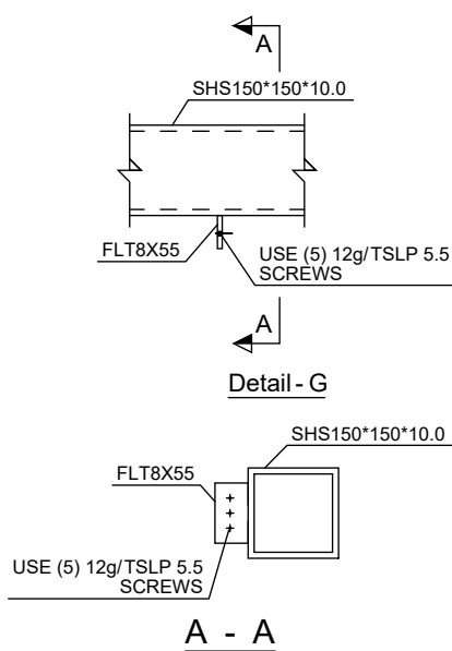
Cassette to Beam Connection
