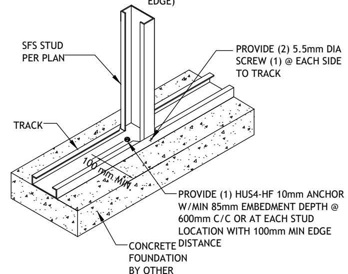
ENLARGE ISO SKETCH
