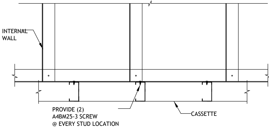
Internal Wall to Cassette Connection at Base
