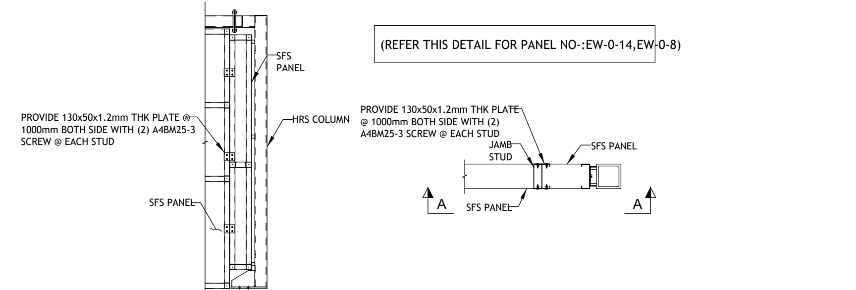
SFS Panel Connection Detail
