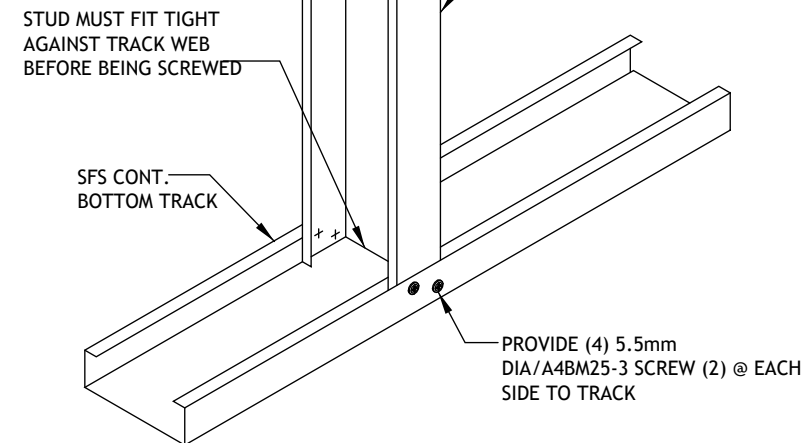
Stud to Bottom Track Connection (External Wall)
