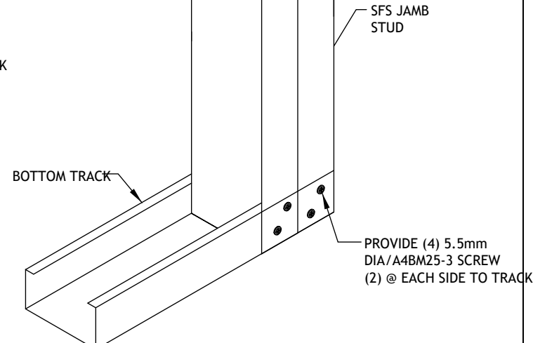
Box Jamb to Bottom Track Connection
