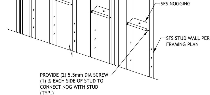
Hit and Miss Nogging to Stud Connection Detail
