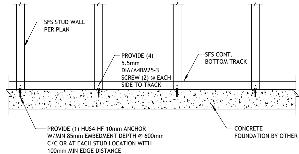
Typical Detail : SFS Bottom Track to Concerete Connection (External Wall)
