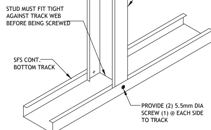
Stud to Bottom Track Connection (Internal Wall)
