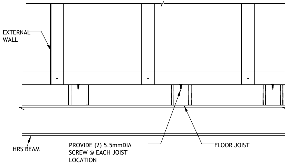
External Wall to Joist Connection at Base
