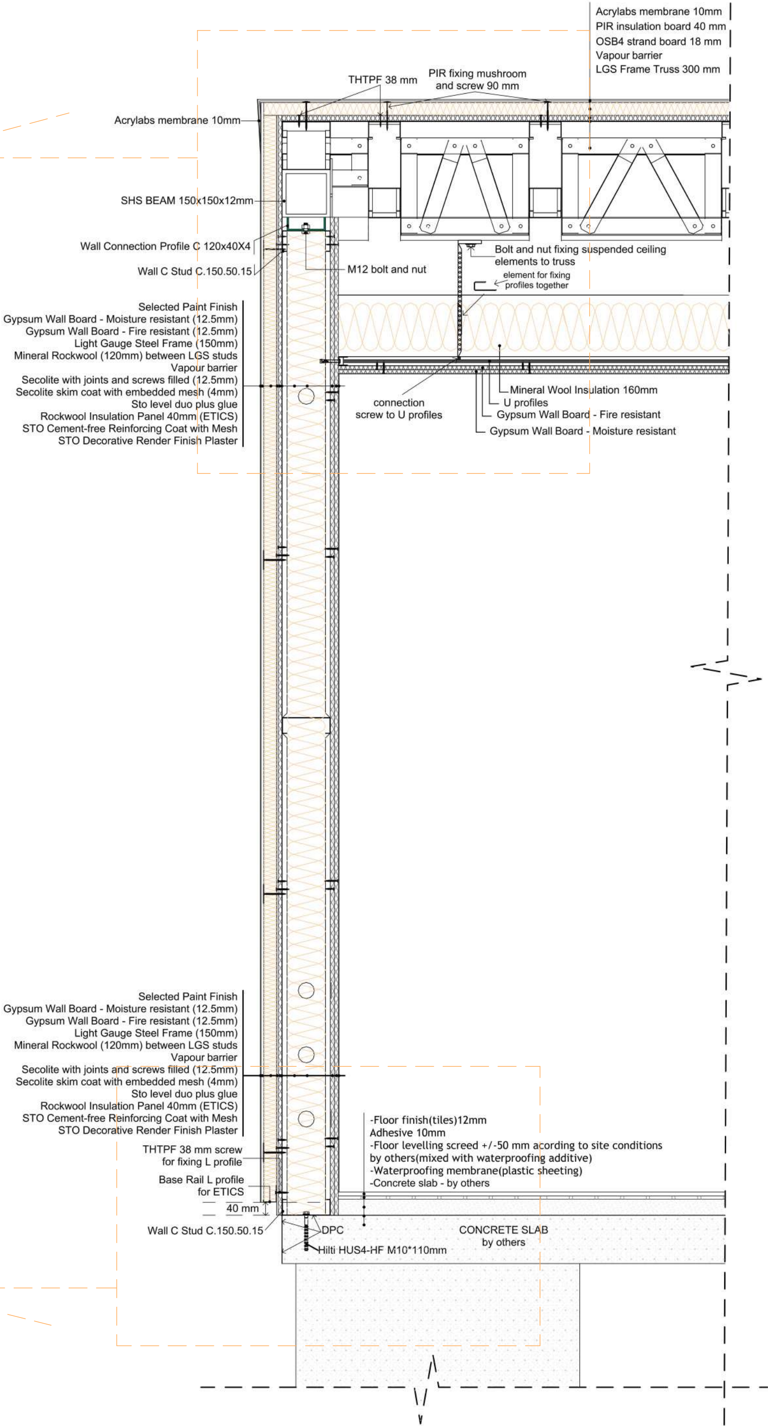
D10.Side wall Detail Sc: 1:12
