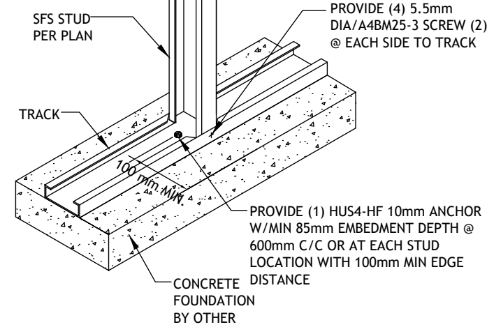
ENLARGE ISO SKETCH
