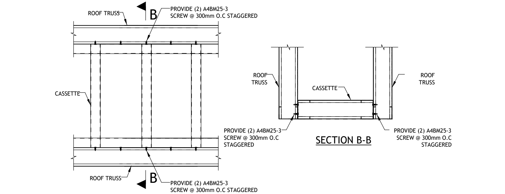
Cassette to Roof Trusses Connection
