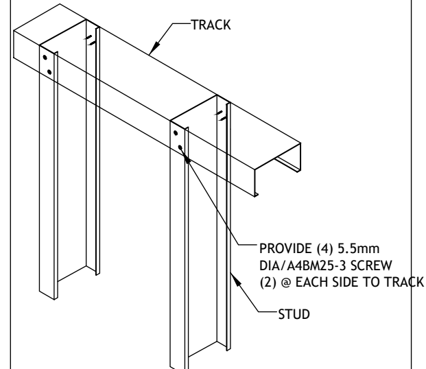
Stud to Top Track Connection (External Wall)
