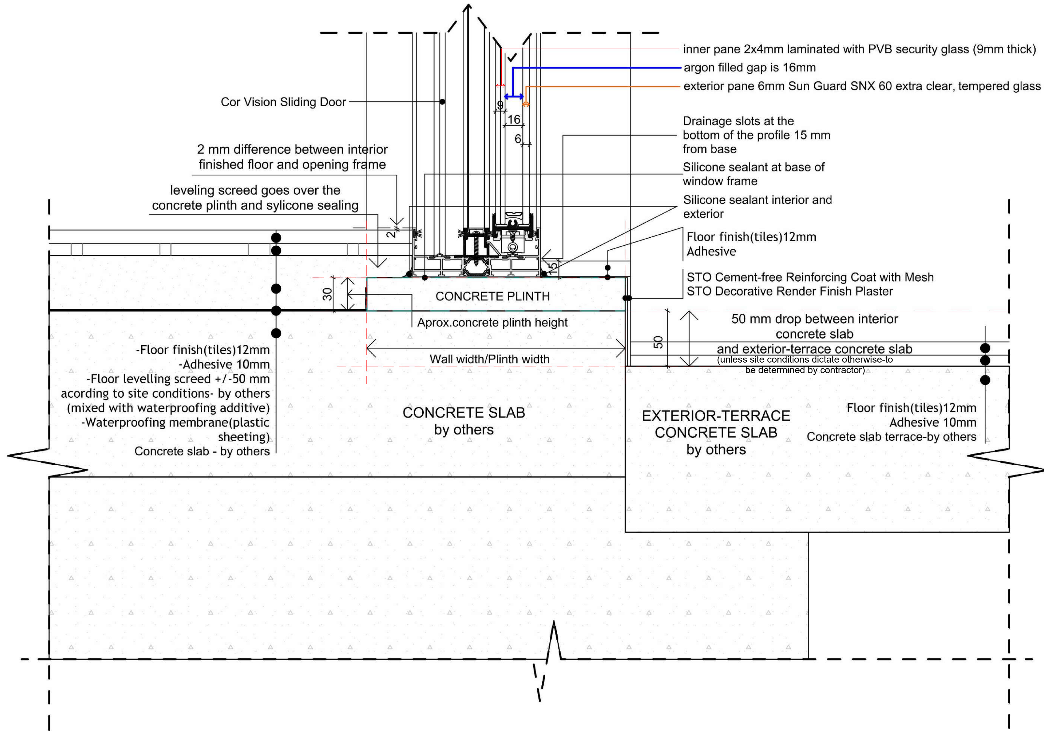
D9.Sliding Window/door fixing to base and concrete plinth detail Sc: 1:2
