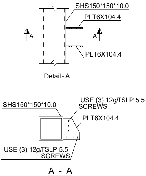
Typ. Truss Outside Plate Connection
