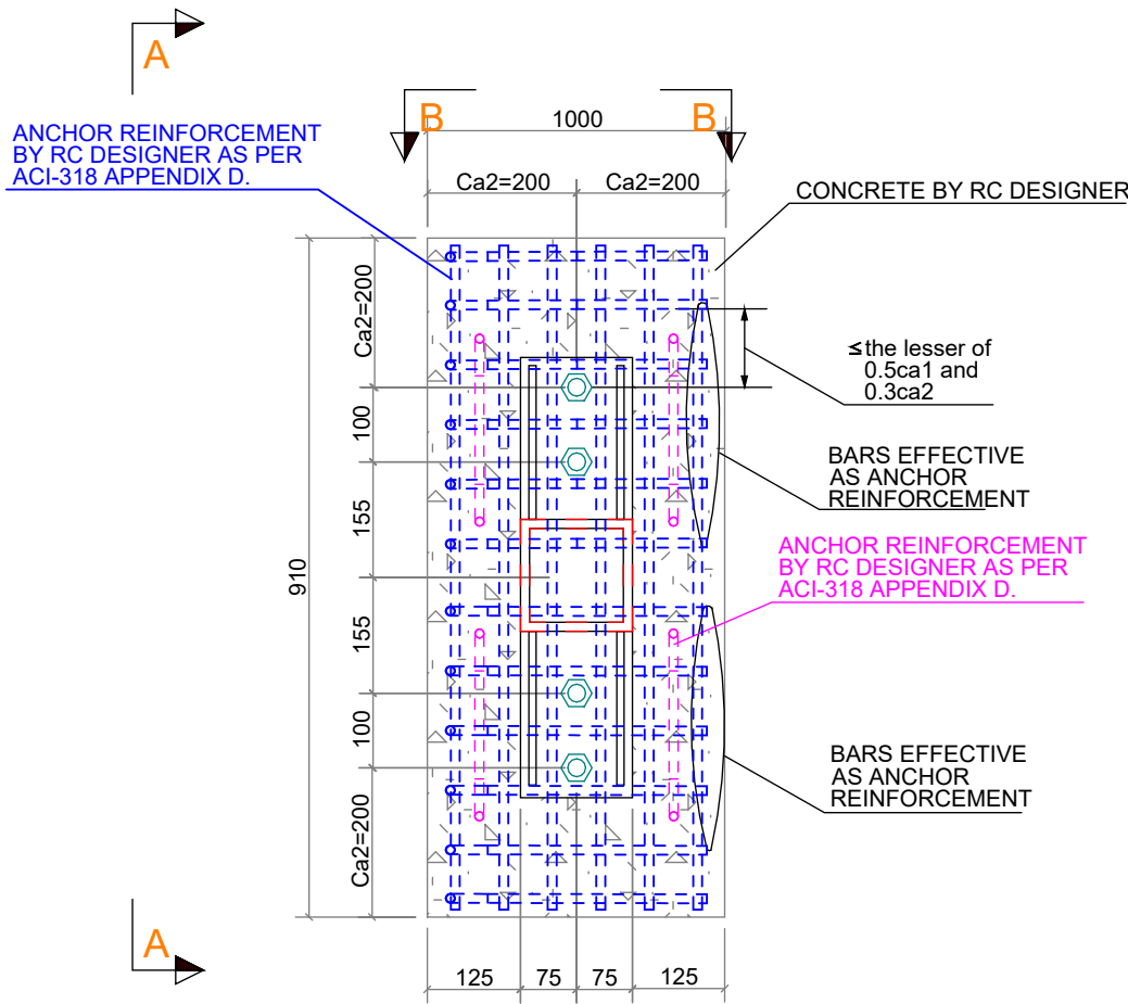
STRAIGHT BASE PLATE
