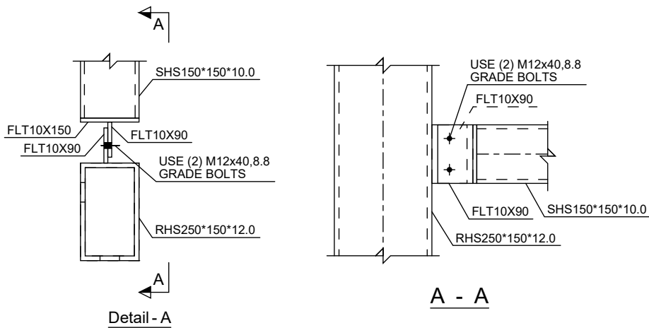
Typ. Fin Plate Connection Detail
