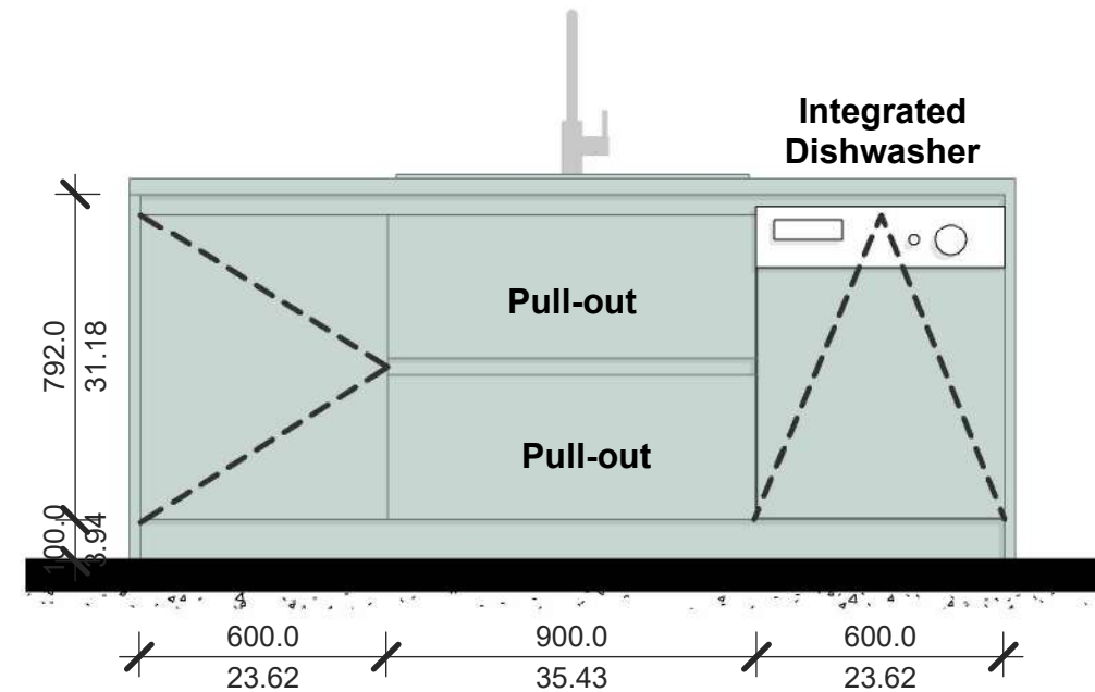
Island Front 1/20
