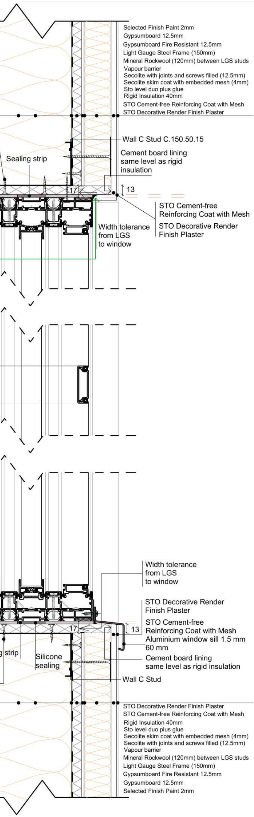
Windows with insect screens
