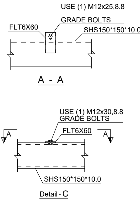
SFS Wall to HRS Beam Connection
