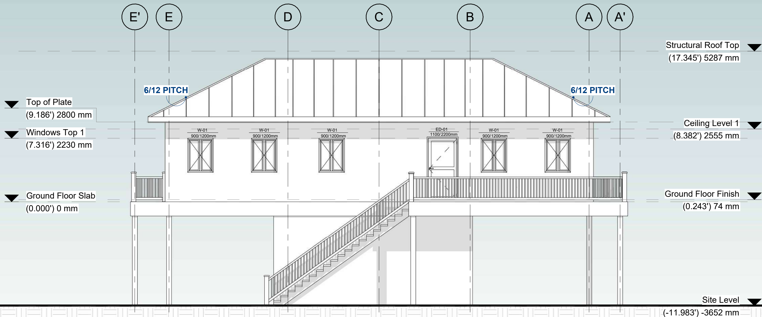
1 Rear Elevation 1 : 70
