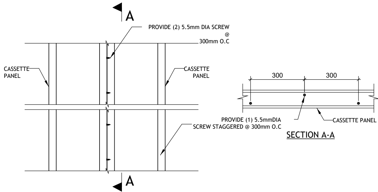
Cassette to Cassette Connection
