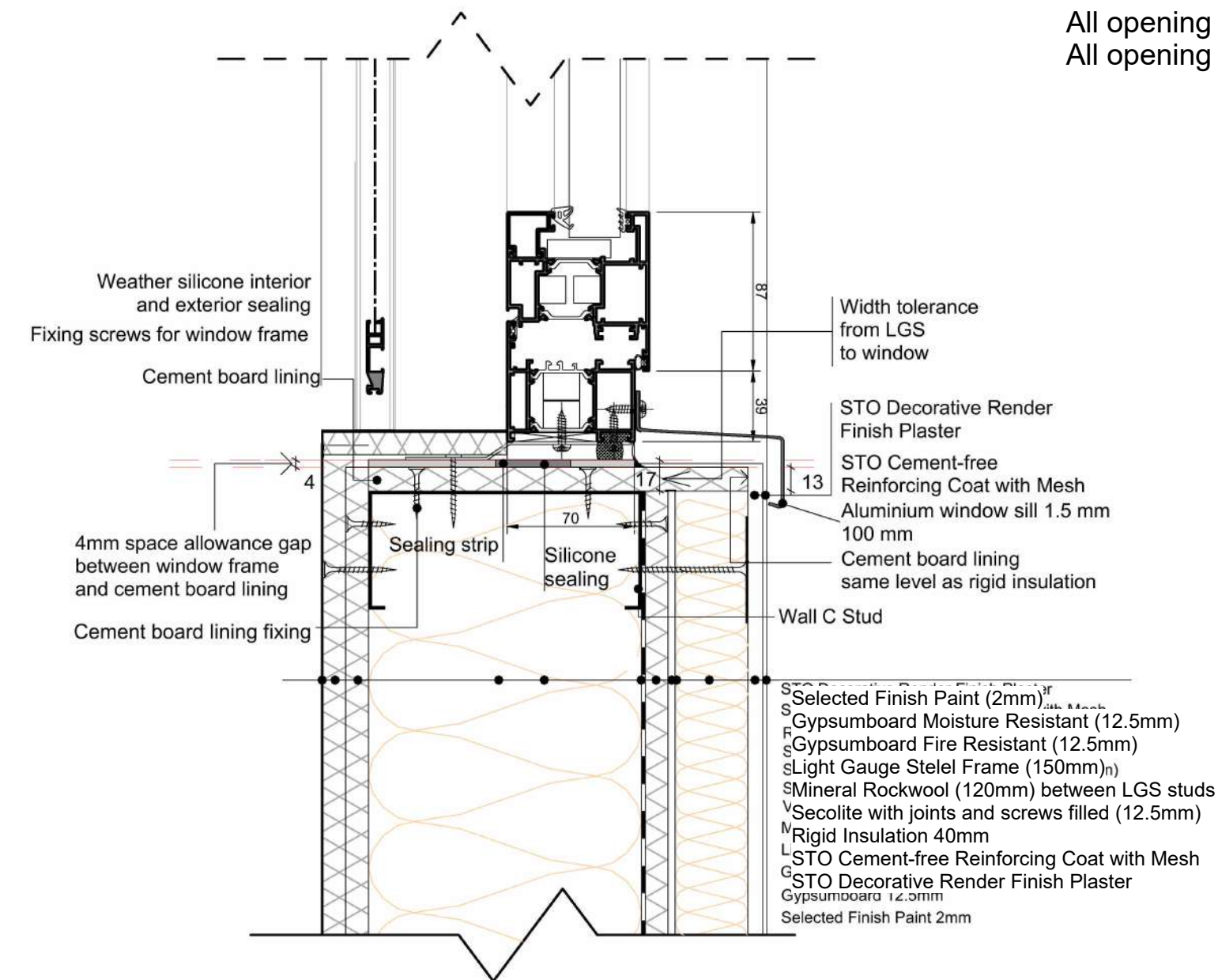
D.Casement Window Section with insect screens
