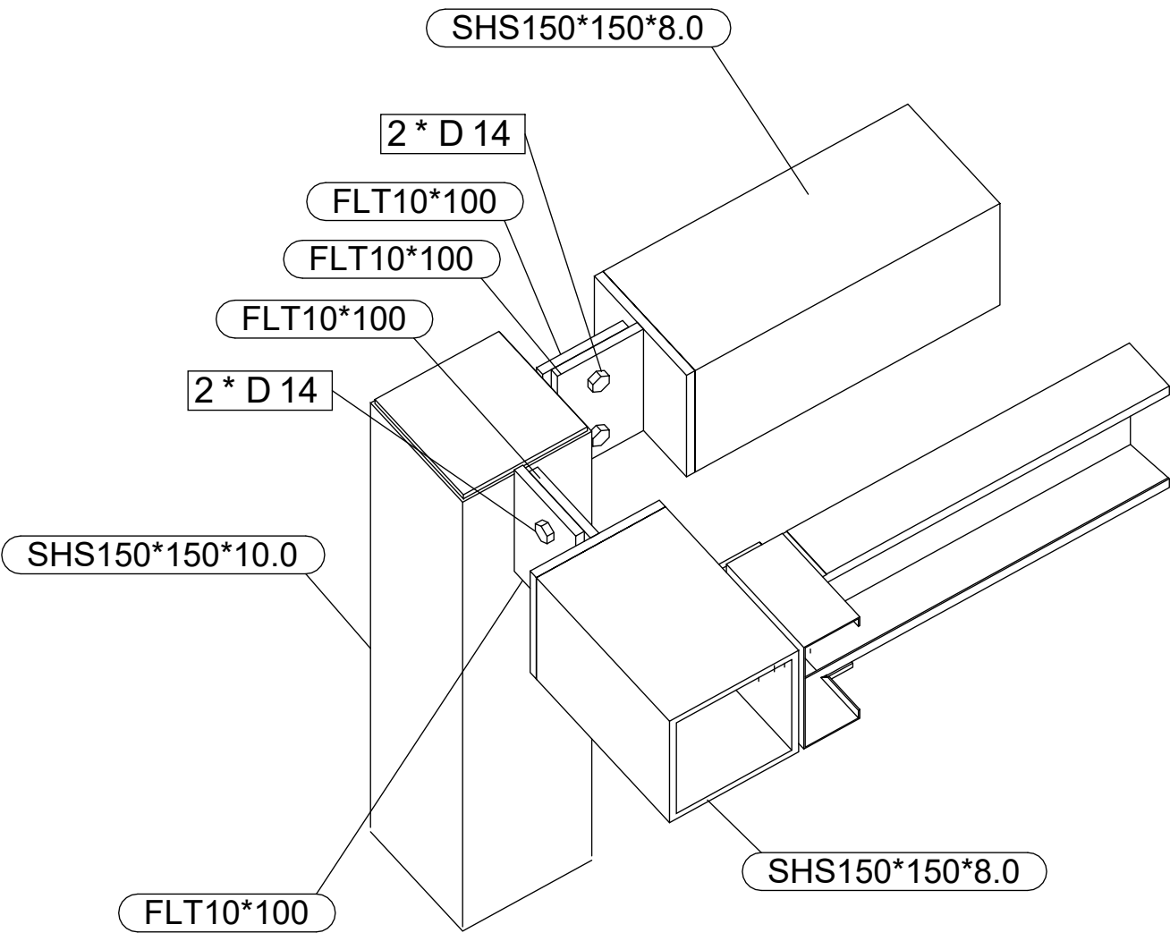
Typical Column to Beam Fine Plate Connection
