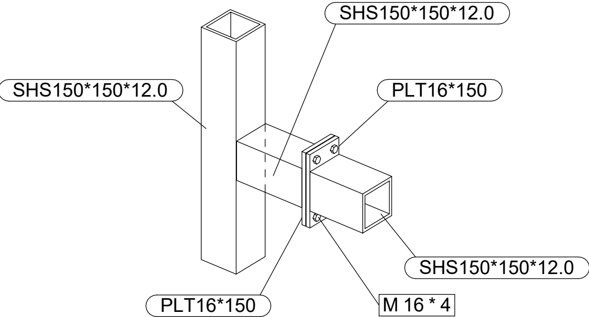
Typical Column Beam Stub Connection
