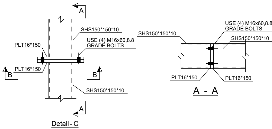
Typ. Horizontal Splice Connection
