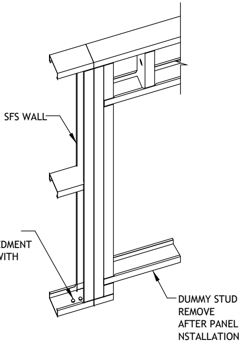
Typical Detail for Two Anchor at Jamb Location
