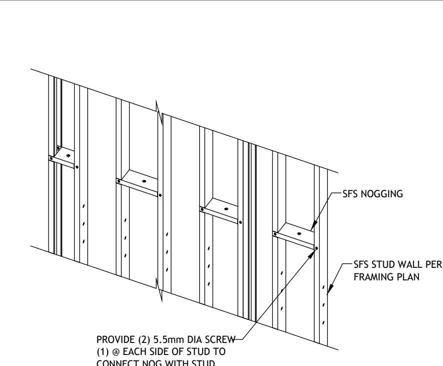
Hit and Miss Nogging to Stud Connection Detail
