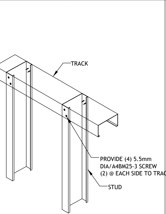
Stud to Top Track Connection (External Wall)
