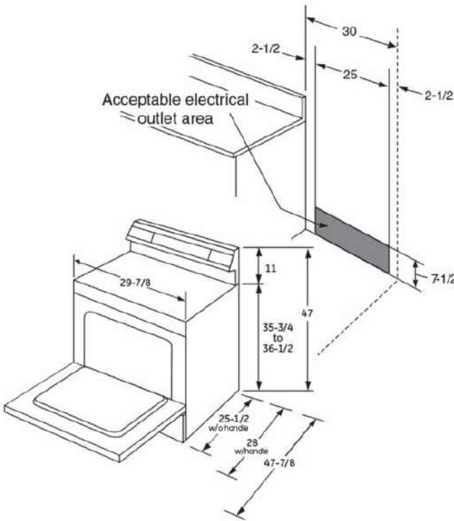
30" Free-Standing Electric Single Oven
