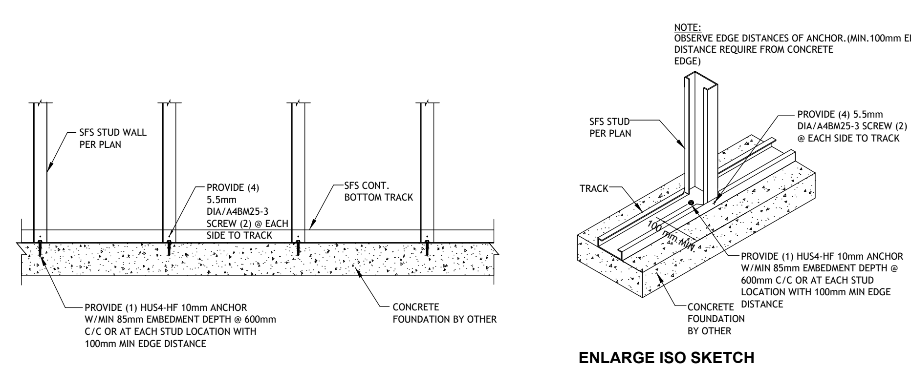
Typical Detail : SFS Bottom Track to Concrete Connection (External Wall)
