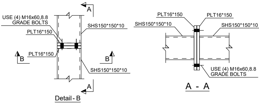
Typ. Vertical Splice Connection
