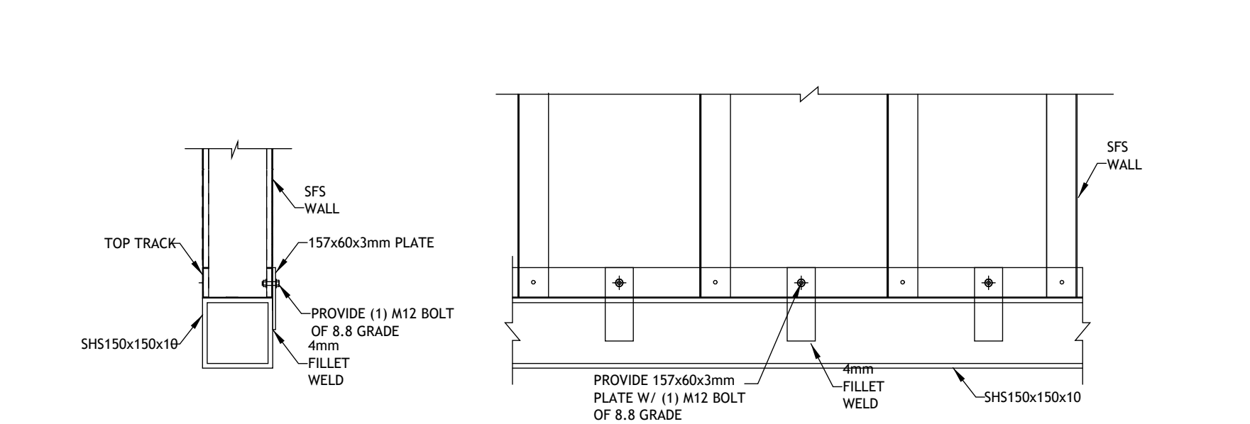
Cassette to Roof Truss Connection
