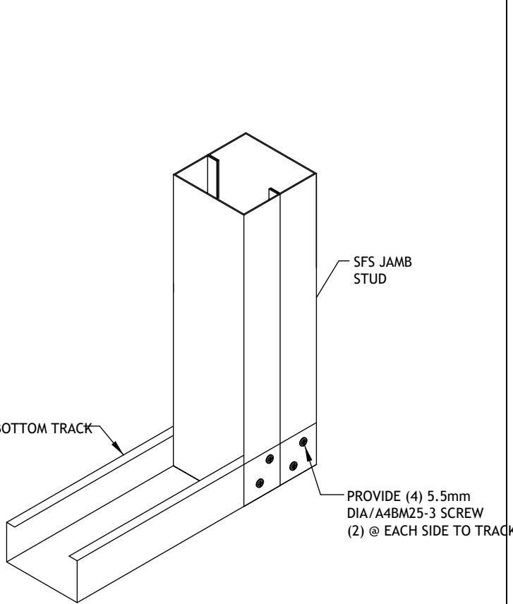
Box Jamb to Bottom Track Connection
