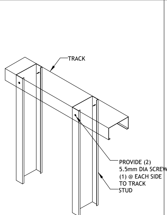
Stud to Top Track Connection (Internal Wall)
