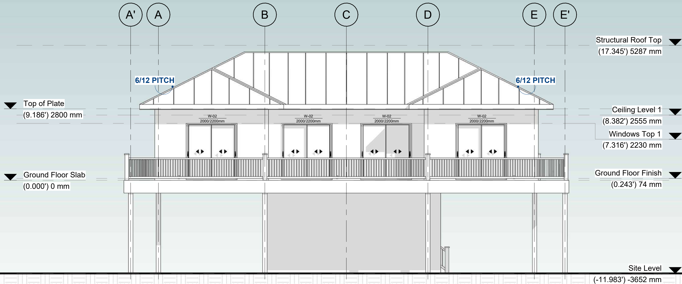
2 Front Elevation 1 : 70
