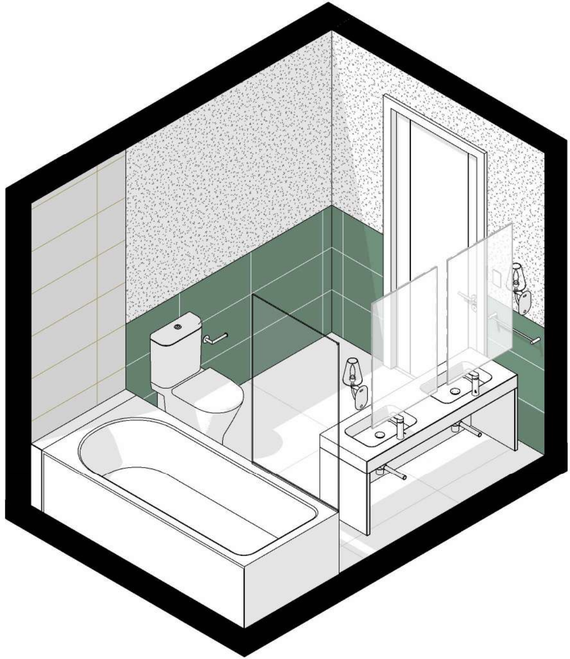
2 Bathroom Iso.View 2
