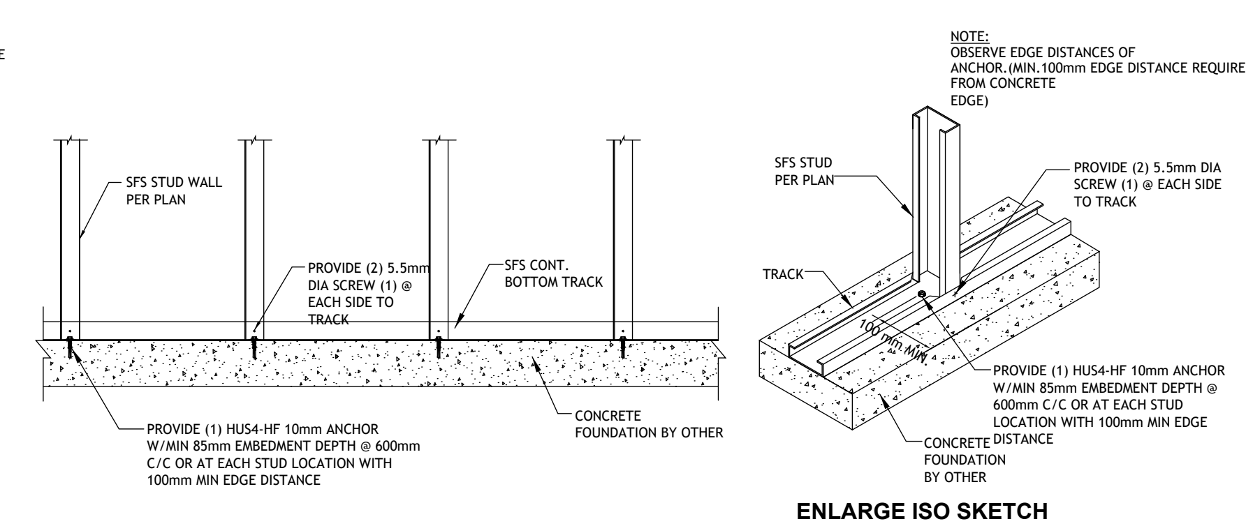
Typical Detail : Bottom Track to Concrete Connection (Internal Wall)
