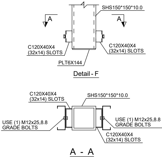
Typ. Lintel to Wind Post Connection
