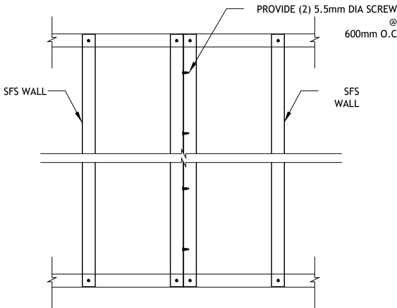
Typical Wall to SFS Wall Connection
