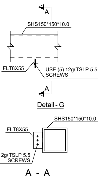
Cassette to Beam Connection
