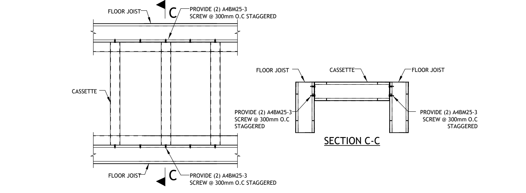
Cassette to Floor Joist Connection
