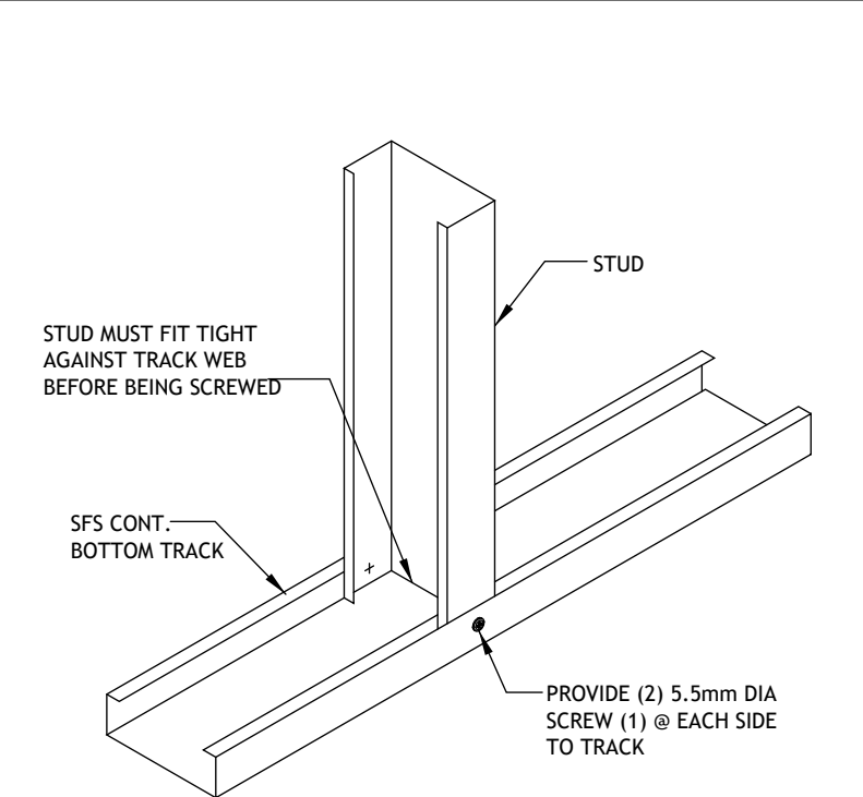
Stud to Bottom Track Connection (Internal Wall)
