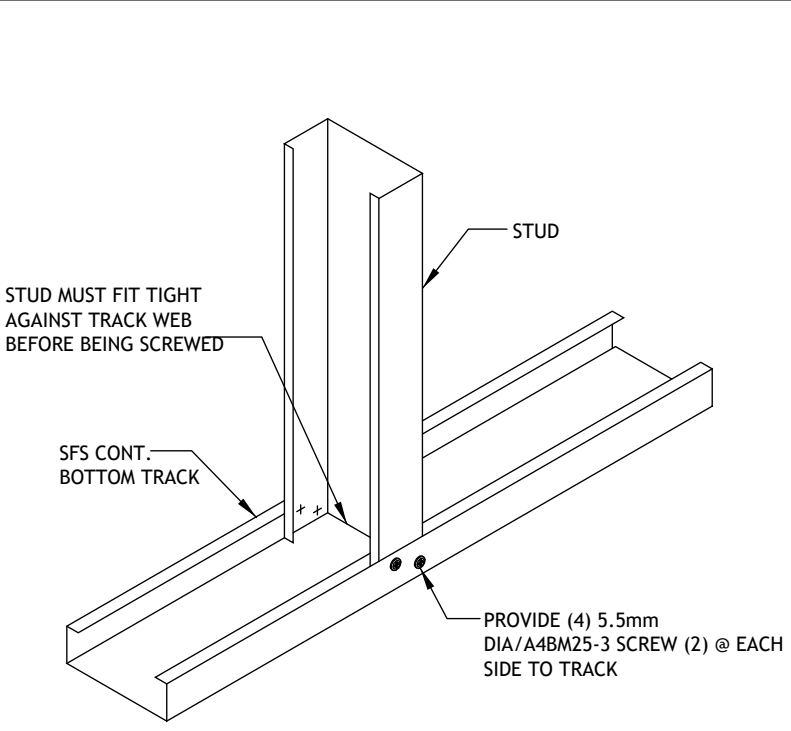
Stud to Bottom Track Connection (External Wall)
