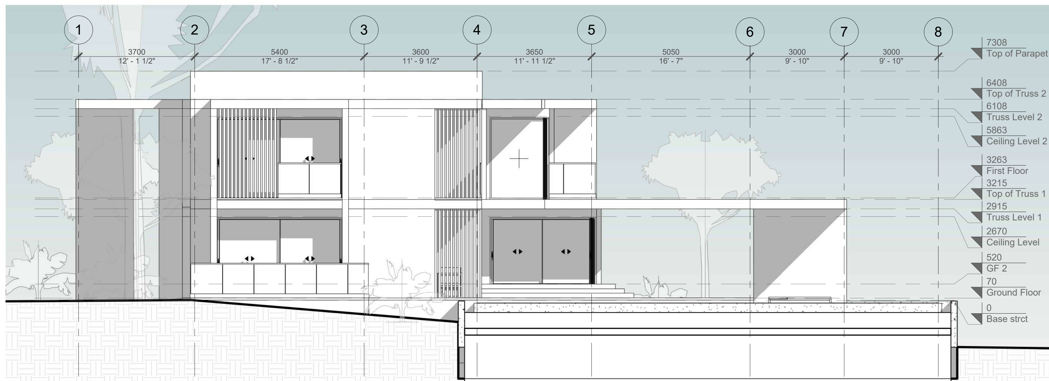
2 Left Elevation 1 : 70
