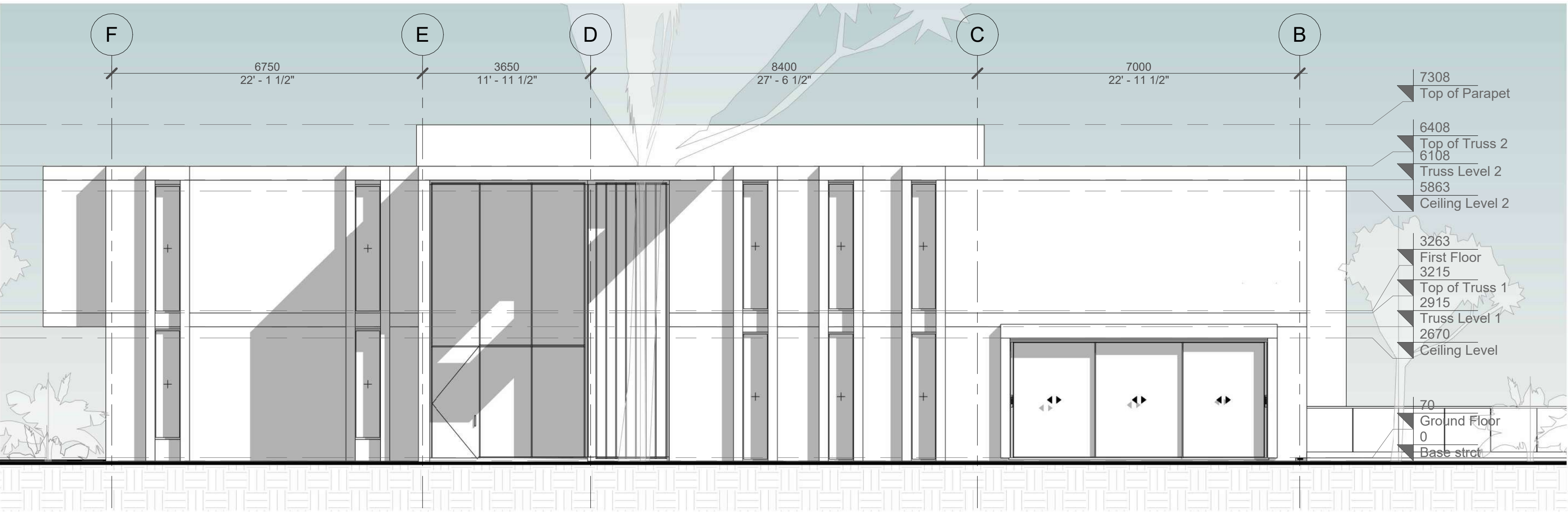
1 Rear Elevation 1 : 70
