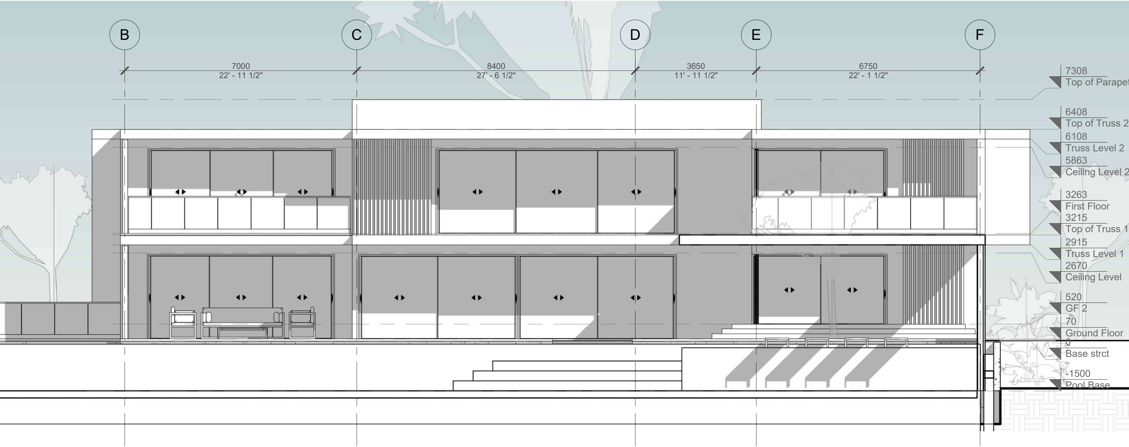
2 Front Elevation 1 : 70
