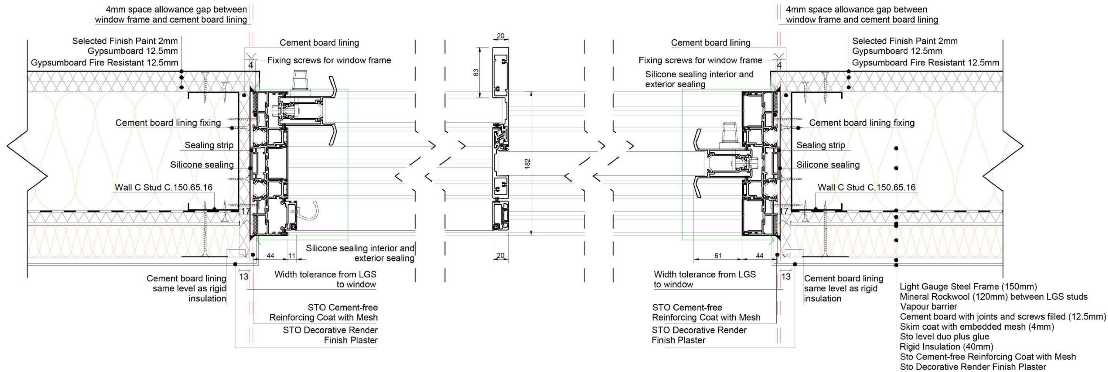
D5.Sliding Door/Window Floor Plan with insect screens
