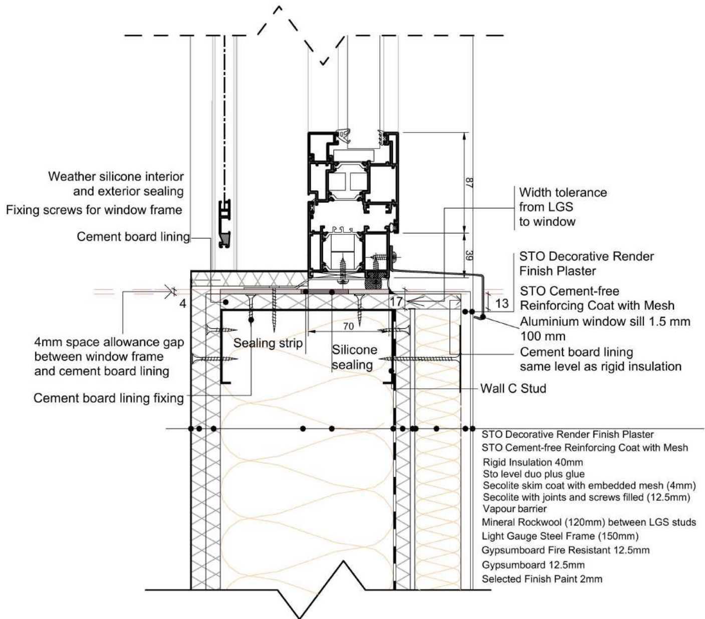
D4.Sliding Window Section with insect screens
