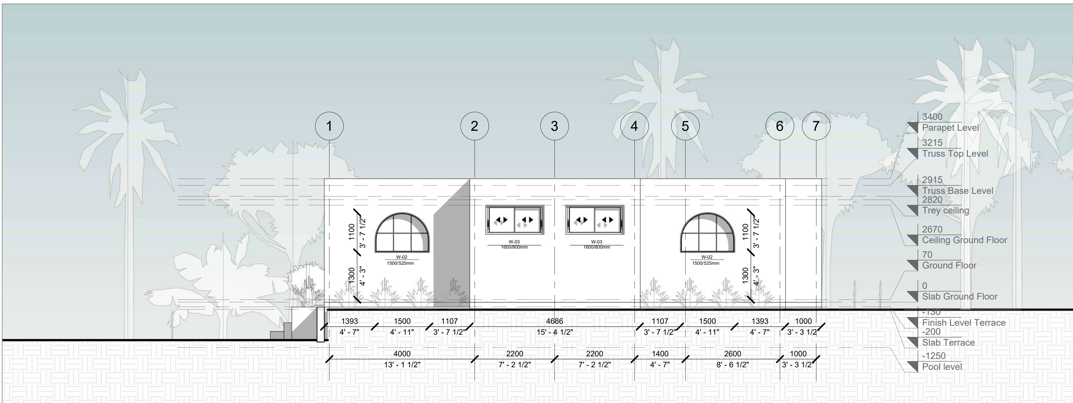
1 Left Elevation 1 : 60
