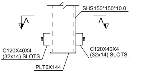
Detail - F
