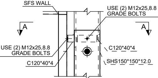
Typ. Truss Outside Plate Connection
