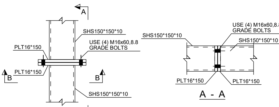
Detail - C
