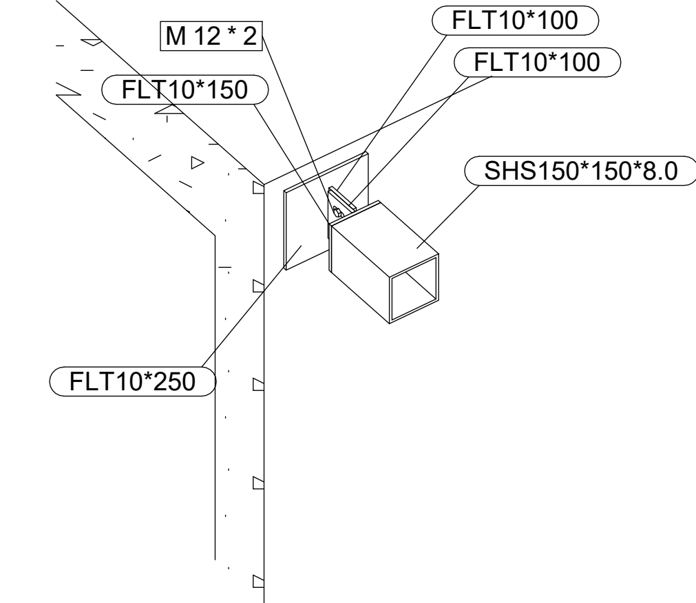
Typical Beam to Concrete Connection
