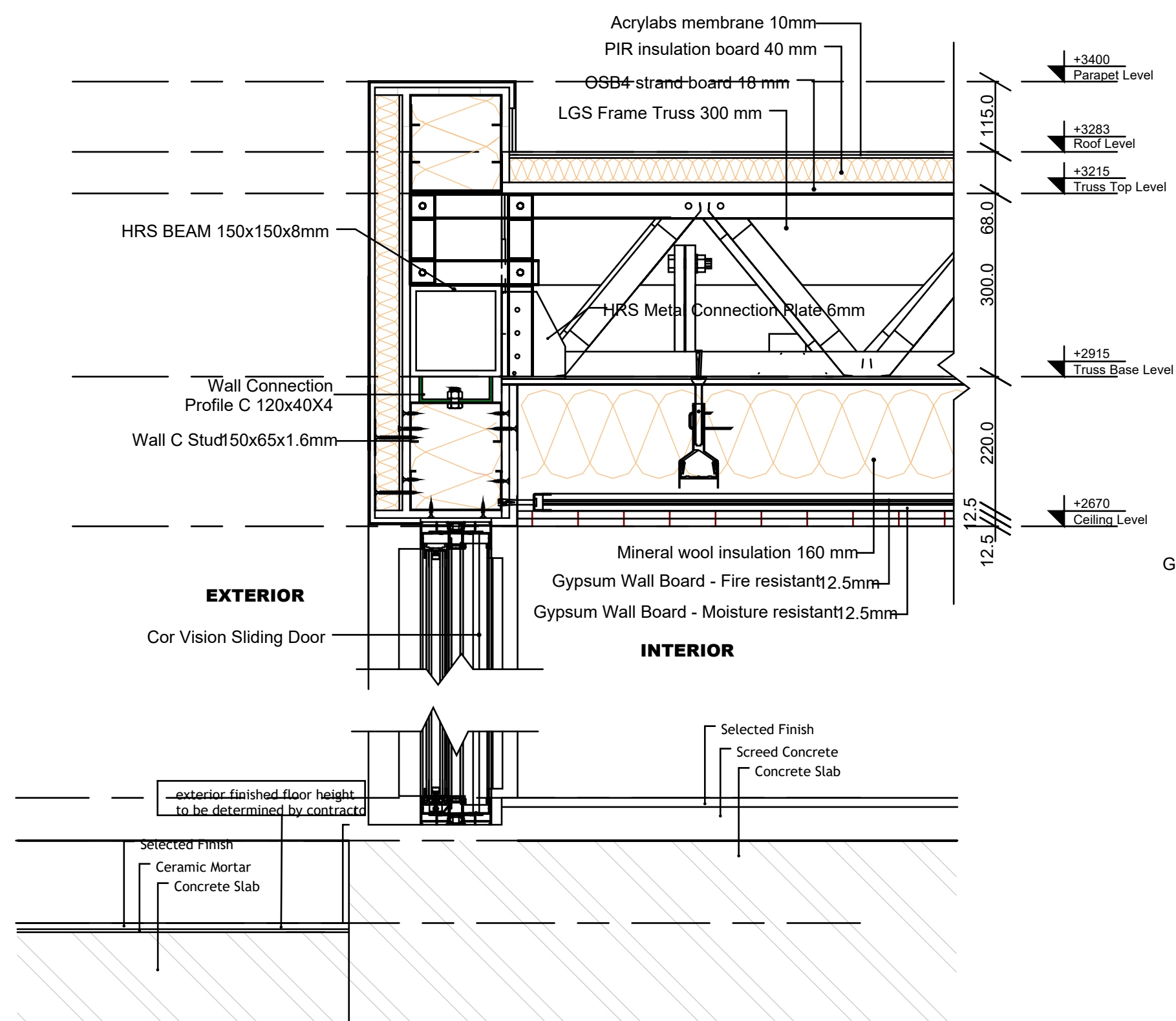
D6: Ground Floor detail Sc: 1:8
