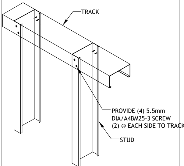
Stud to Top Track Connection (External Wall)
