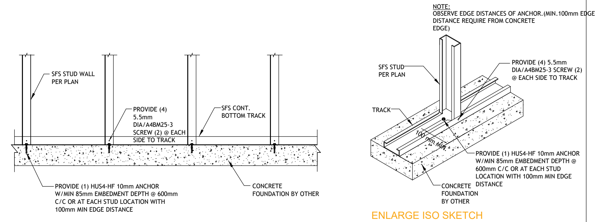
Typical Detail : SFS Bottom Track to Concerete Connection (External Wall)
