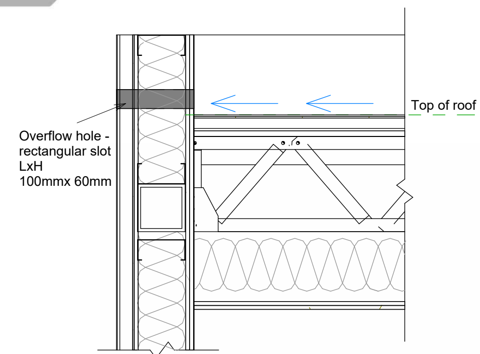
Roof parapet overflow hole
