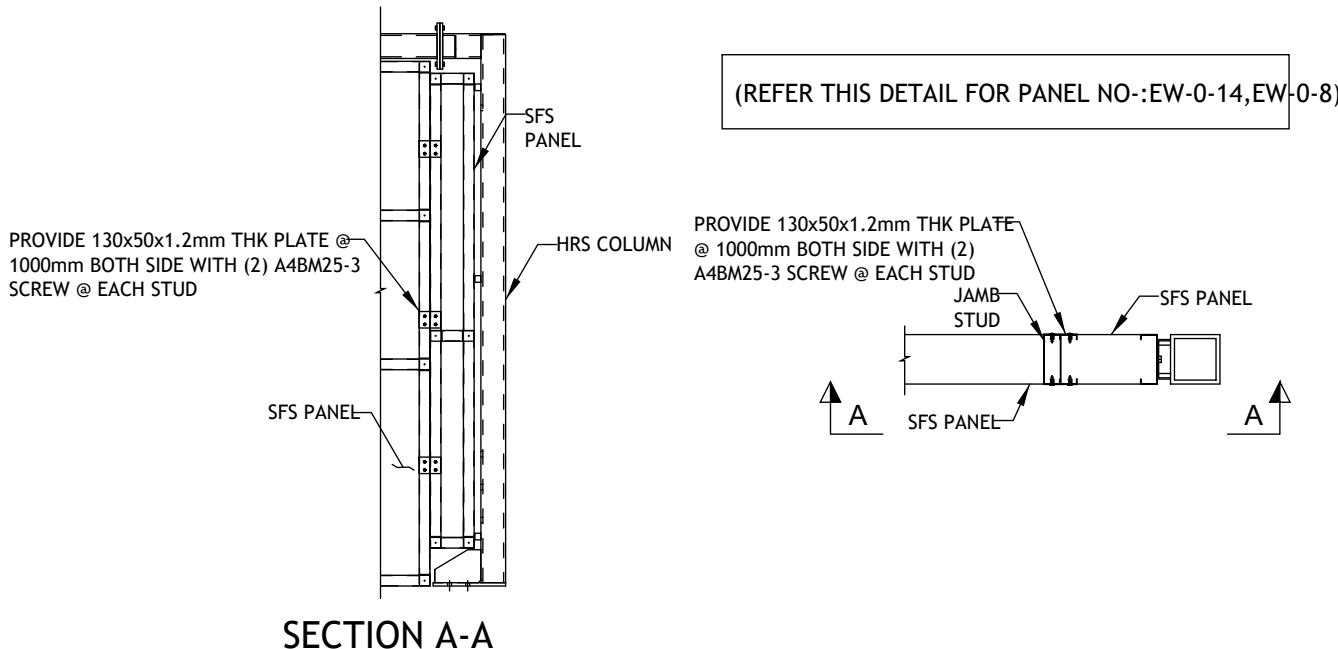
SFS Panel Connection Detail
