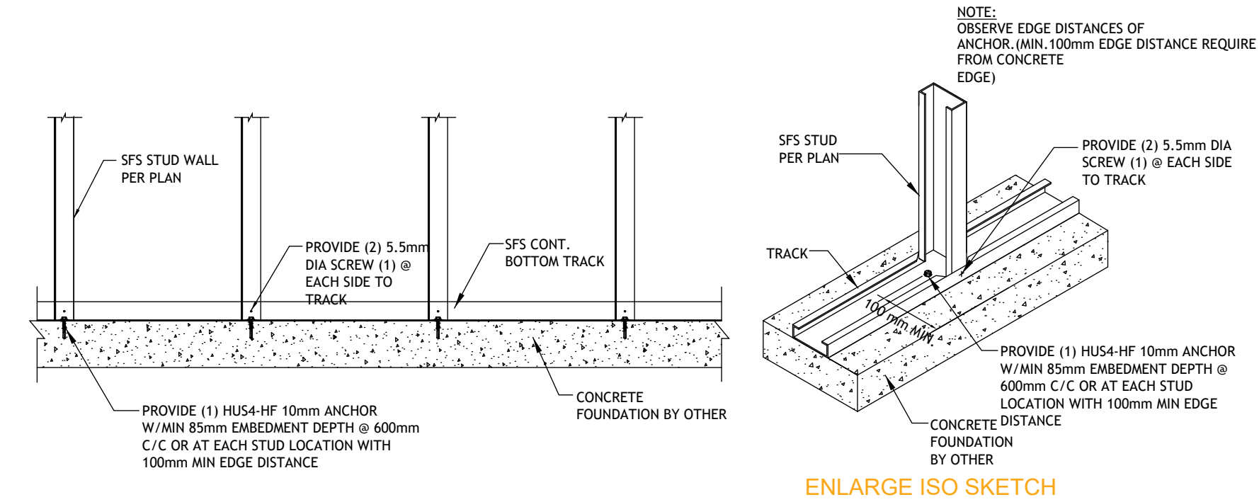
Typical Detail : Bottom Track to Concerete Connection (Internal Wall)
