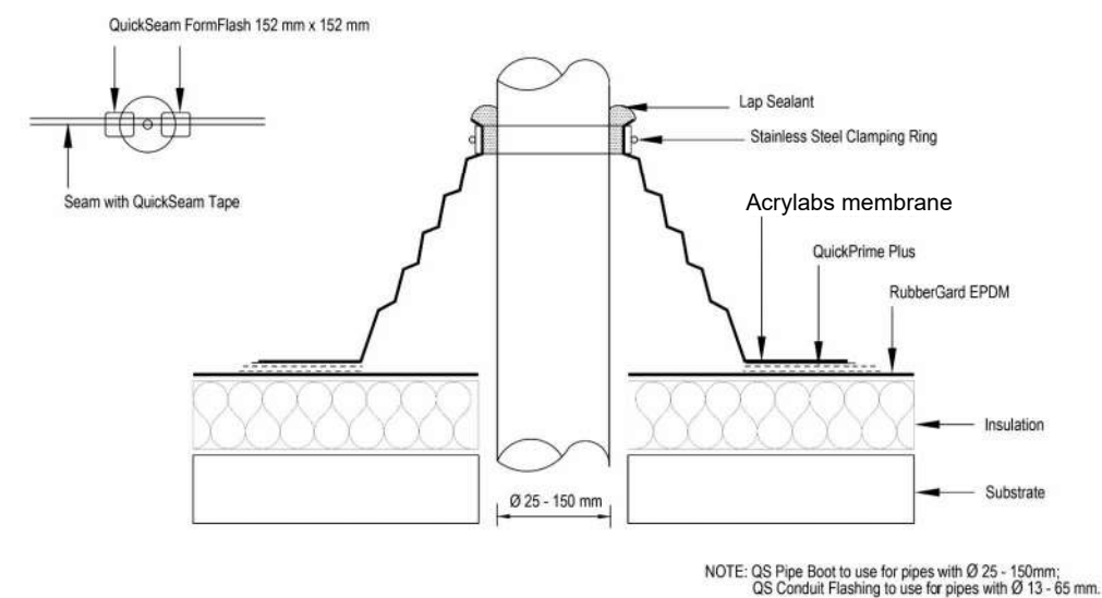
Roof Breather Pipe Detail
