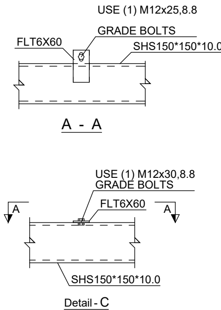
SFS Wall to HRS Beam Connection
