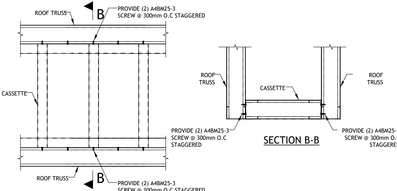
Cassette to Roof Trusses Connection
