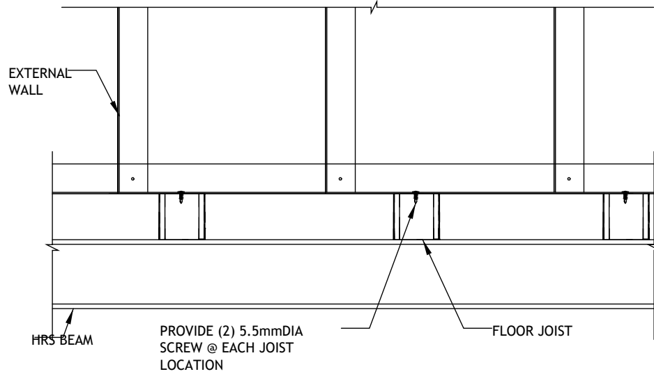
External Wall toJoist Connection at Base
