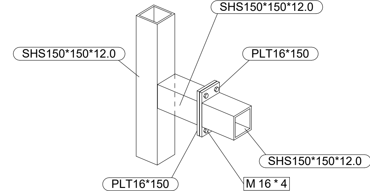
Typical Column Beam Stub Connection
