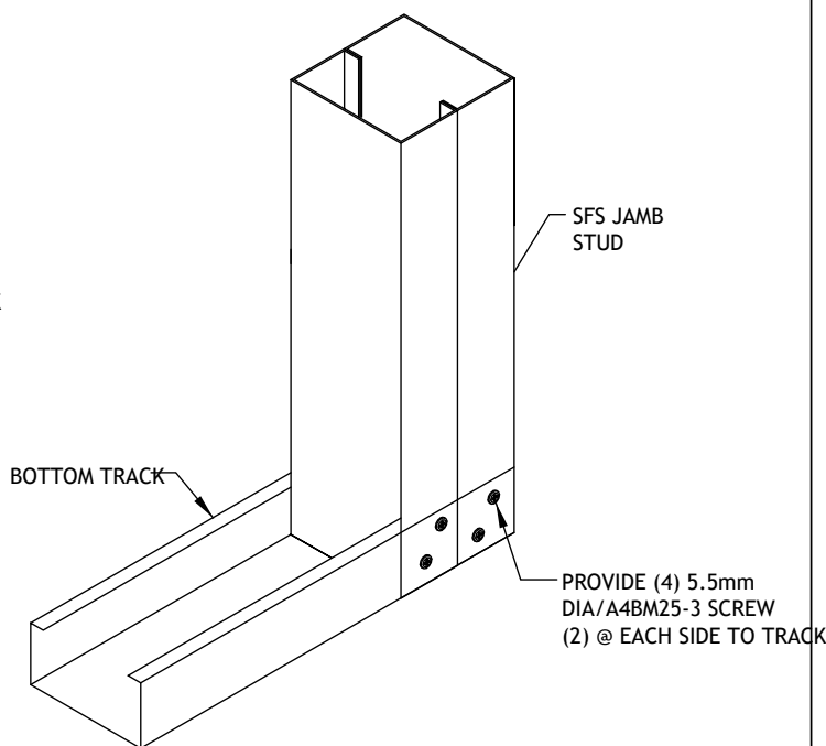
Box Jamb to Bottom Track Connection
