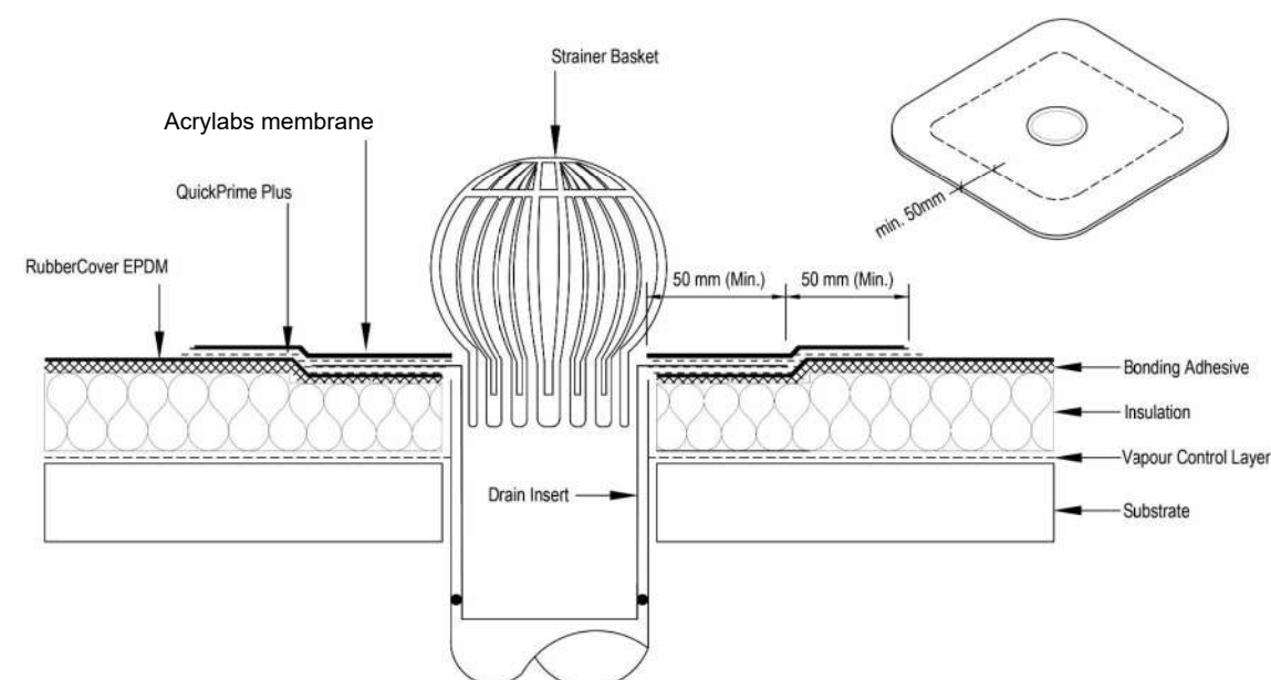
Roof Drain Detail
