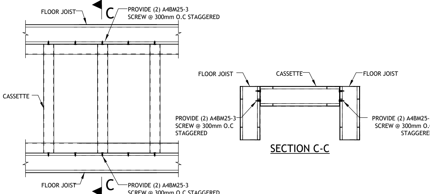
Cassette to Floor Joist Connection
