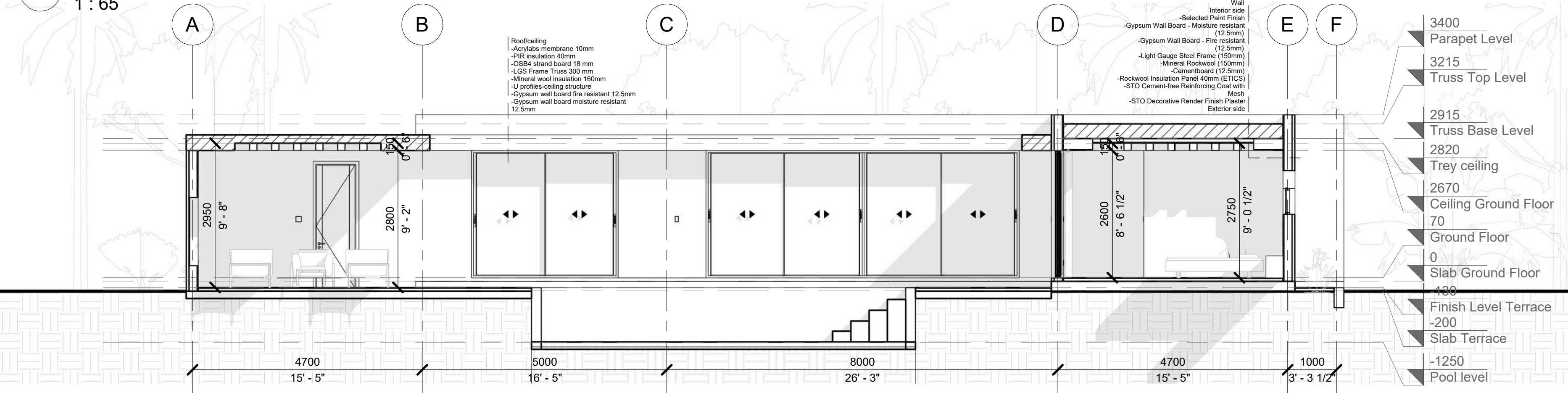
Section 2
