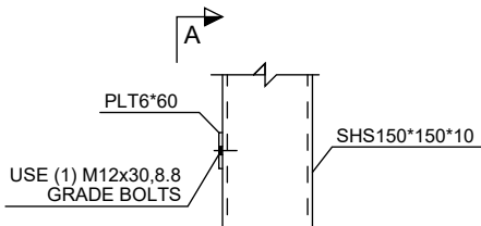
Detail - E
