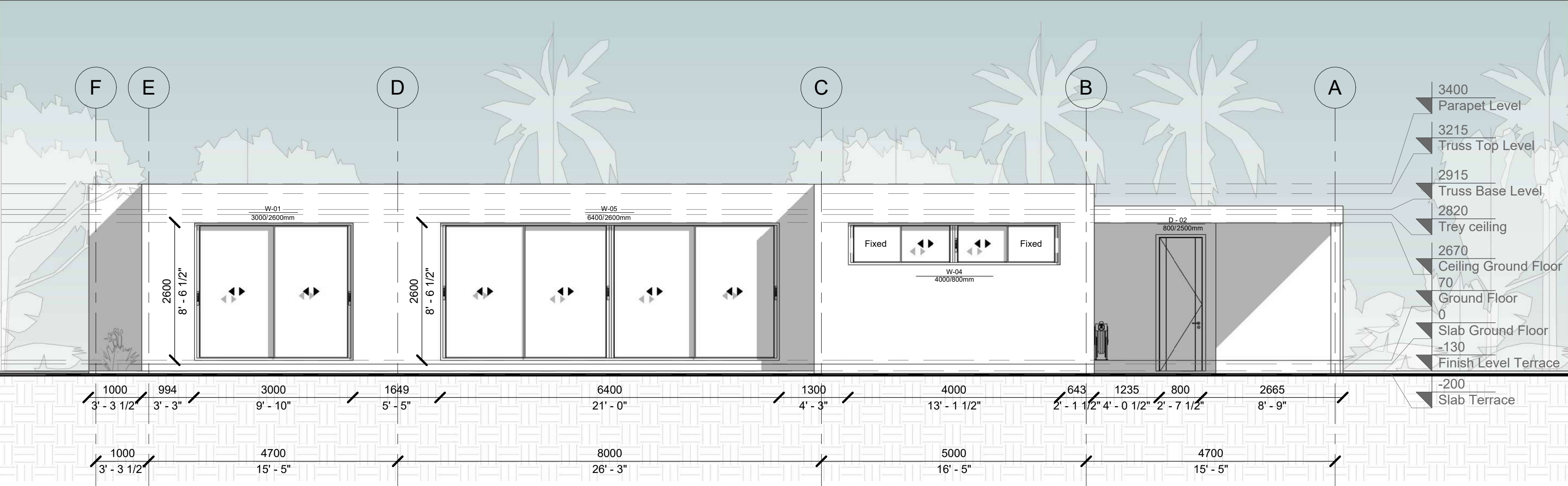
1 Front Elevation 1 : 60
