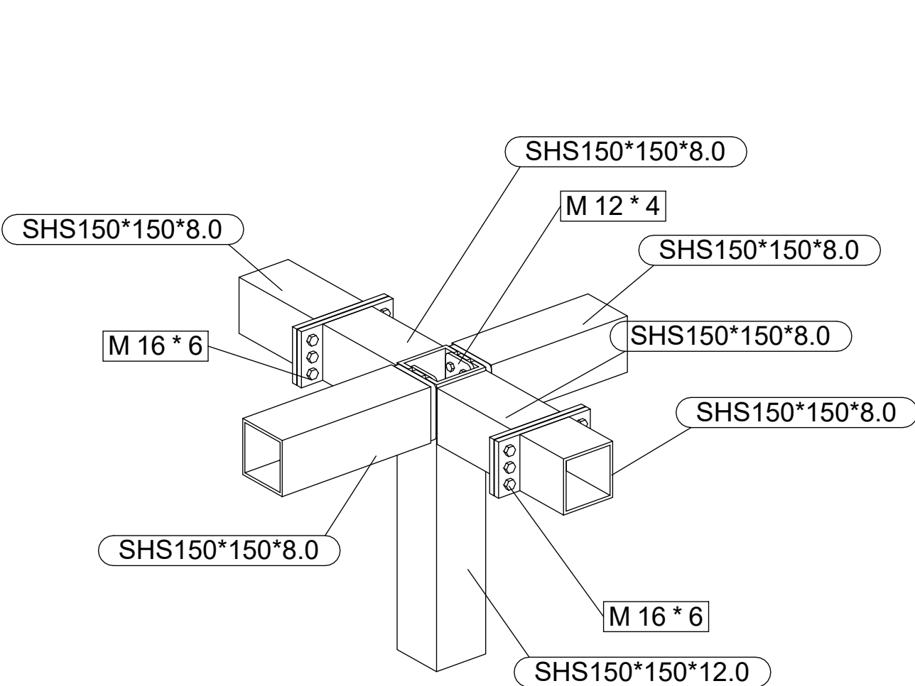
Typical Roof Column Beam Connection
