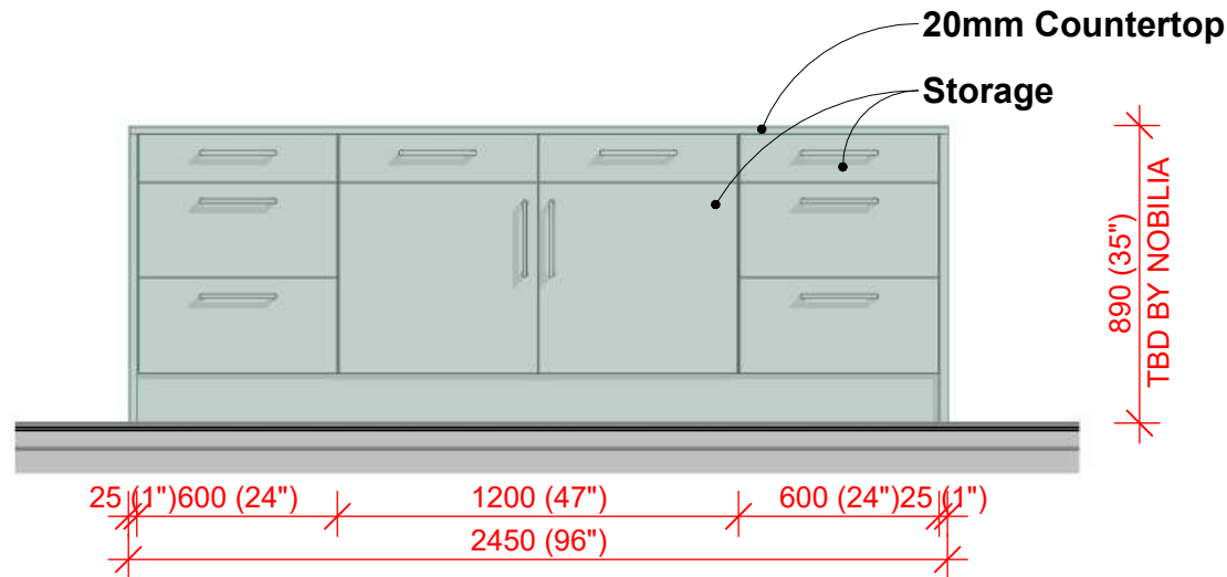
2 K2 Island Front 1 : 25
