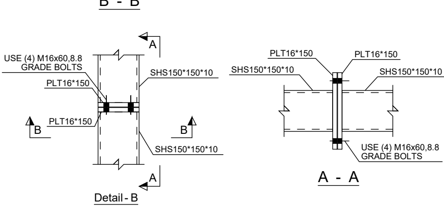
Typ. Vertical Splice Connection
