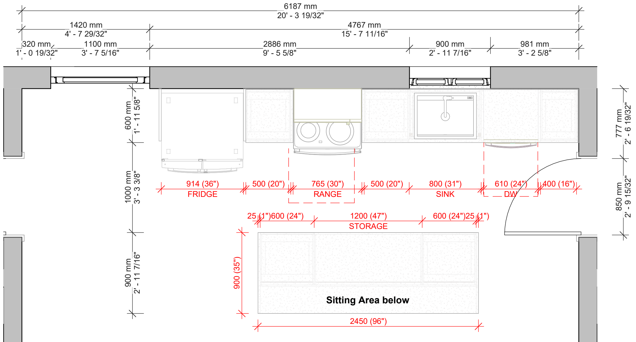
1 Kitchen Plan 1 : 25
