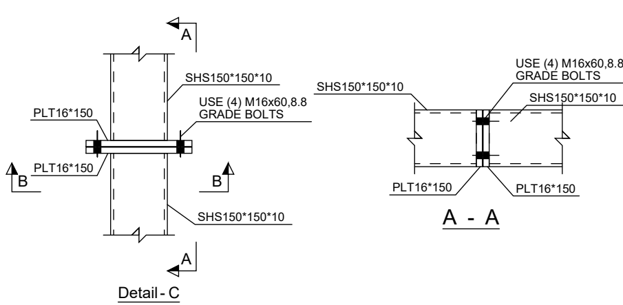
Typ. Horizontal Splice Connection
