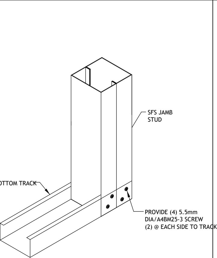
Stud to Bottom Track Connection (Internal Wall)
