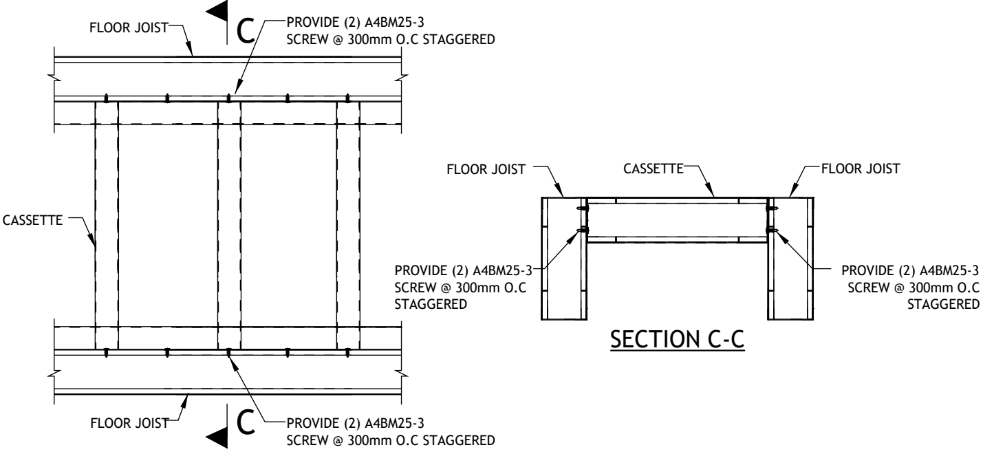
Cassette to Floor Joist Connection
