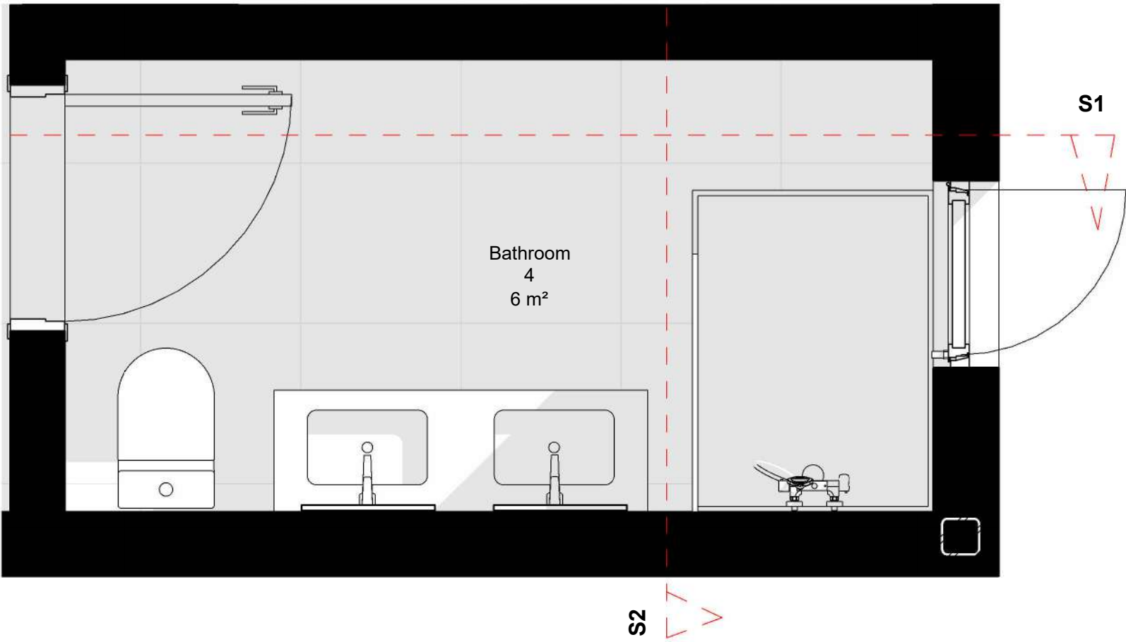
3 Bathroom plan 1 : 20
