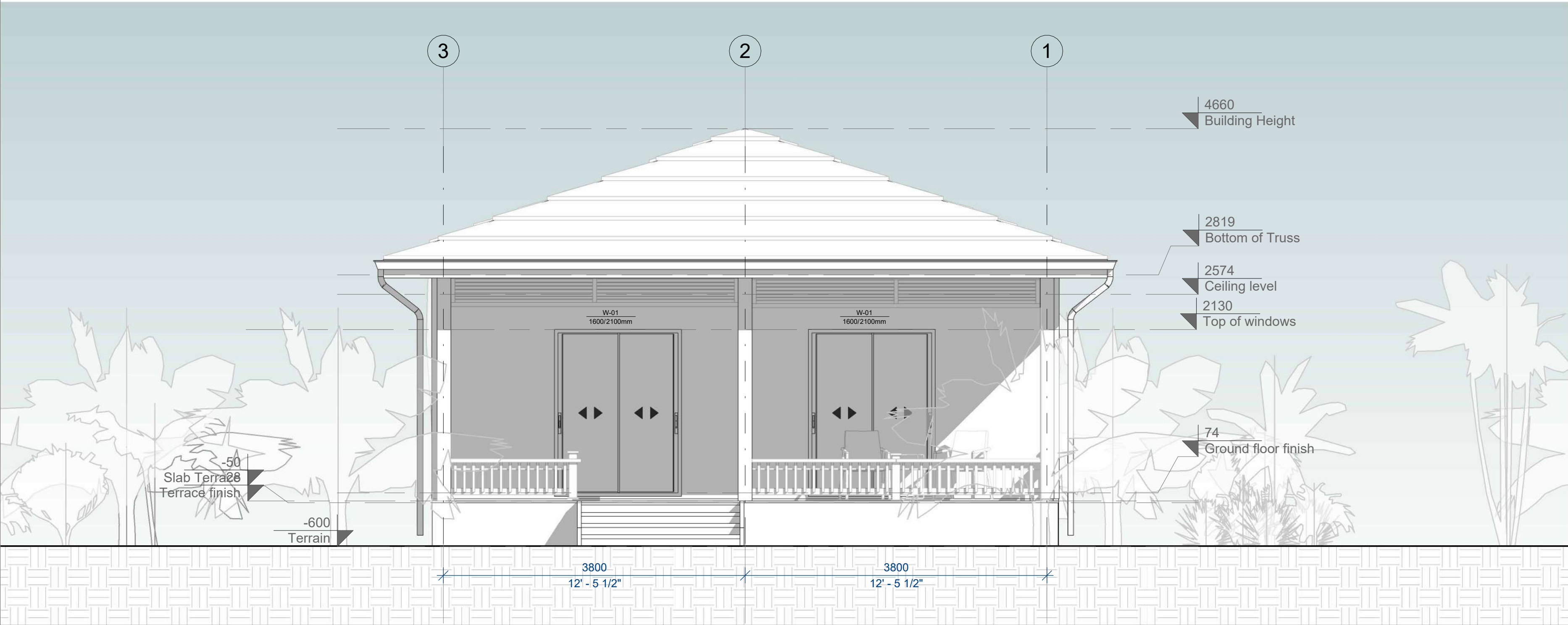
3 Left Elevation 1 : 40
