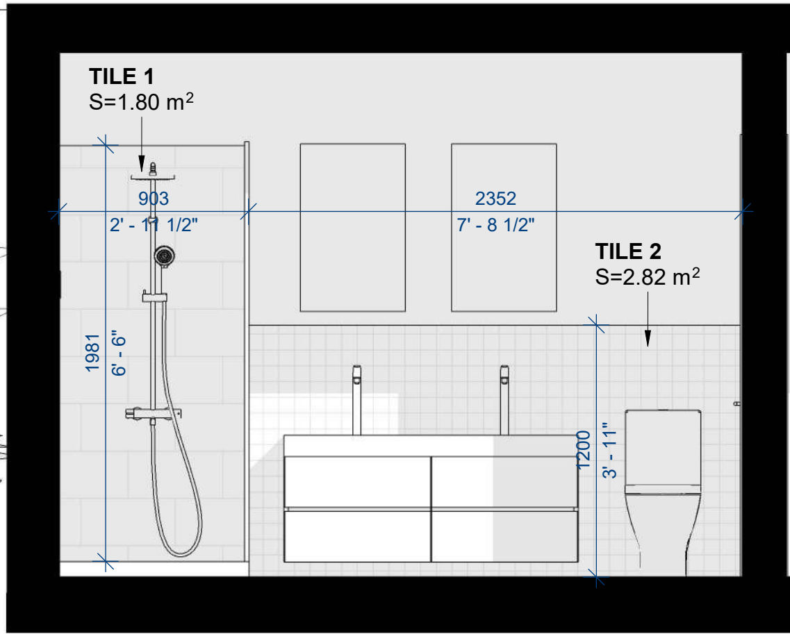
1 Bathroom - S1 1 : 25
