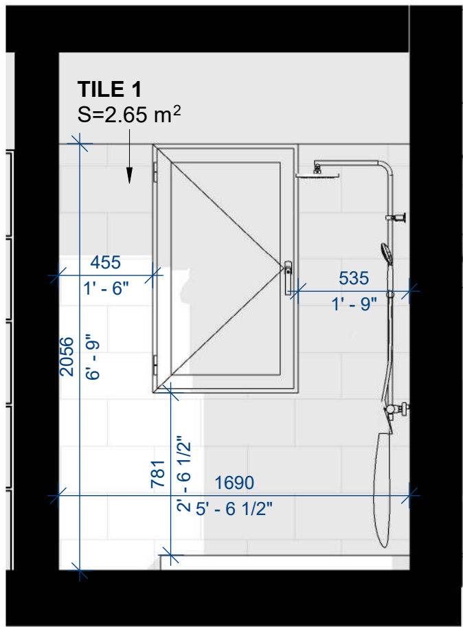
2 Bathroom - S2 1 : 25
