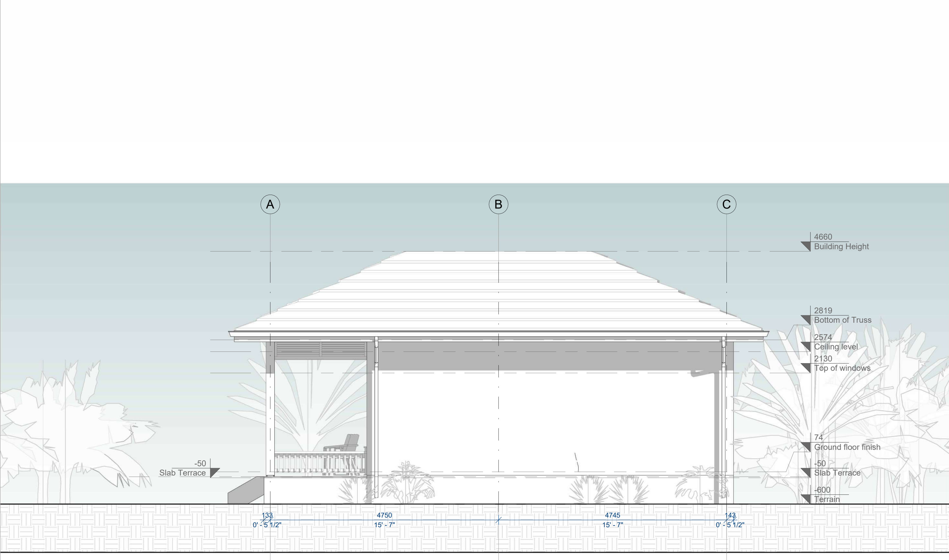
2 Rear Elevation 1 : 40
