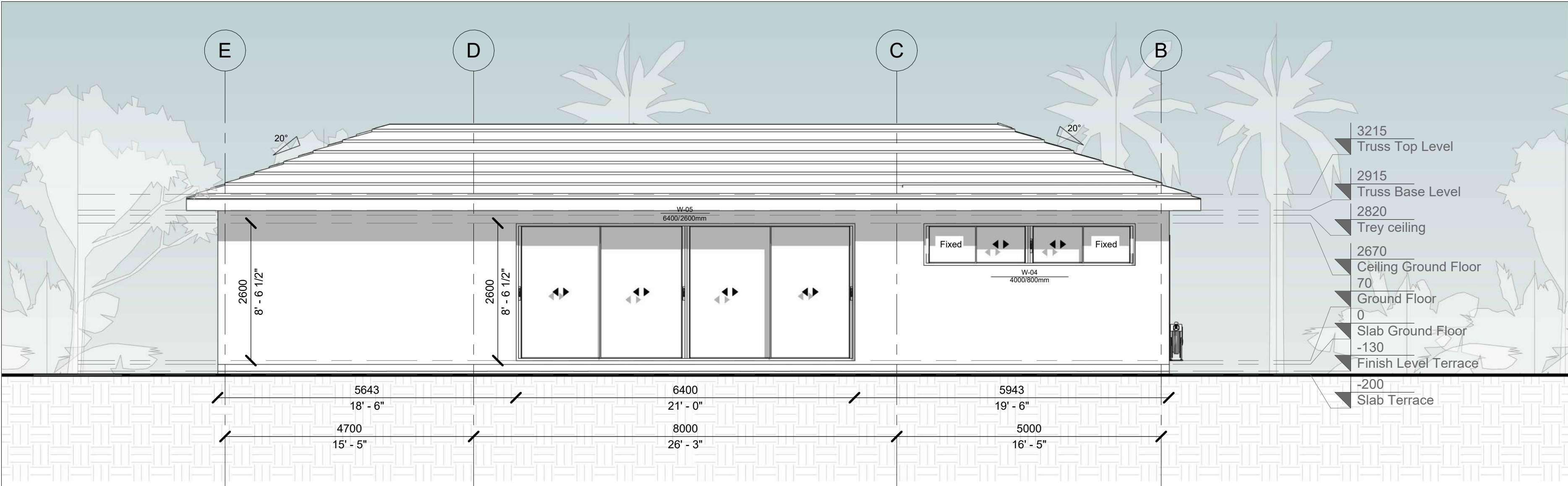
1 Front Elevation 1 : 60
