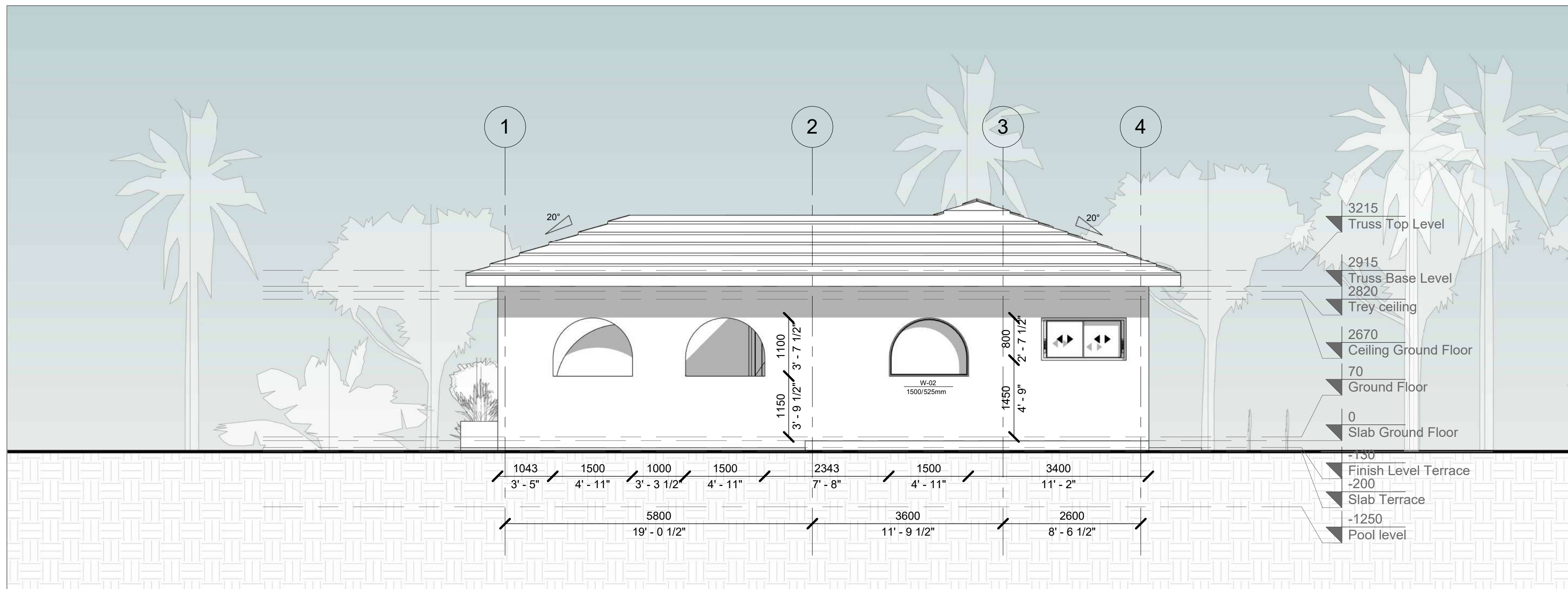
1 Left Elevation 1 : 60
