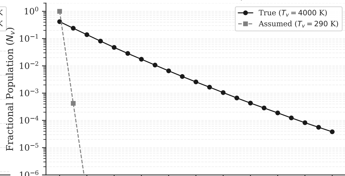
State-Resolved Dist. (Mach 8 | T_0 = 4000 K)
