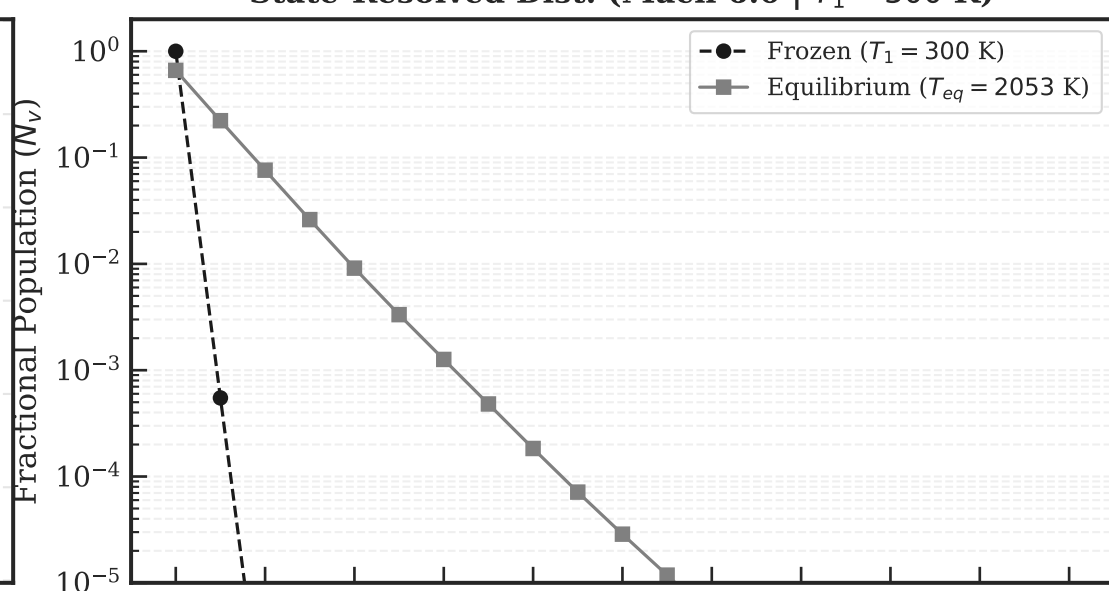
State-Resolved Dist. (Mach 6.0 | T_1 = 300 K)
