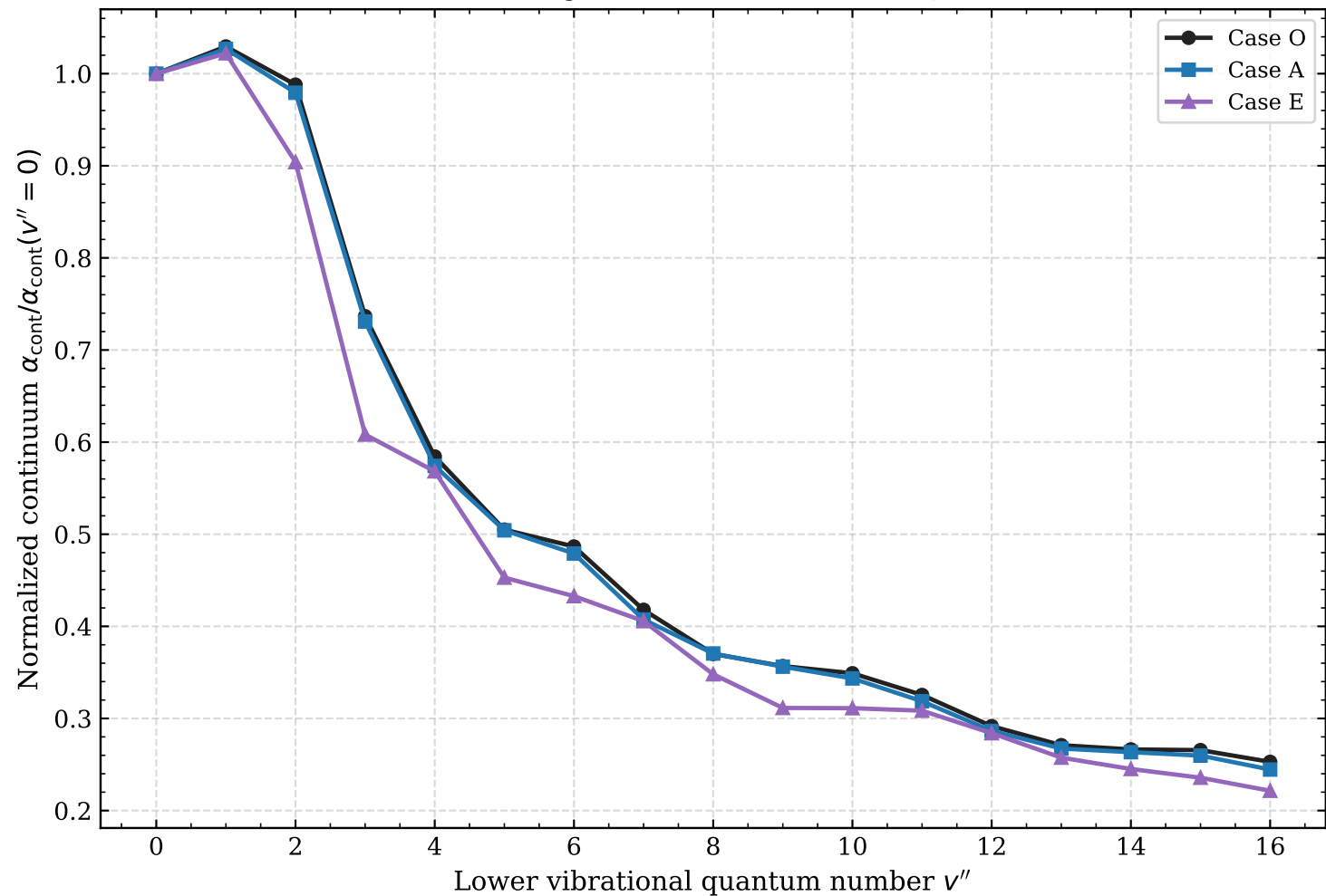
Continuum growth rates at 632.8 nm, J'' = 80
