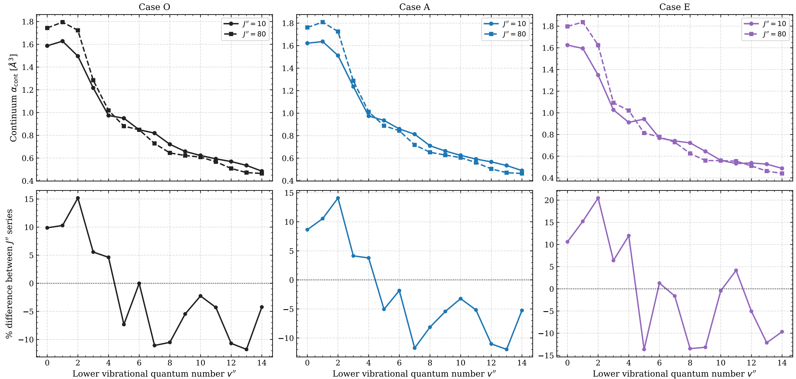
Continuum polarizability at 632.8 nm: Cases O, A, E (absolute; top = two J'' series, bottom = % difference)
